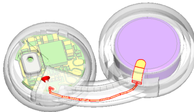
Fig 2.1 Antenna in ear-piece
