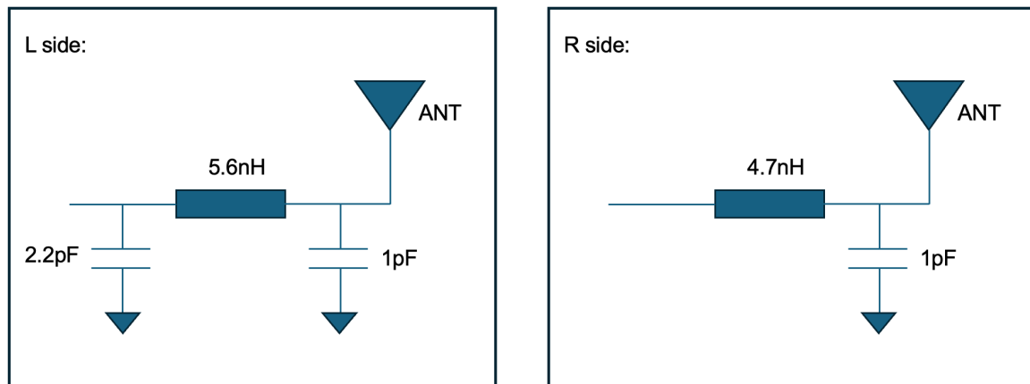
Fig 4.1 recommended matching circuit for antenna
