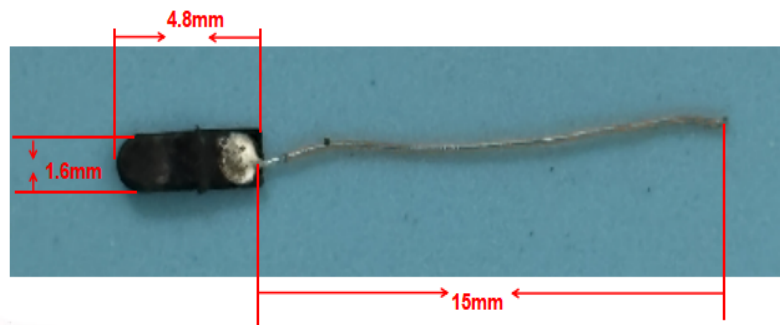
Fig 2.1 Antenna in ear-piece
