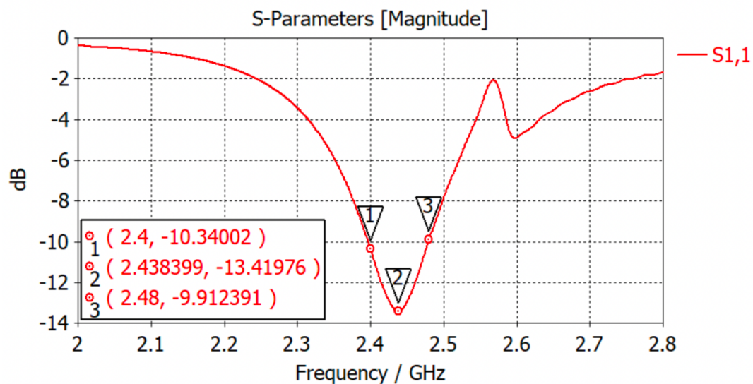
Fig 2.1 S11 of antenna
