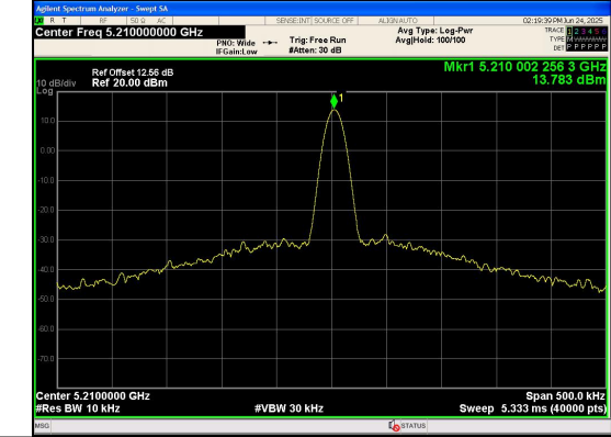
NT/NV_Antenna 0 IEEE 802.11ac_Channel 42_80MHz
