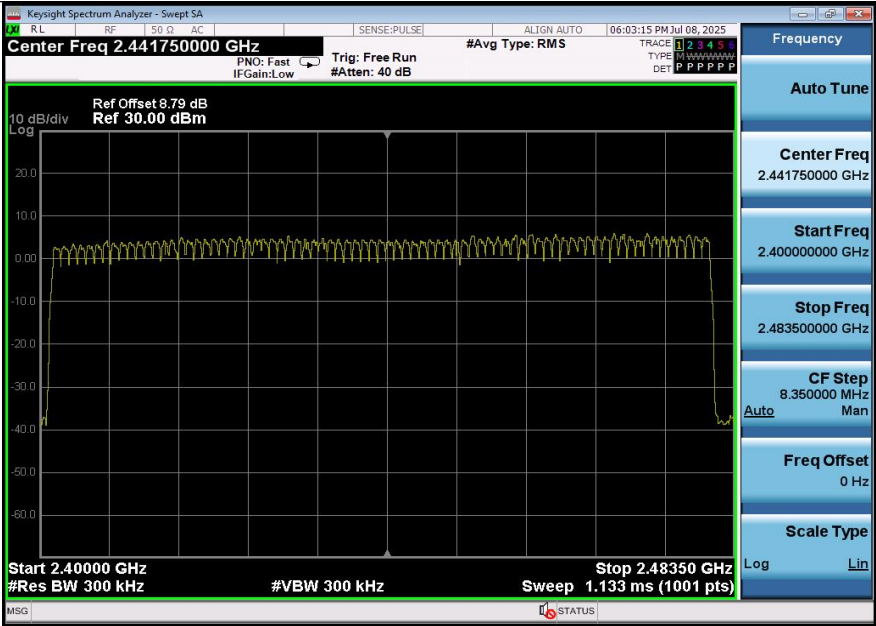
8DPSK Modulation
