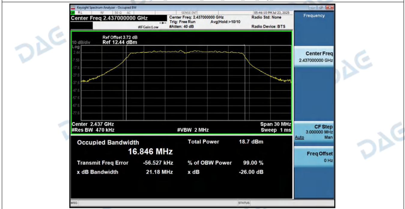
99%_Occupied_Bandwidth_NVNT_ANT1_802_11g_2437
