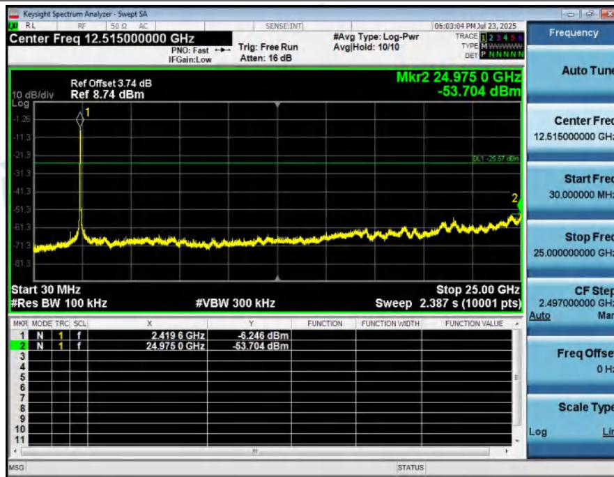
1_Reference_Level_NVNT_ANT1_802_11n(HT40)_2437
