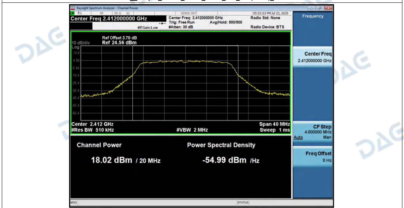
MAX__Output_Power_NVNT_ANT1_802_11n(HT20)_2412
