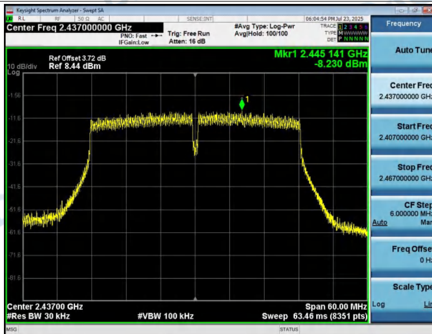
Power_Spectral_Density_NVNT_ANT1_802_11n(HT40)_2437
