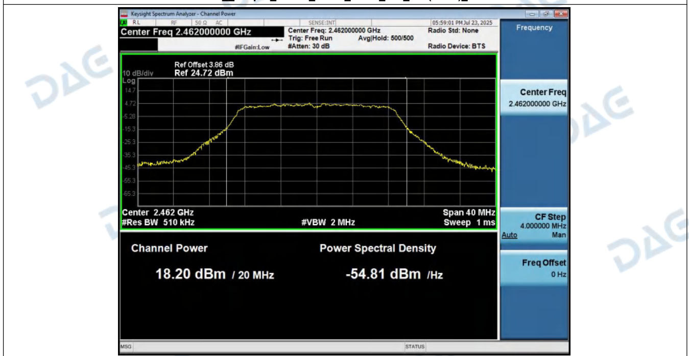
MAX__Output_Power_NVNT_ANT1_802_11n(HT20)_2462
