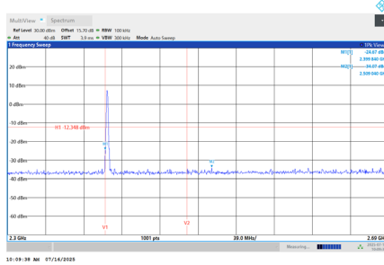
Bandedge-CH37
