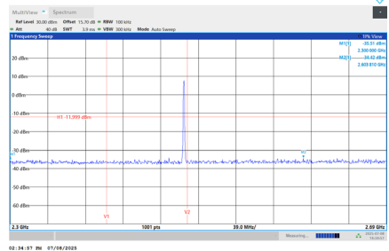
Bandedge-CH39
