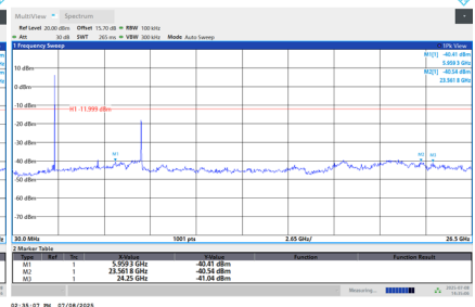
Harmonic-CH39
