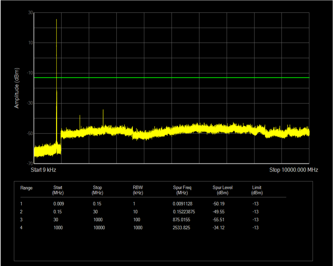
Band5 QPSK BW=5MHz Channel=20625 RB Size=1 Position=#Mid
