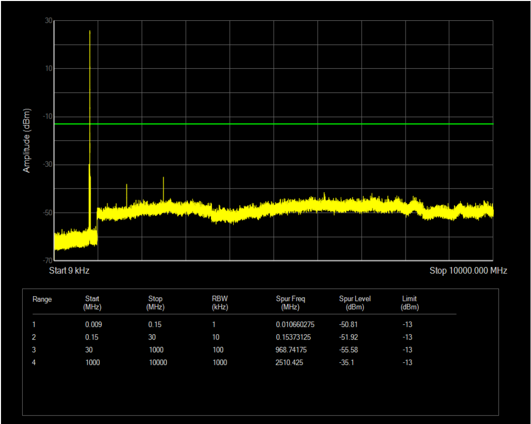
Band5 QPSK BW=3MHz Channel=20525 RB Size=1 Position=#Mid
