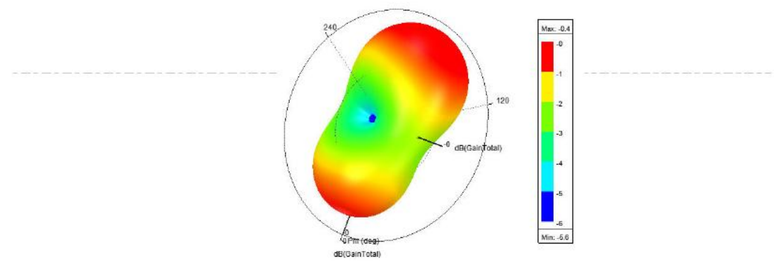
3D Gain Pattern (2450 MHz)
