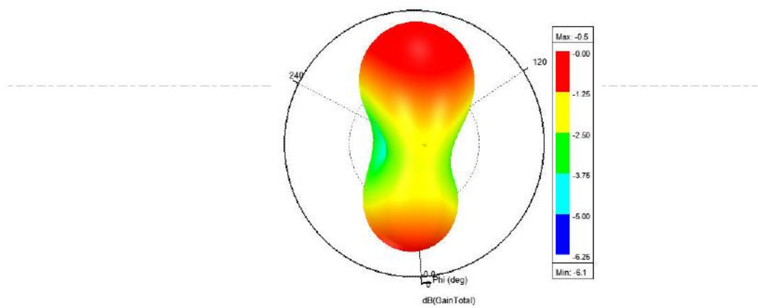
3D Gain Pattern (2500 MHz)
