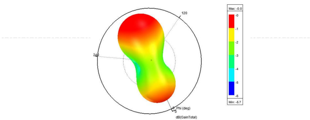
3D Gain Pattern (2500 MHz)
