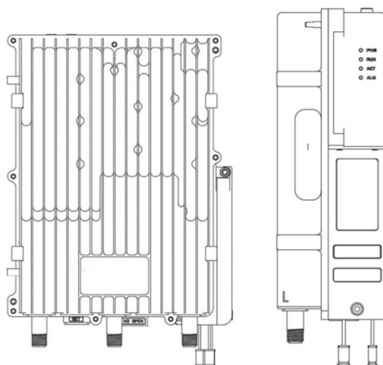
Figure 1-1 Polaris10 Appearance
