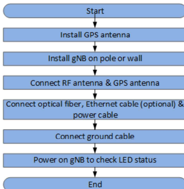
Figure 3-1 Installation Process
