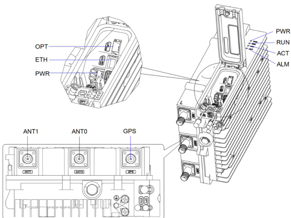
Figure 1-2 Polaris10 Interfaces and Indicators
