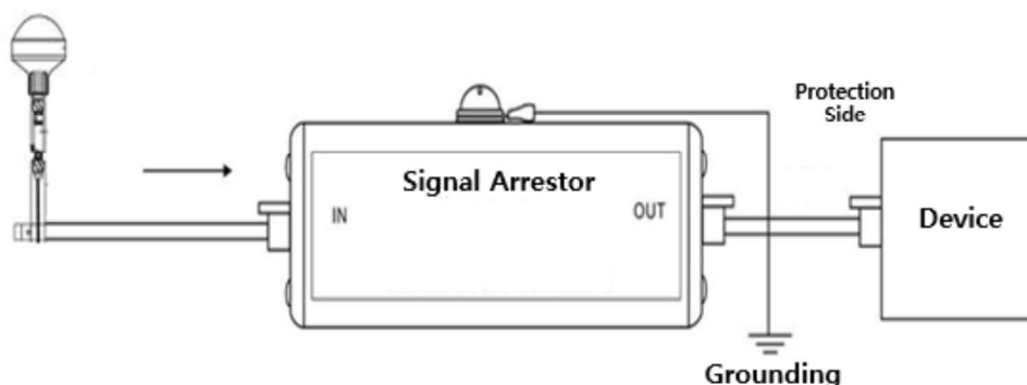
Figure 3-10 GPS Grounding
