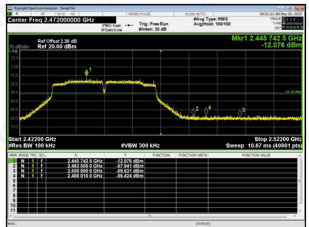
Right bandedge
