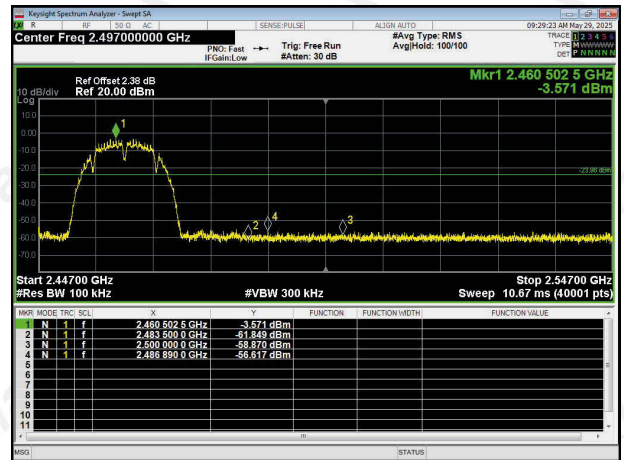
Right bandedge
