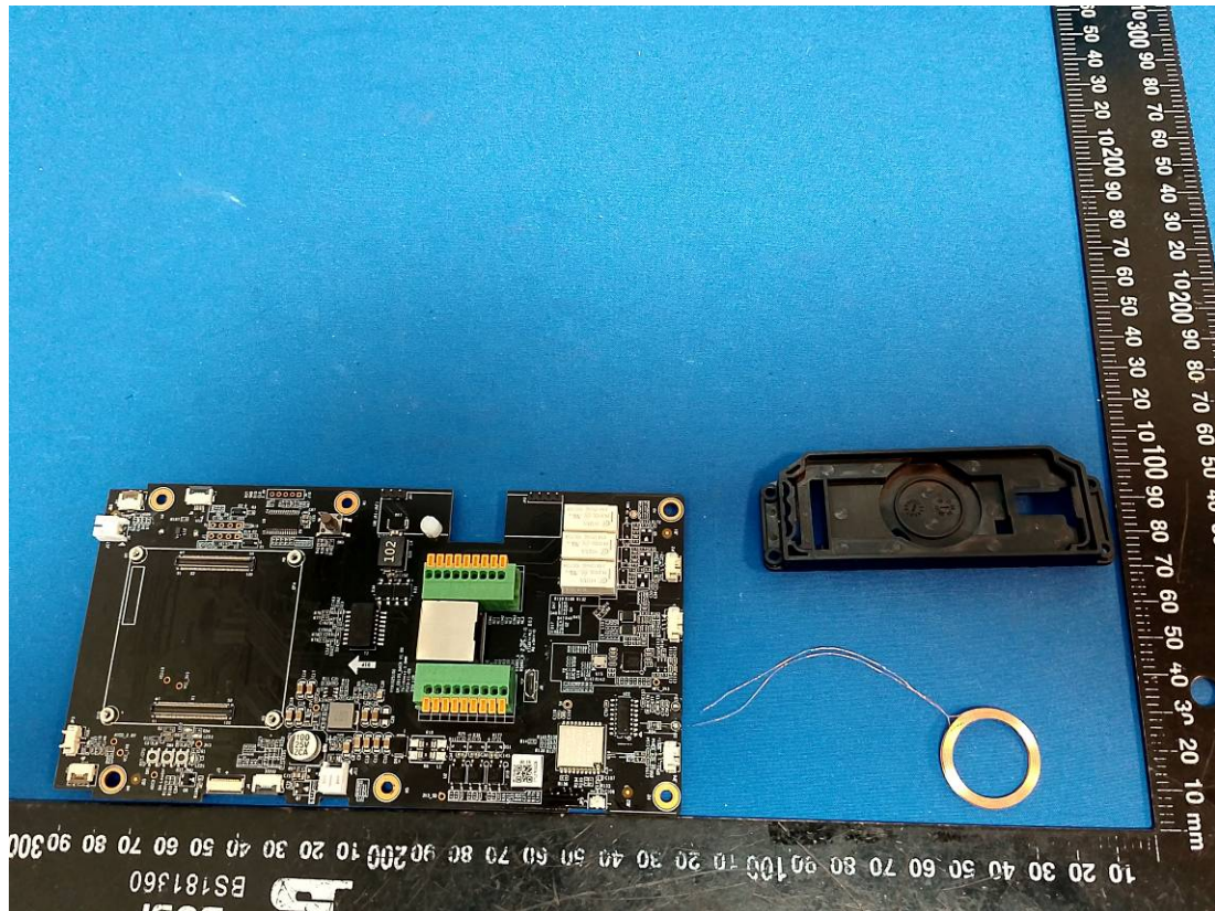
125k Antenna
