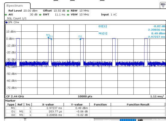
BLE_2M_Middle_Channel
