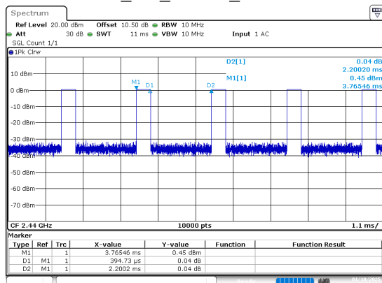
BLE_1M_Middle_Channel
