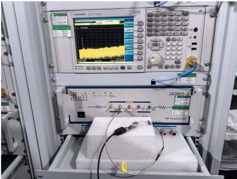
RF Conducted Emission(L)
