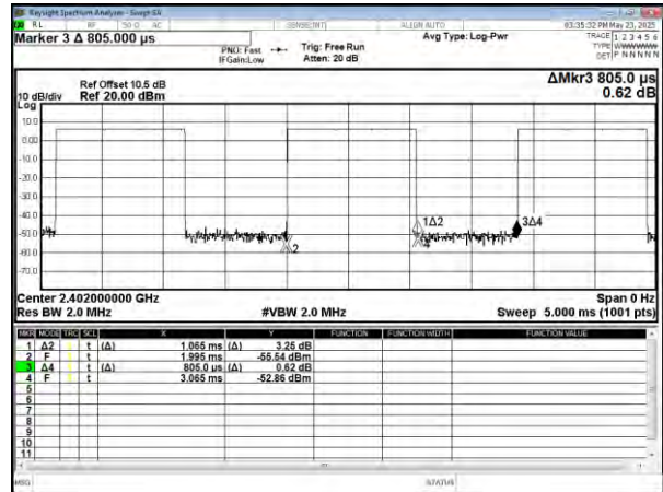
Modulation Type: GFSK 500kbps
