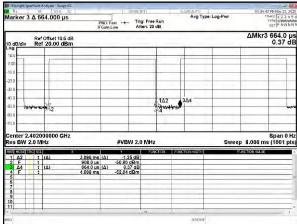
Modulation Type: GFSK 125kbps
