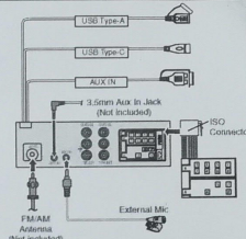
ISO Connector Wiring Chart
