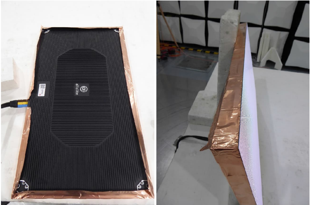
Test setup semi anechoic chamber (copper tape covering of EUT)
