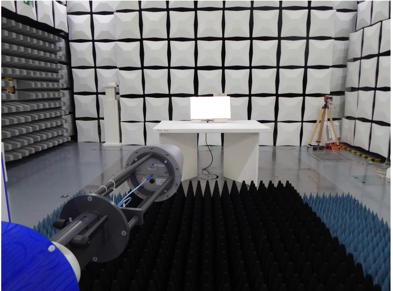
Test setup fully anechoic chamber (1 - 4 GHz)
