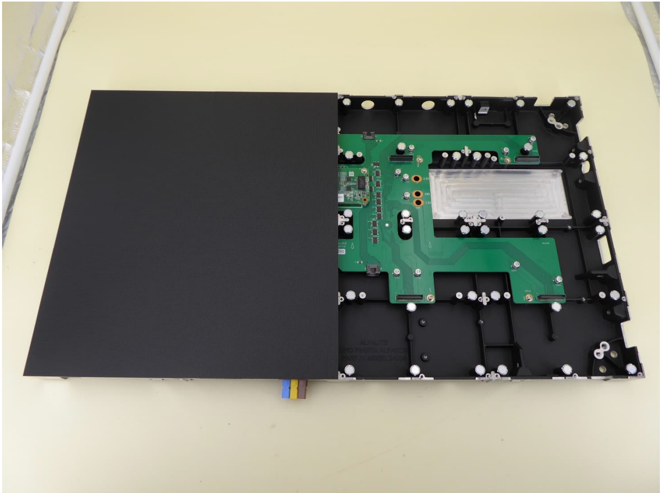
EUT top view with half the panels removed
