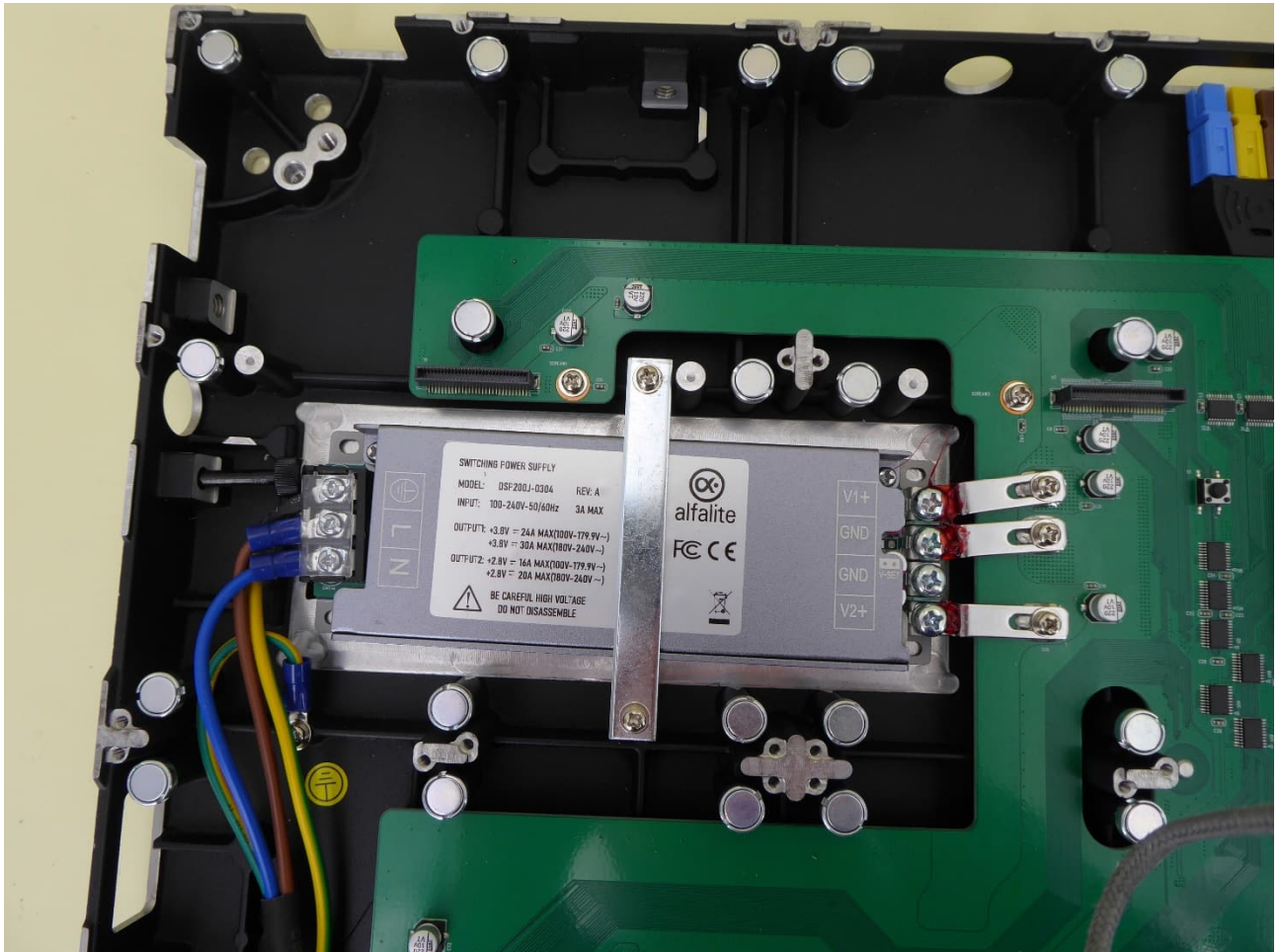
Power supply top view
