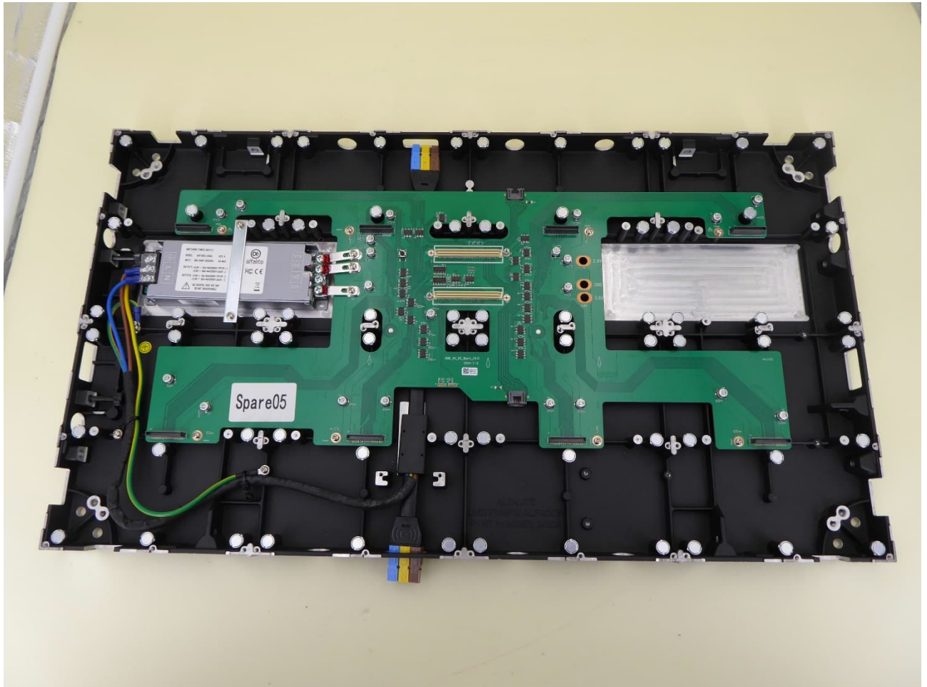
Main PCB top view with Nova Star PCB removed
