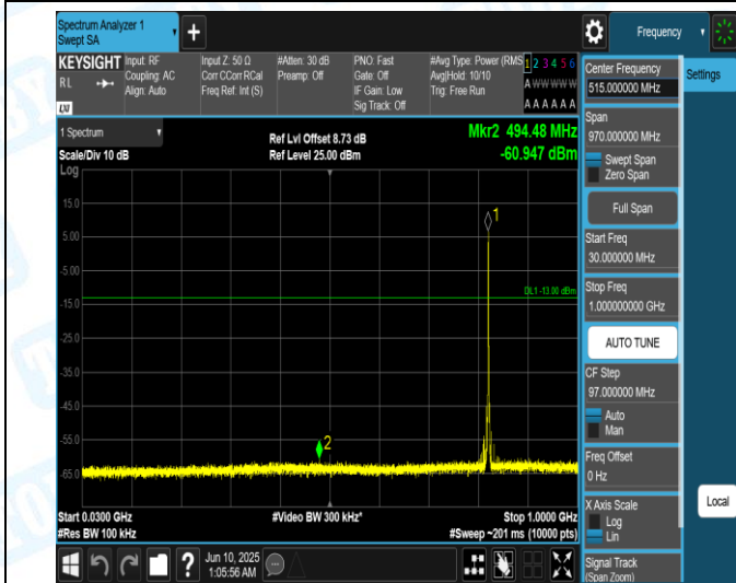
Band 5 - 10 MHz - QPSK - 20450 - PASS
