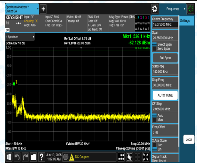
Band 5 - 10 MHz - QPSK - 20525 - PASS
