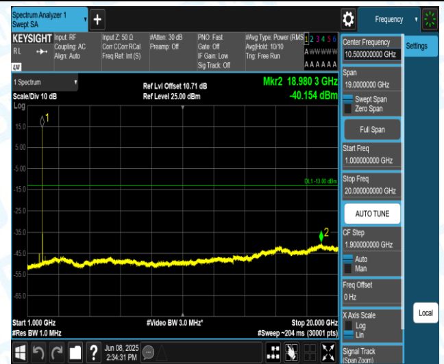
Band 2 - 10 MHz - 16 QAM - 19150 - PASS
