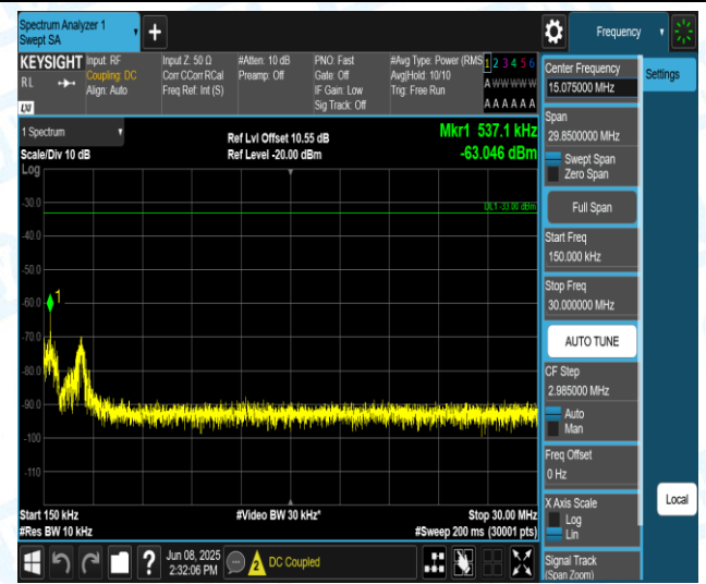
Band 2 - 10 MHz - QPSK - 18900 - PASS
