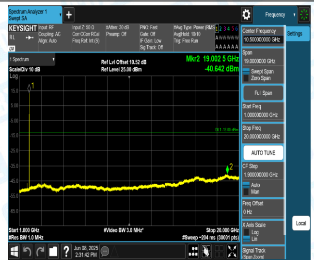
Band 2 - 10 MHz - 16 QAM - 18650 - PASS
