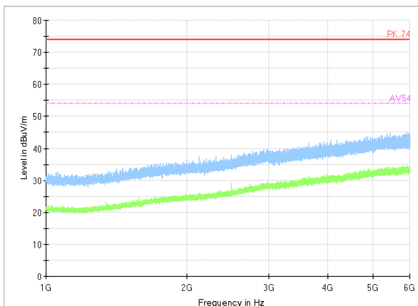
Pic3. Radiated emission (1GHz –6GHz)
