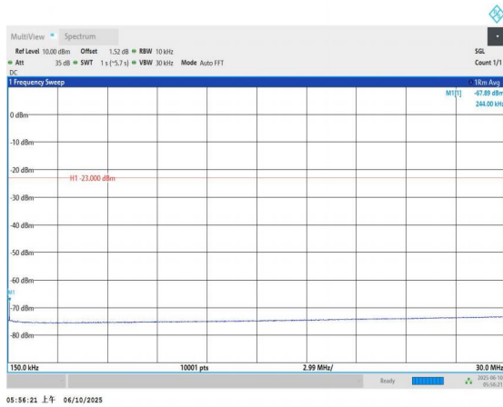
Band5-4182-0.15~30MHz-PASS
