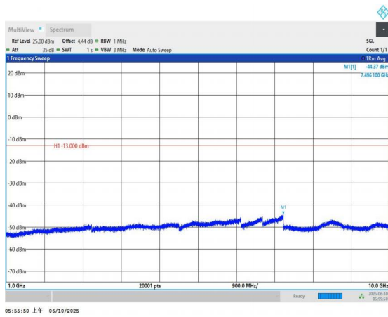
Band5-4132-1000~10000MHz-PASS
