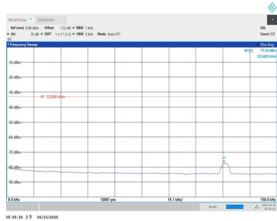
Band5-4132-0.009~0.15MHz-PASS
