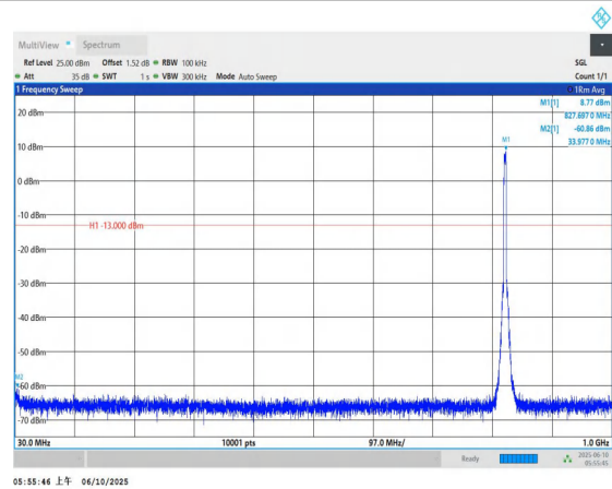
Band5-4132-30~1000MHz-PASS
