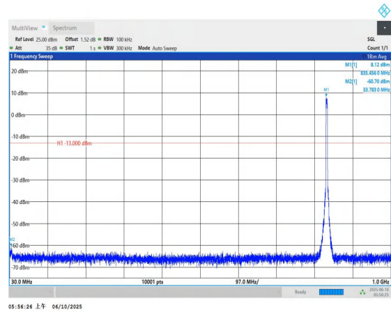
Band5-4182-30~1000MHz-PASS
