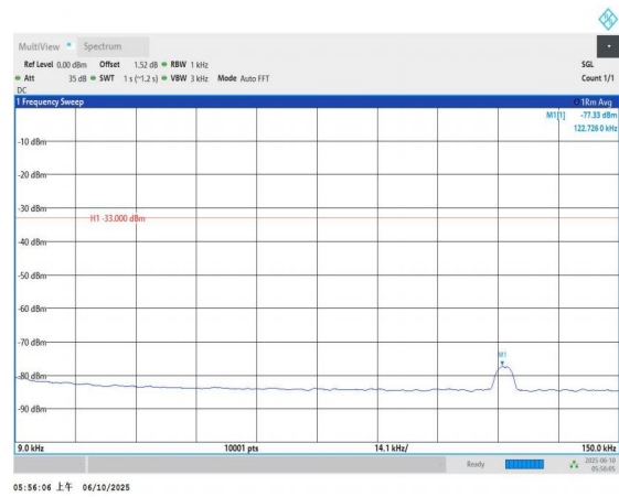
Band5-4182-0.009~0.15MHz-PASS
