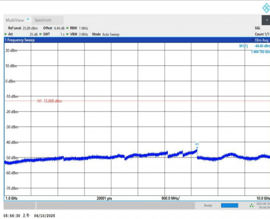
Band5-4182-1000~10000MHz-PASS
