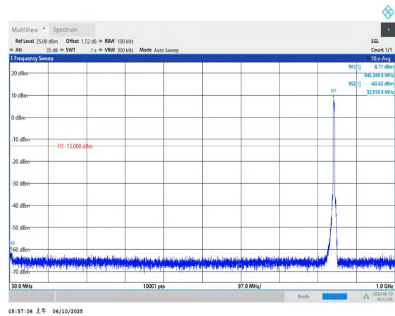
Band5-4233-30~1000MHz-PASS
