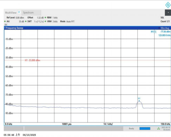
Band5-4233-0.009~0.15MHz-PASS
