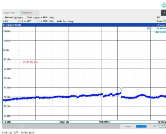
Band5-4233-1000~10000MHz-PASS
