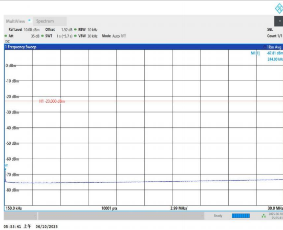
Band5-4132-0.15~30MHz-PASS
