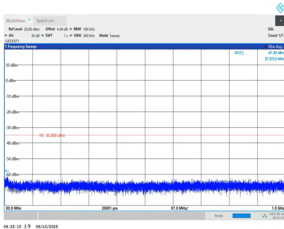
Band41-5MHz-QPSK-41565-1RB#0-30~1000-PASS
