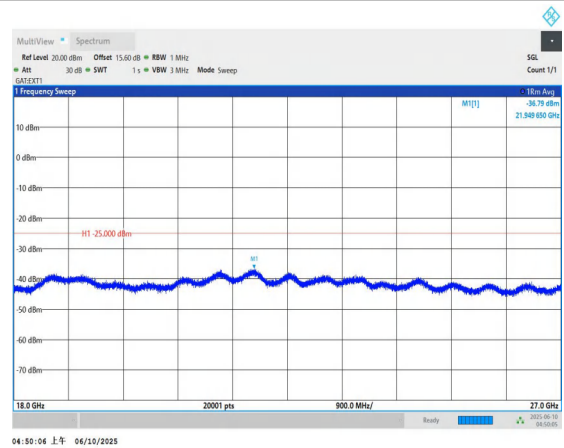
Band41-10MHz-QPSK-41540-1RB#0-18000~27000-PASS
