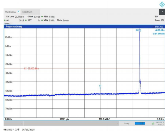
Band41-5MHz-QPSK-41565-1RB#0-1000~3000-PASS
