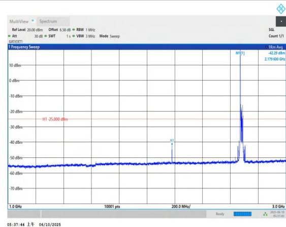
Band41-20MHz-QPSK-41490-1RB#0-1000~3000-PASS
