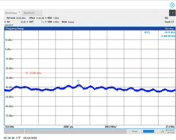
Band41-15MHz-QPSK-41515-1RB#0-18000~27000-PASS
