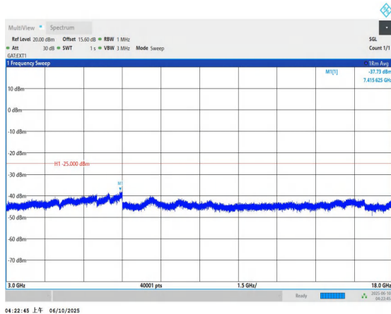
Band41-5MHz-QPSK-39675-1RB#0-3000~18000-PASS
