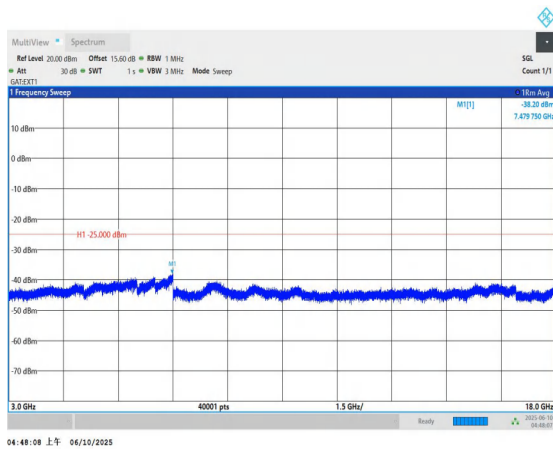
Band41-10MHz-QPSK-40620-1RB#0-3000~18000-PASS
