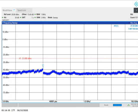
Band41-15MHz-QPSK-41515-1RB#0-3000~18000-PASS
