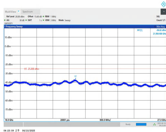
Band41-5MHz-QPSK-39675-1RB#0-18000~27000-PASS
