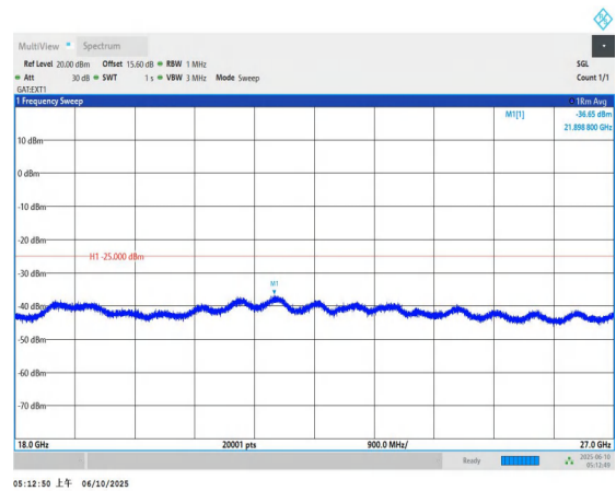
Band41-15MHz-QPSK-40620-1RB#0-18000~27000-PASS
