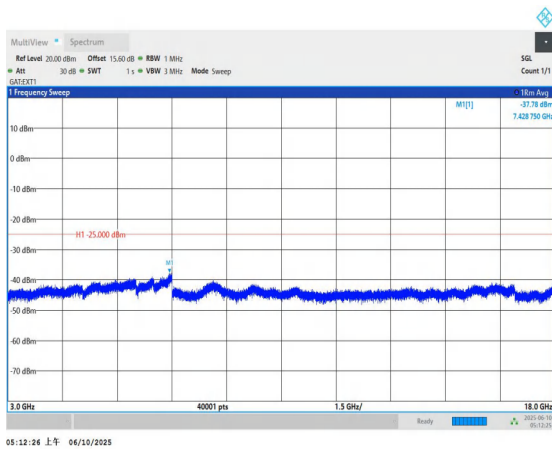
Band41-15MHz-QPSK-40620-1RB#0-3000~18000-PASS
