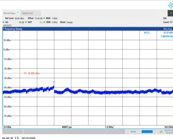
Band41-10MHz-QPSK-39700-1RB#0-3000~18000-PASS
