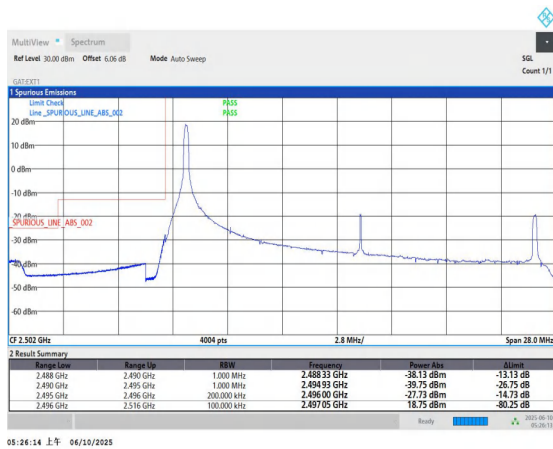
Band41-20MHz-QPSK-39750-1RB#0-PASS
