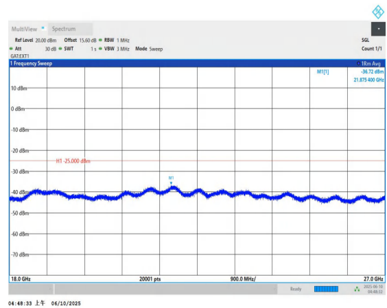
Band41-10MHz-QPSK-40620-1RB#0-18000~27000-PASS
