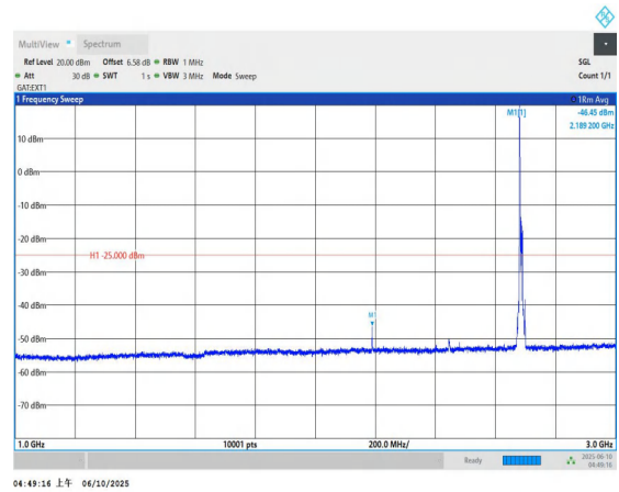
Band41-10MHz-QPSK-41540-1RB#0-1000~3000-PASS
