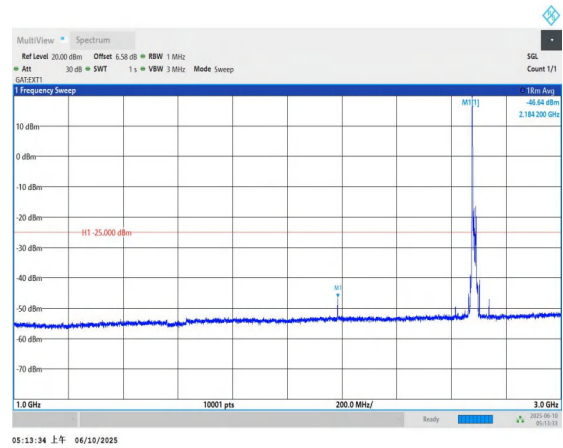
Band41-15MHz-QPSK-41515-1RB#0-1000~3000-PASS
