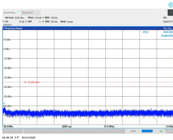
Band41-10MHz-QPSK-41540-1RB#0-30~1000-PASS
