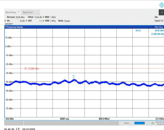
Band41-10MHz-QPSK-39700-1RB#0-18000~27000-PASS
