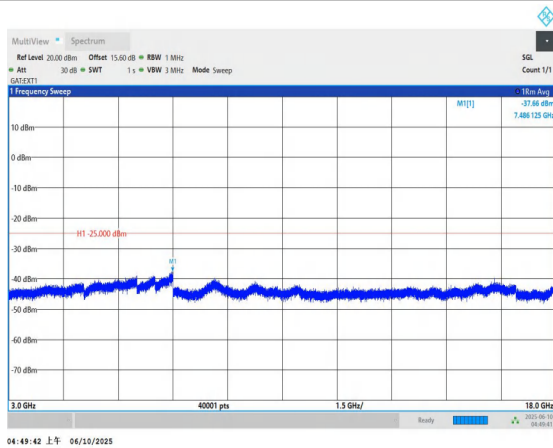
Band41-10MHz-QPSK-41540-1RB#0-3000~18000-PASS
