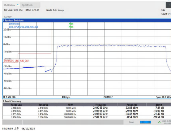
Band41-20MHz-QPSK-39750-100RB#0-PASS
