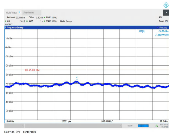
Band41-20MHz-QPSK-40620-1RB#0-18000~27000-PASS
