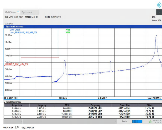
Band41-15MHz-QPSK-39725-1RB#74-PASS
