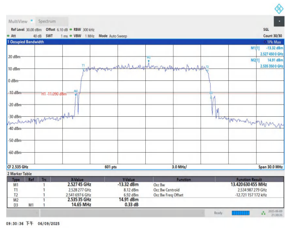
Band7-15MHz-QPSK-21100-75RB#0-PASS
