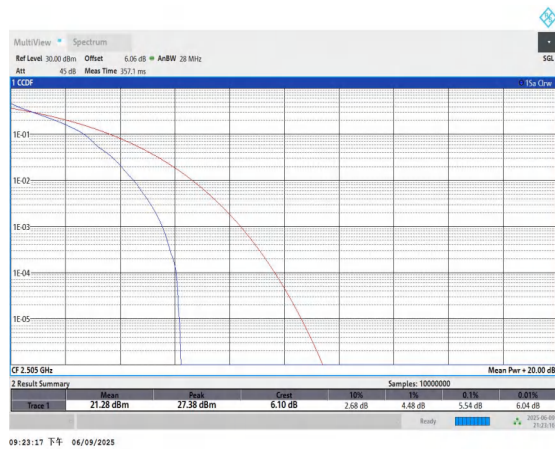
Band7-10MHz-QPSK-20800-1RB#0-PASS
