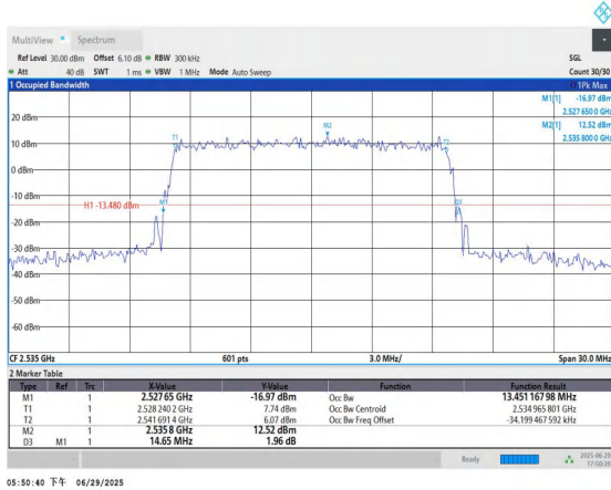
Band7-15MHz-16QAM-21100-75RB#0-PASS
