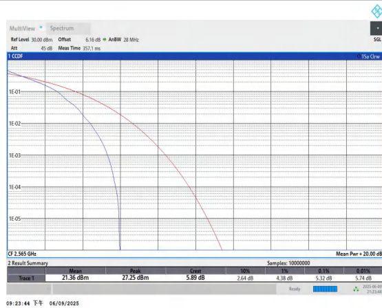
Band7-10MHz-QPSK-21400-1RB#0-PASS
