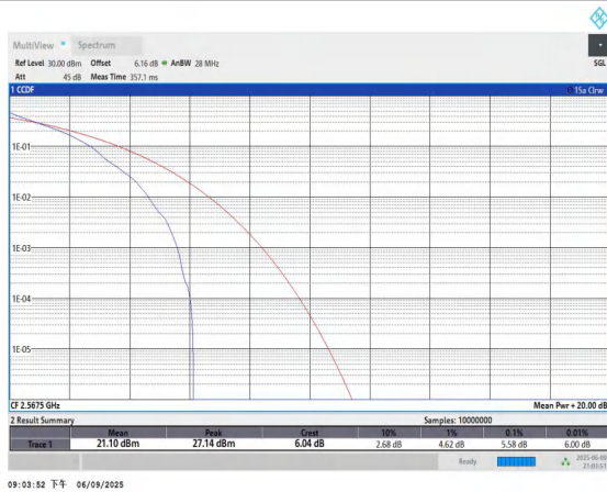
Band7-5MHz-QPSK-21425-1RB#0-PASS
