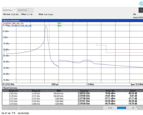
Band7-5MHz-QPSK-21425-1RB#24-PASS
