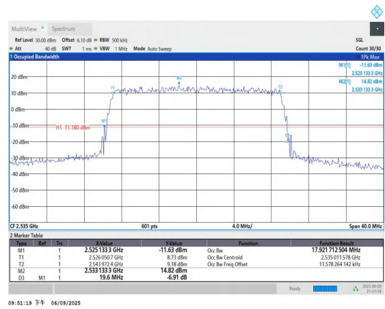
Band7-20MHz-QPSK-21100-100RB#0-PASS
