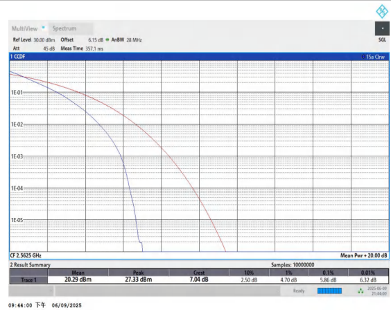
Band7-15MHz-QPSK-21375-75RB#0-PASS
