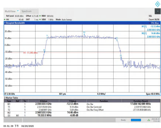
Band7-20MHz-16QAM-21350-100RB#0-PASS
