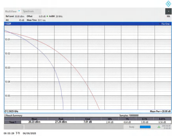
Band7-5MHz-QPSK-20775-25RB#0-PASS
