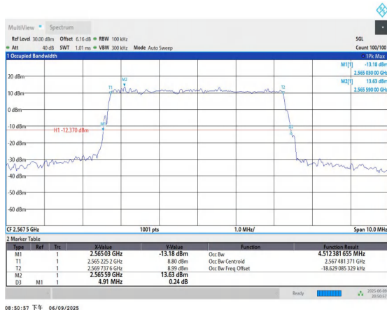
Band7-5MHz-QPSK-21425-25RB#0-PASS
