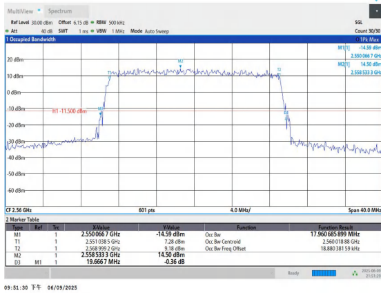
Band7-20MHz-QPSK-21350-100RB#0-PASS
