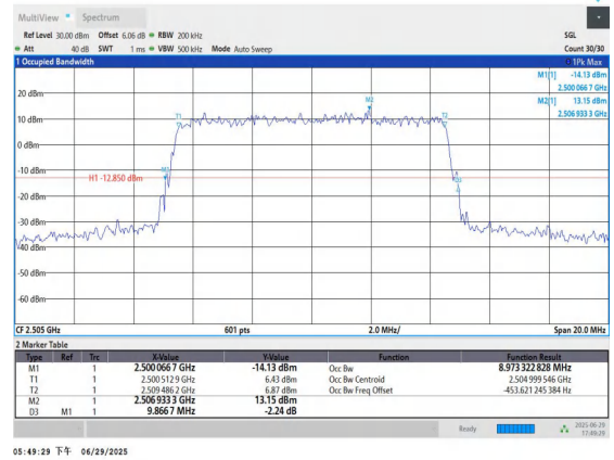
Band7-10MHz-16QAM-20800-50RB#0-PASS
