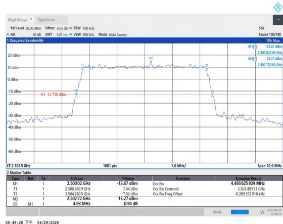
Band7-5MHz-16QAM-20775-25RB#0-PASS
