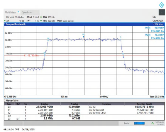
Band7-10MHz-QPSK-21100-50RB#0-PASS
