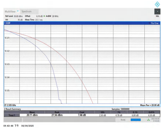
Band7-15MHz-QPSK-21100-75RB#0-PASS
