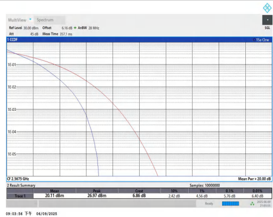
Band7-5MHz-QPSK-21425-25RB#0-PASS
