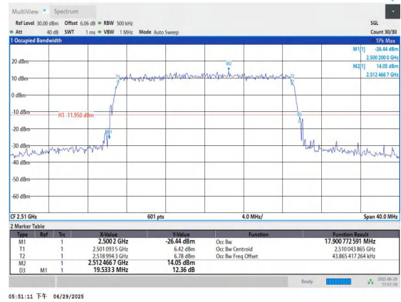
Band7-20MHz-16QAM-20850-100RB#0-PASS
