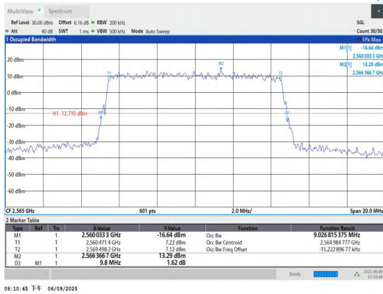
Band7-10MHz-QPSK-21400-50RB#0-PASS
