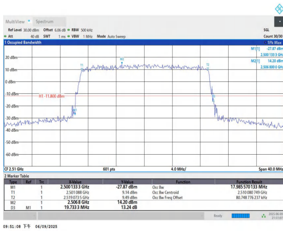
Band7-20MHz-QPSK-20850-100RB#0-PASS
