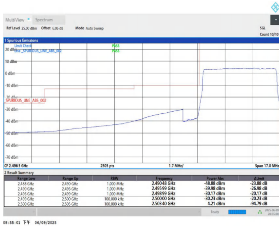
Band7-5MHz-QPSK-20775-25RB#0-PASS
