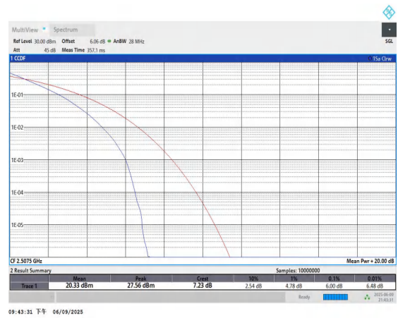
Band7-15MHz-QPSK-20825-75RB#0-PASS
