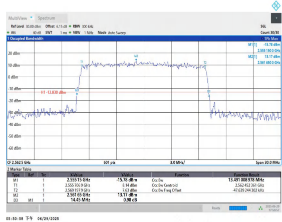
Band7-15MHz-16QAM-21375-75RB#0-PASS
