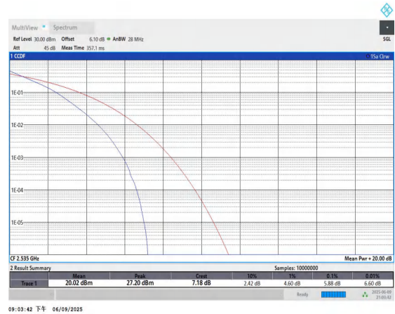
Band7-5MHz-QPSK-21100-25RB#0-PASS
