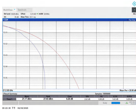
Band7-10MHz-QPSK-21100-1RB#0-PASS
