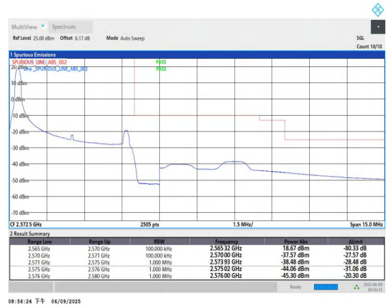
Band7-5MHz-QPSK-21425-1RB#0-PASS
