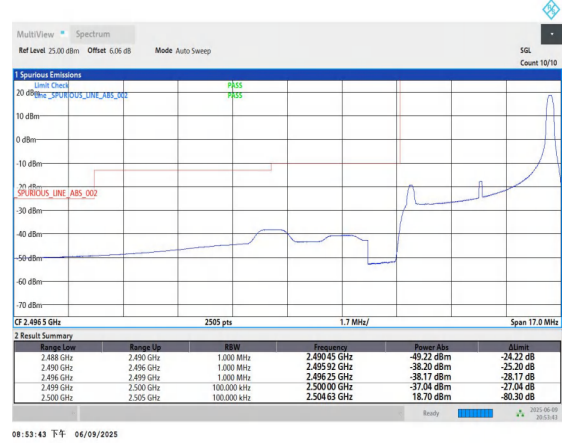
Band7-5MHz-QPSK-20775-1RB#24-PASS
