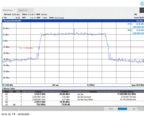
Band7-20MHz-16QAM-21100-100RB#0-PASS
