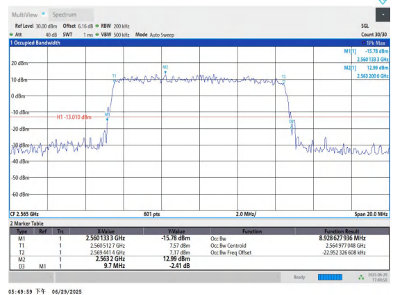
Band7-10MHz-16QAM-21400-50RB#0-PASS
