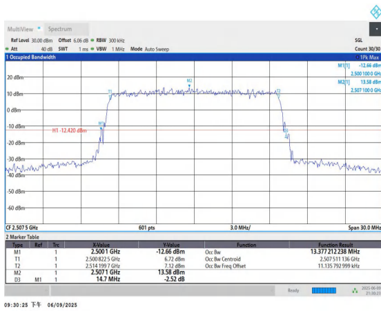
Band7-15MHz-QPSK-20825-75RB#0-PASS
