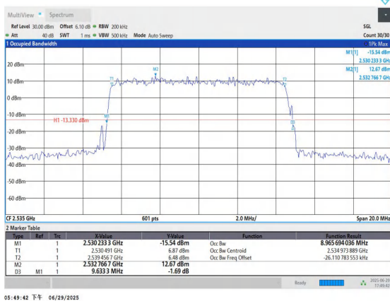
Band7-10MHz-16QAM-21100-50RB#0-PASS
