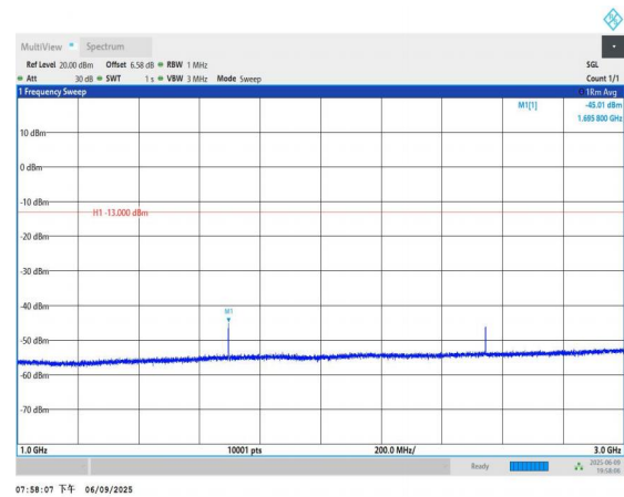
Band5-1.4MHz-QPSK-20643-1RB#0-1000~3000-PASS
