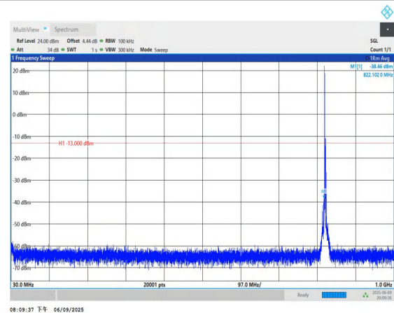
Band5-3MHz-QPSK-20415-1RB#0-30~1000-PASS
