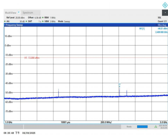
Band5-10MHz-QPSK-20525-1RB#0-1000~3000-PASS
