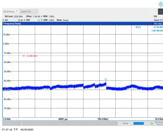
Band5-1.4MHz-QPSK-20407-1RB#0-3000~10000-PASS
