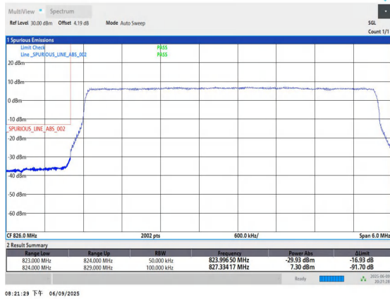
Band5-5MHz-QPSK-20425-25RB#0-PASS
