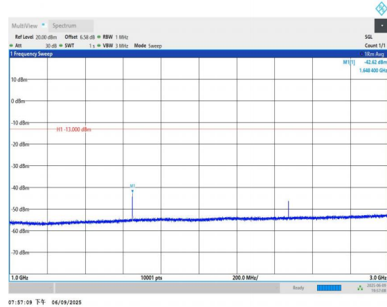
Band5-1.4MHz-QPSK-20407-1RB#0-1000~3000-PASS
