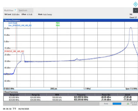
Band5-10MHz-QPSK-20450-1RB#49-PASS
