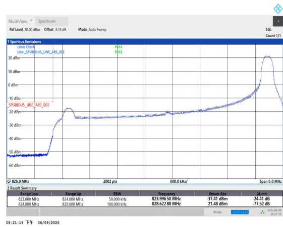
Band5-5MHz-QPSK-20425-1RB#24-PASS
