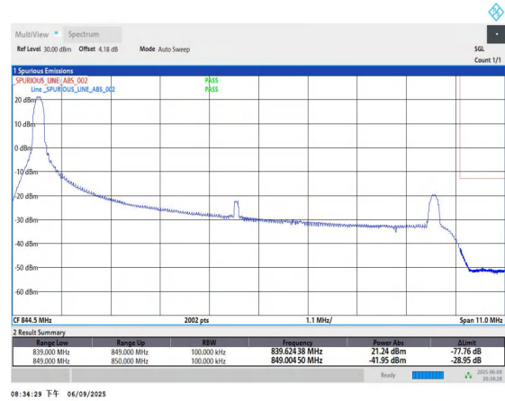
Band5-10MHz-QPSK-20600-1RB#0-PASS
