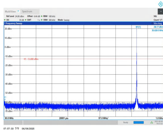
Band5-1.4MHz-QPSK-20525-1RB#0-30~1000-PASS
