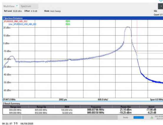
Band5-5MHz-QPSK-20625-1RB#24-PASS
