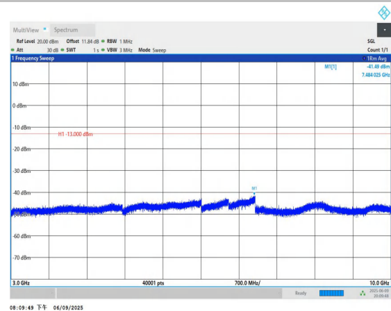
Band5-3MHz-QPSK-20415-1RB#0-3000~10000-PASS
