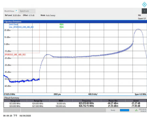
Band5-3MHz-QPSK-20415-1RB#14-PASS
