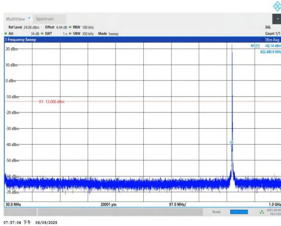
Band5-1.4MHz-QPSK-20407-1RB#0-30~1000-PASS
