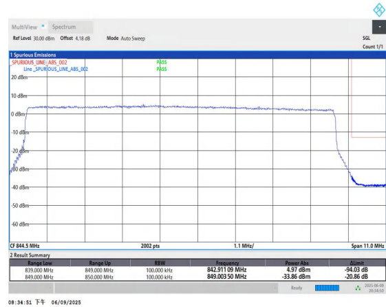
Band5-10MHz-QPSK-20600-50RB#0-PASS
