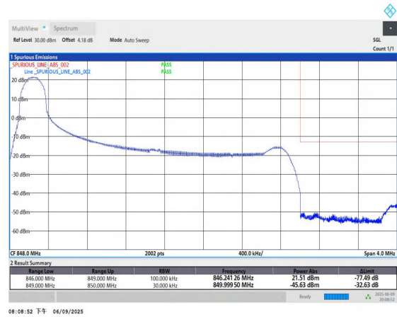
Band5-3MHz-QPSK-20635-1RB#0-PASS
