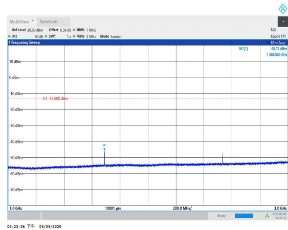
Band5-5MHz-QPSK-20625-1RB#0-1000~3000-PASS
