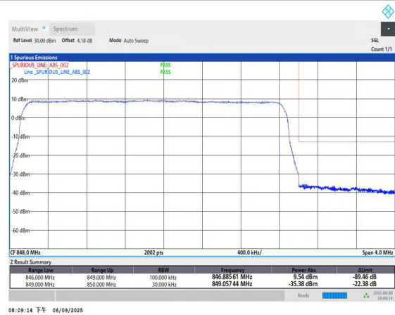
Band5-3MHz-QPSK-20635-15RB#0-PASS
