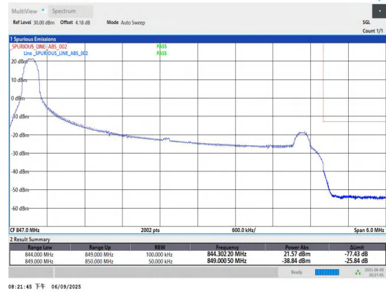
Band5-5MHz-QPSK-20625-1RB#0-PASS
