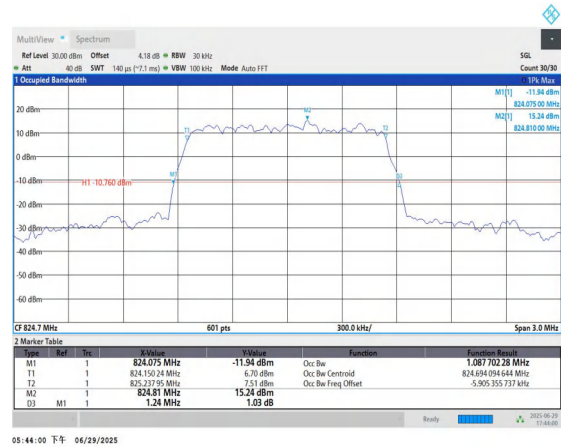
Band5-1.4MHz-16QAM-20407-6RB#0-PASS
