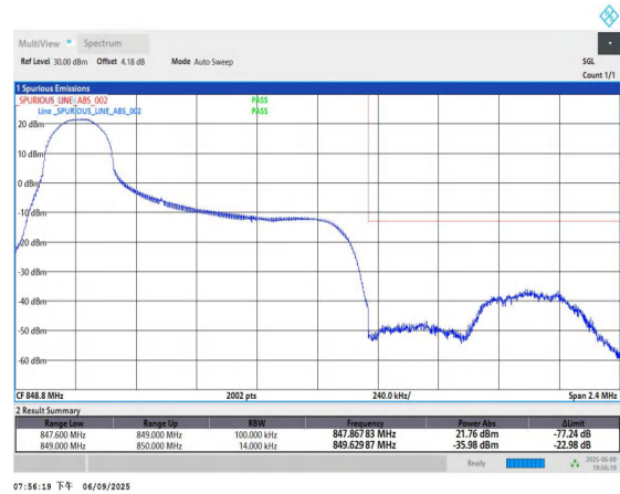
Band5-1.4MHz-QPSK-20643-1RB#0-PASS
