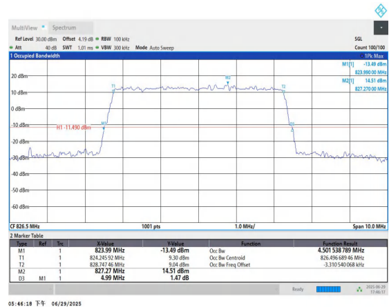
Band5-5MHz-16QAM-20425-25RB#0-PASS
