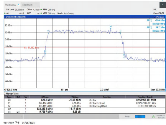
Band5-10MHz-16QAM-20450-50RB#0-PASS
