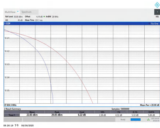
Band5-5MHz-QPSK-20425-25RB#0-PASS
