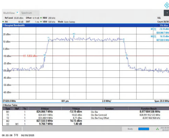
Band5-10MHz-QPSK-20450-50RB#0-PASS
