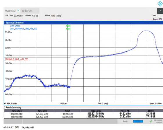
Band5-1.4MHz-QPSK-20407-1RB#5-PASS
