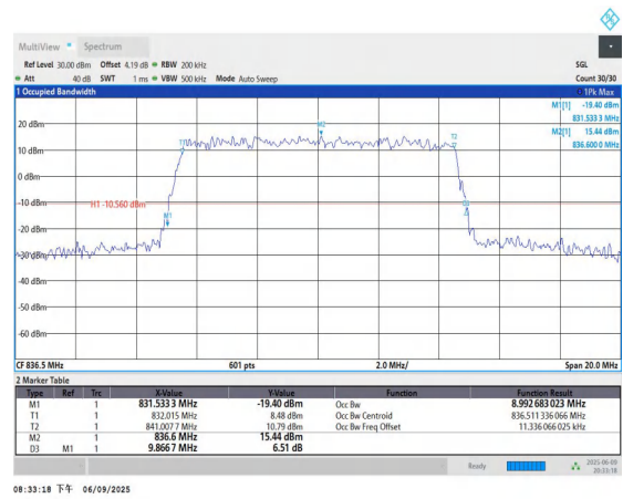
Band5-10MHz-QPSK-20525-50RB#0-PASS
