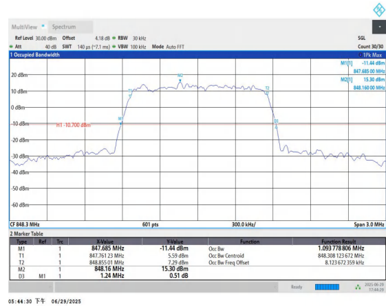
Band5-1.4MHz-16QAM-20643-6RB#0-PASS
