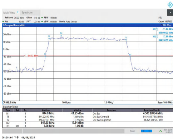
Band5-5MHz-QPSK-20625-25RB#0-PASS
