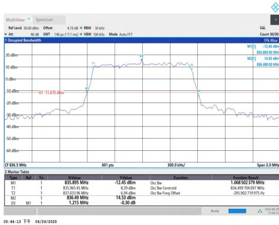
Band5-1.4MHz-16QAM-20525-6RB#0-PASS
