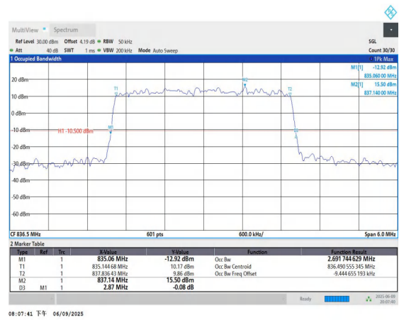
Band5-3MHz-QPSK-20525-15RB#0-PASS
