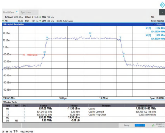
Band5-5MHz-16QAM-20525-25RB#0-PASS
