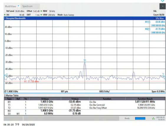
Band2-3MHz-16QAM-19185-15RB#0-PASS
