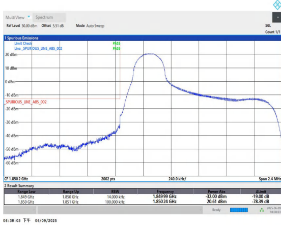
Band2-1.4MHz-QPSK-18607-1RB#0-PASS
