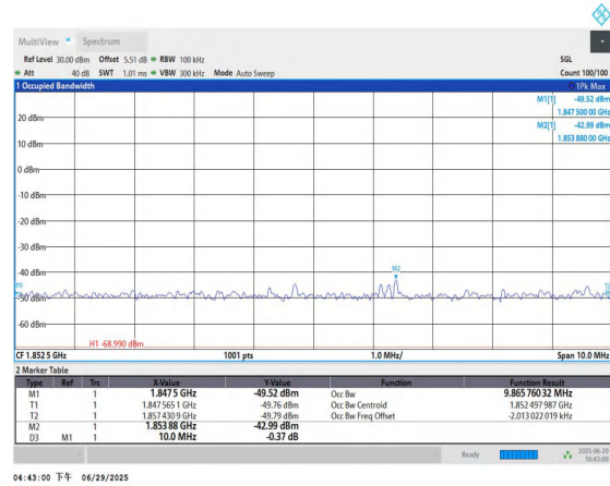
Band2-5MHz-16QAM-18625-25RB#0-PASS
