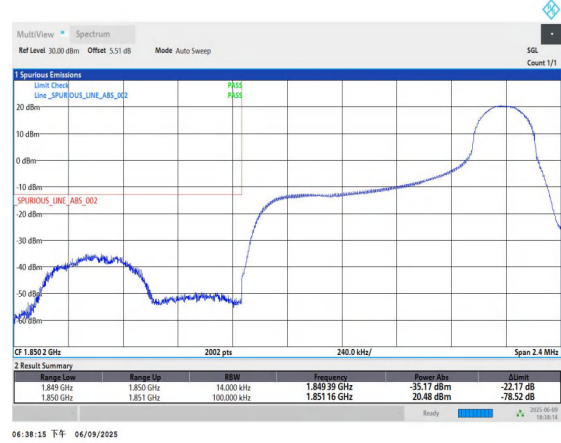
Band2-1.4MHz-QPSK-18607-1RB#5-PASS
