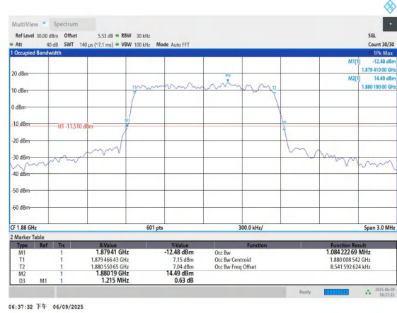
Band2-1.4MHz-QPSK-18900-6RB#0-PASS
