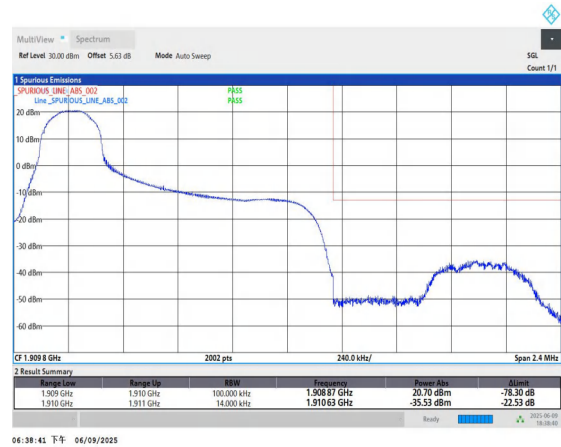
Band2-1.4MHz-QPSK-19193-1RB#0-PASS
