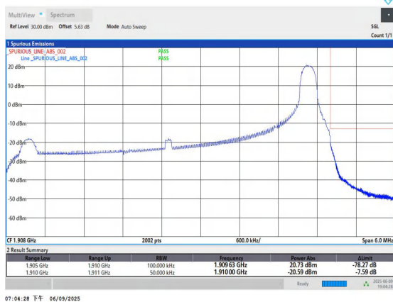
Band2-5MHz-QPSK-19175-1RB#24-PASS
