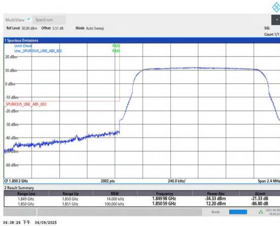
Band2-1.4MHz-QPSK-18607-6RB#0-PASS
