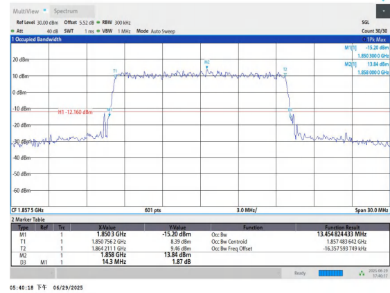
Band2-15MHz-16QAM-18675-75RB#0-PASS
