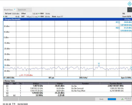
Band2-1.4MHz-16QAM-19193-6RB#0-PASS
