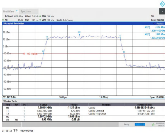
Band2-5MHz-QPSK-19175-25RB#0-PASS
