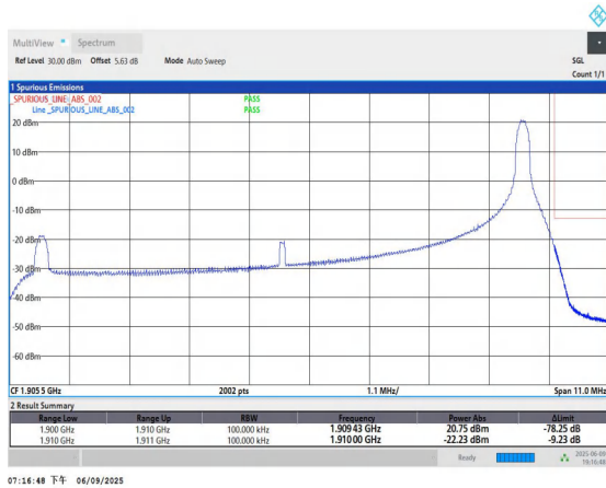
Band2-10MHz-QPSK-19150-1RB#49-PASS
