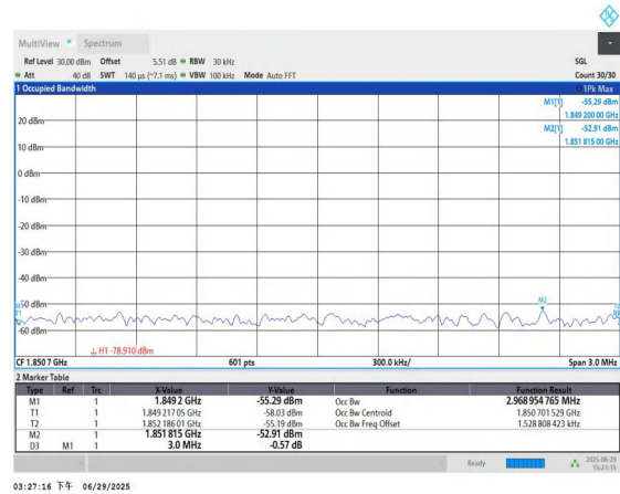
Band2-1.4MHz-16QAM-18607-6RB#0-PASS
