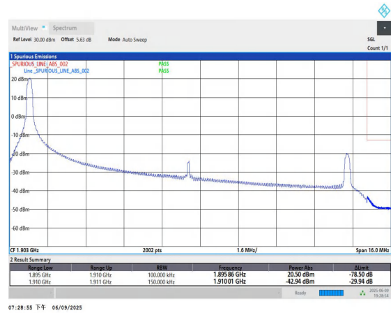
Band2-15MHz-QPSK-19125-1RB#0-PASS
