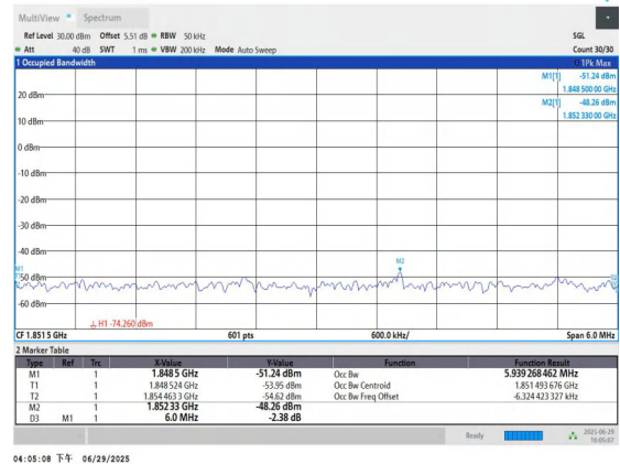
Band2-3MHz-16QAM-18615-15RB#0-PASS
