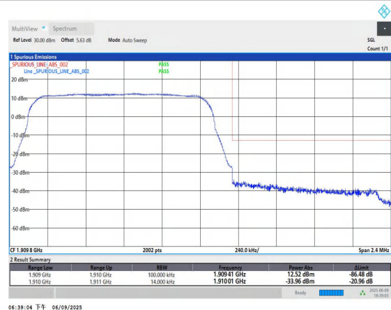
Band2-1.4MHz-QPSK-19193-6RB#0-PASS
