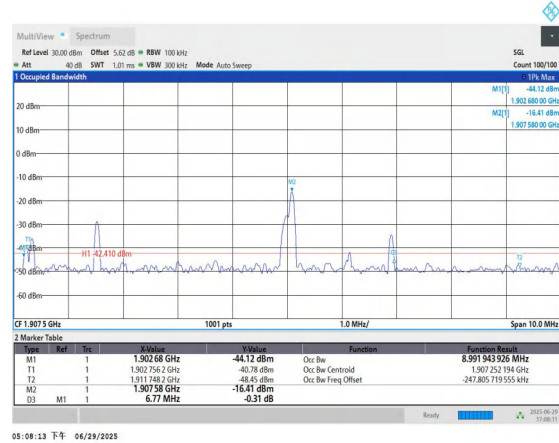
Band2-5MHz-16QAM-19175-25RB#0-PASS
