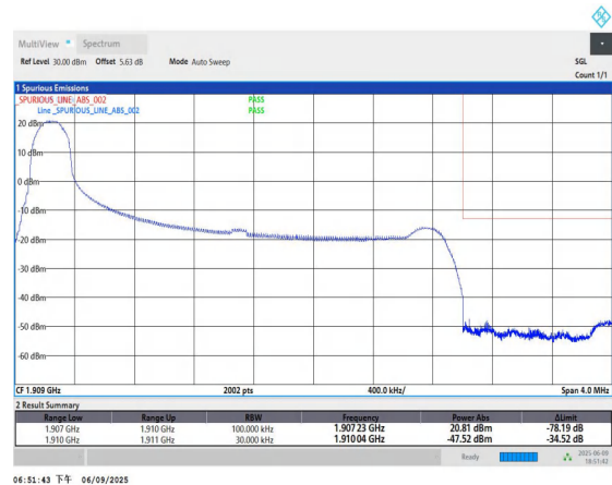
Band2-3MHz-QPSK-19185-1RB#0-PASS
