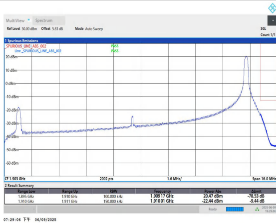
Band2-15MHz-QPSK-19125-1RB#74-PASS
