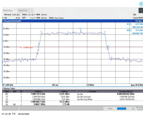
Band2-10MHz-QPSK-19150-50RB#0-PASS
