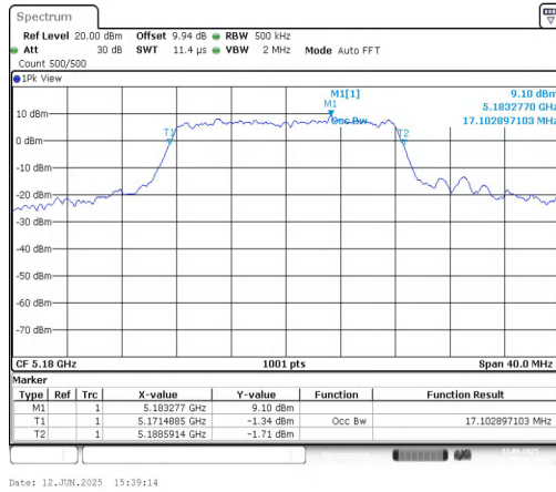
11A-Ant1-5180
