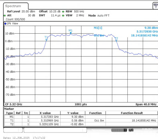
11N20SISO-Ant1-5320
