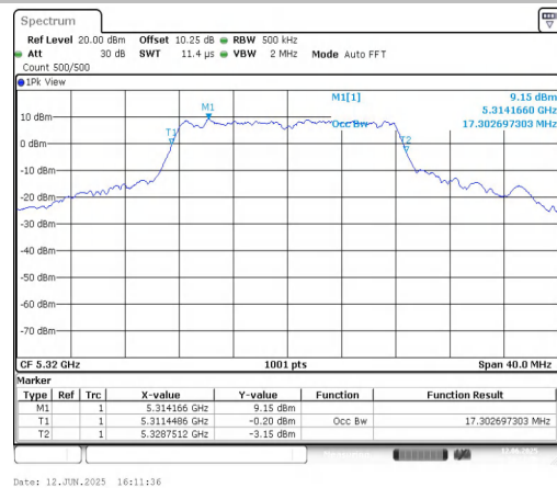
11A-Ant1-5320
