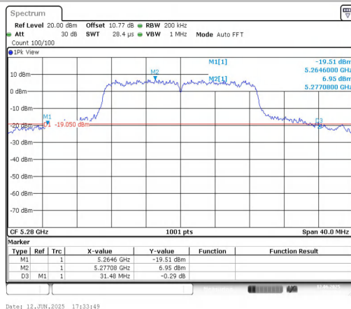
11AC20SISO-Ant1-5280
