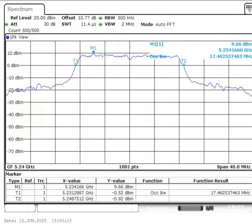
11A-Ant1-5240
