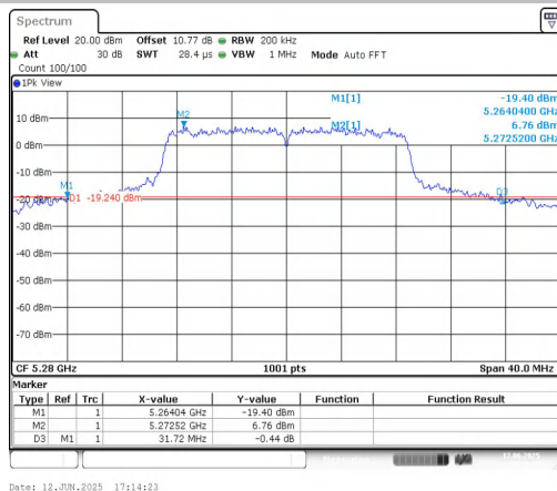
11N20SISO-Ant1-5280
