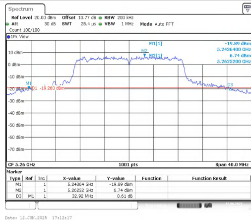
11N20SISO-Ant1-5260
