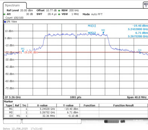
11AC20SISO-Ant1-5260
