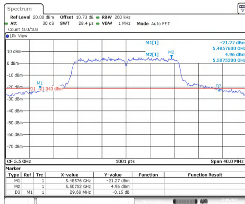
11AC20SISO-Ant1-5500
