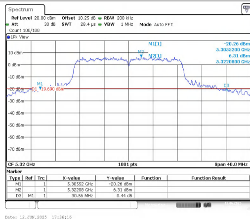
11AC20SISO-Ant1-5320
