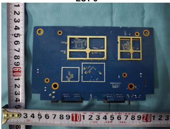
PCB board 2
