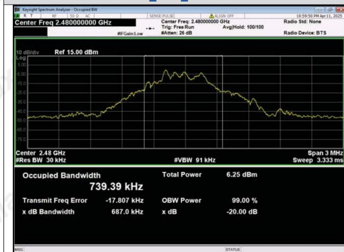
GFSK_DH5_Channel 78
