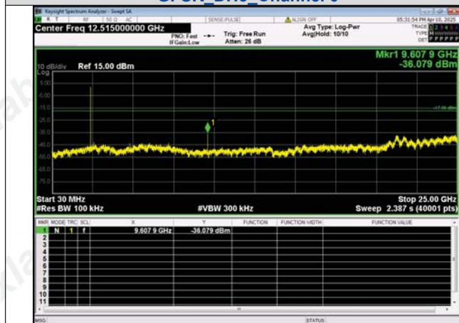
30.0 MHz - 25000.0 MHz GFSK_DH5_Channel 0
