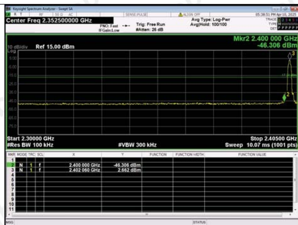
Out Of Band Emission \pi/4 DQPSK_2-DH5_Channel 0
