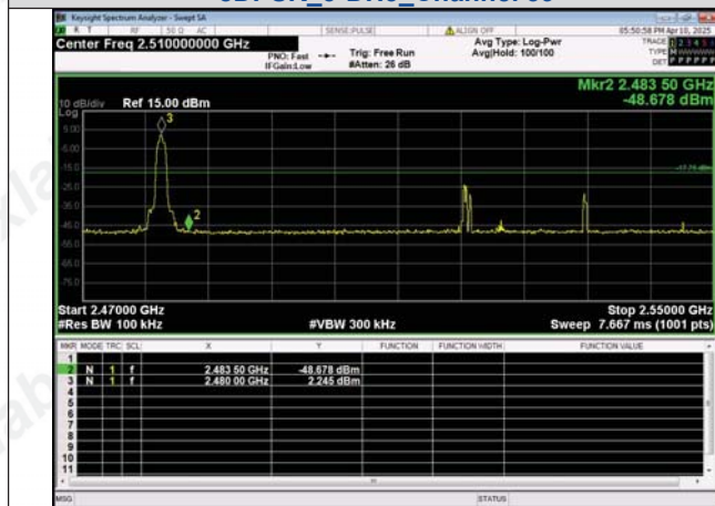
Out Of Band Emission 8DPSK_3-DH5_Channel 78
