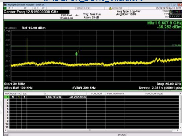
30.0 MHz - 25000.0 MHz \pi/4 DQPSK_2-DH5_Channel 0
