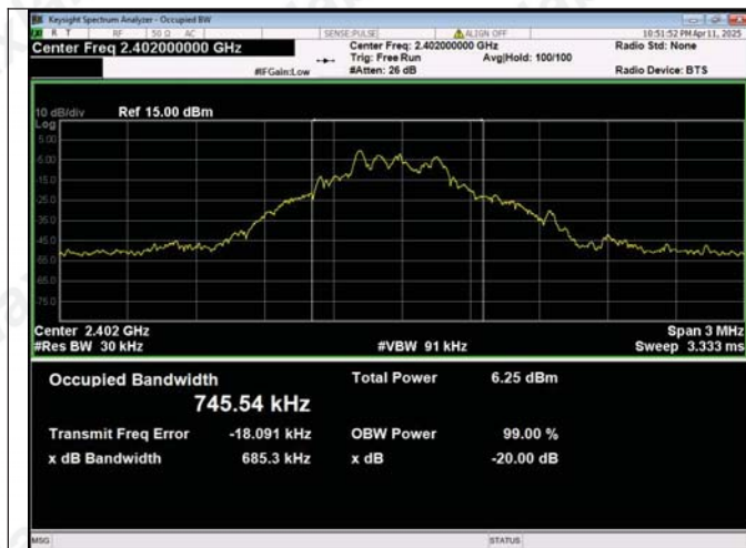
GFSK_DH5_Channel 0
