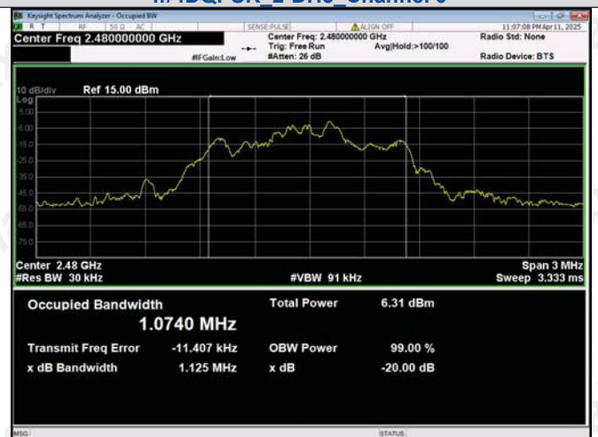
π/4DQPSK_2-DH5_Channel 78
