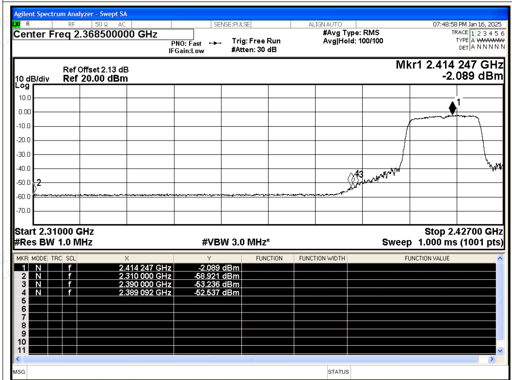
Restrict Band NVNT n20 2412MHz Ant Average
