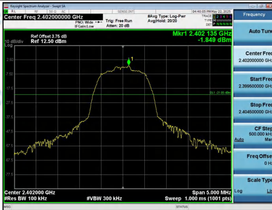
2_Bandedge_NVNT_ANT1_2-DH5_2402_00
