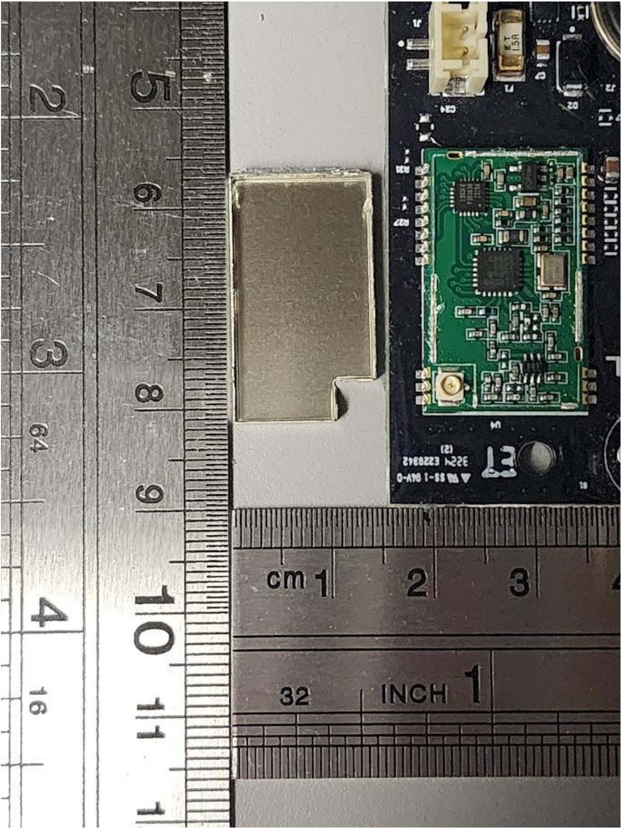
PCB Top View Close-up without shield:
