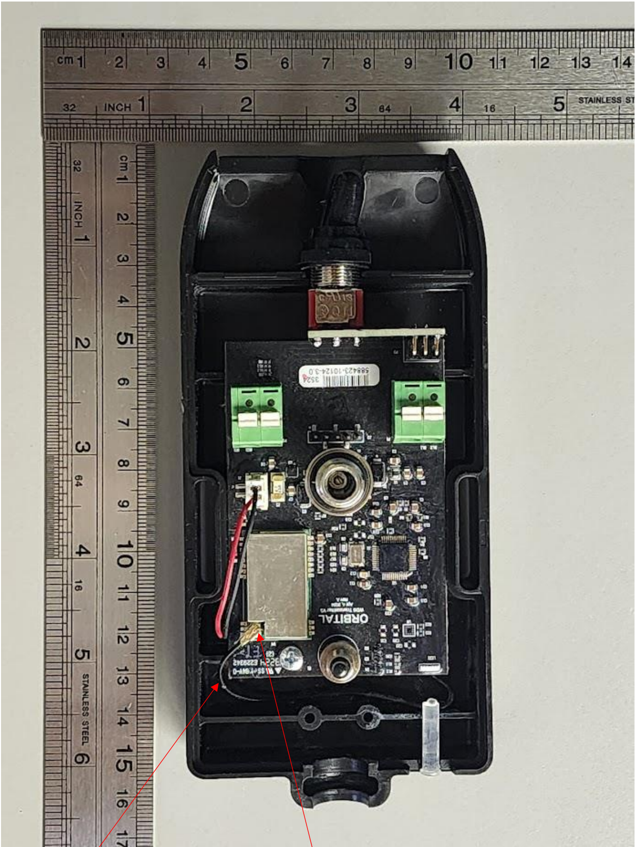
Antenna Cable
