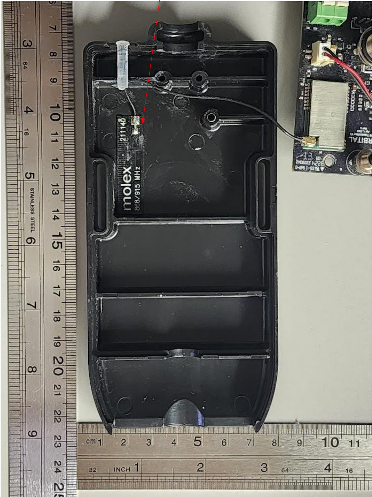
Enclosure inside view without PCB/battery: TX Antenna
