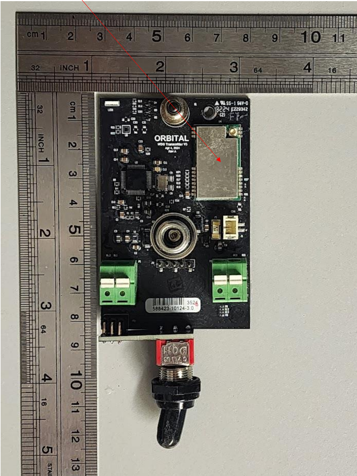
PCB Top View with Shield:
