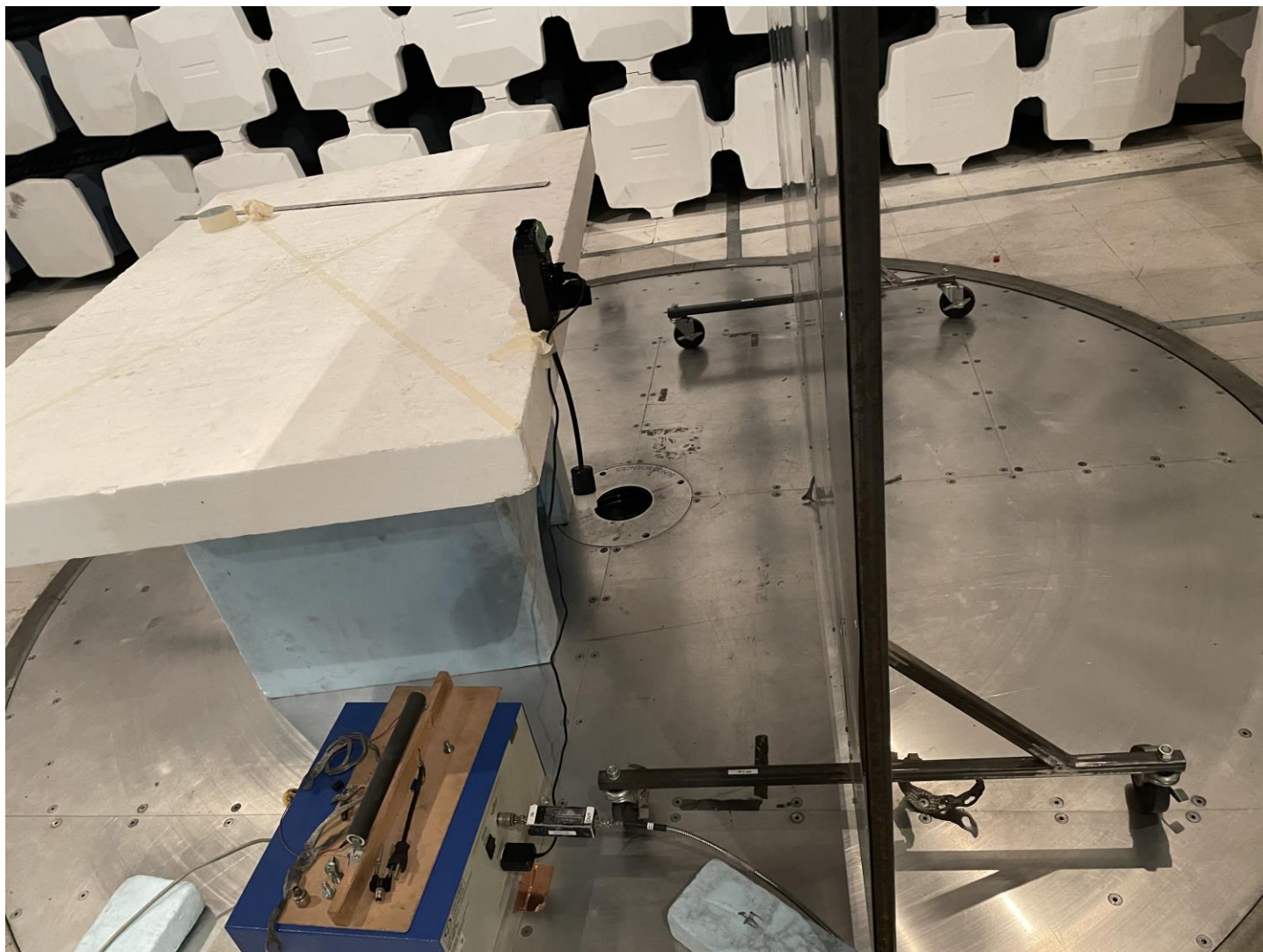
AC Main Conducte Emission test setup Photo:
