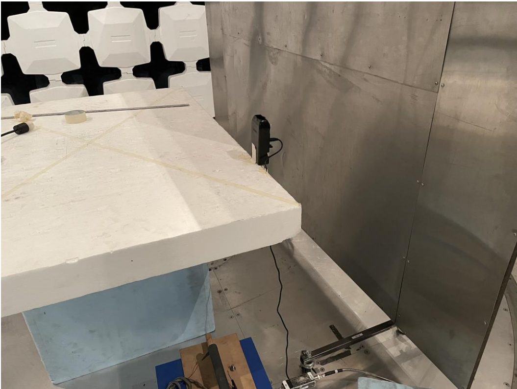
AC Main (AC/DC Adaptor) Conducted Emission test setup Photo: TX/RX Mode
