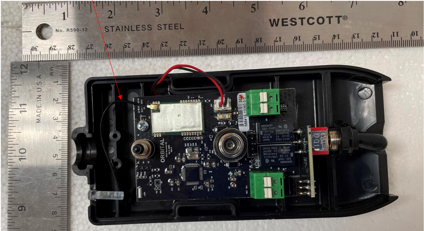
Antenna Cable
