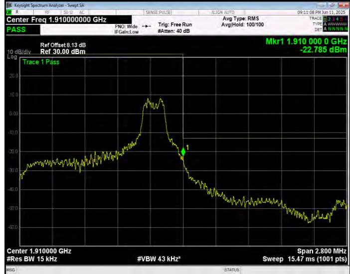
Band2 QPSK BW=1.4MHz Channel=19193 RB Size=1 Position=#Max NB Index=0
