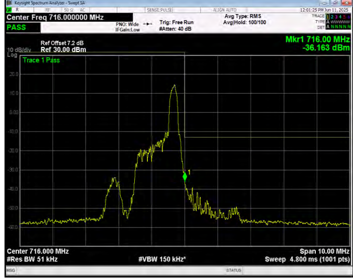
Band12 QAM16 BW=5MHz Channel=23155 RB Size=1 Position=#Max NB Index=3
