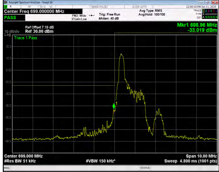
Band12 QAM16 BW=5MHz Channel=23035 RB Size=6 Position=#0 NB Index=0
