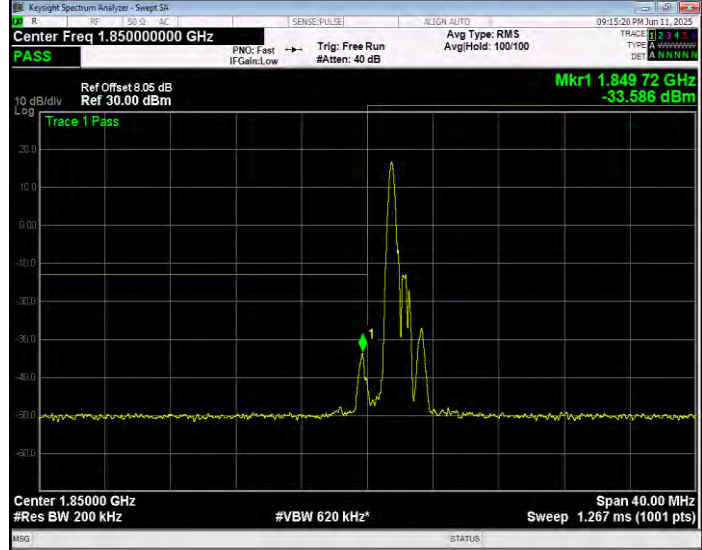
Band2 QAM16 BW=20MHz Channel=18700 RB Size=6 Position=#0 NB Index=0
