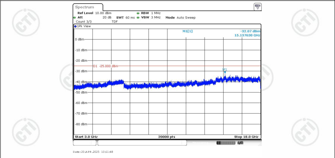
Band41-10MHz-16QAM-39700-1RB#0-Range3:3000~18000MHz
