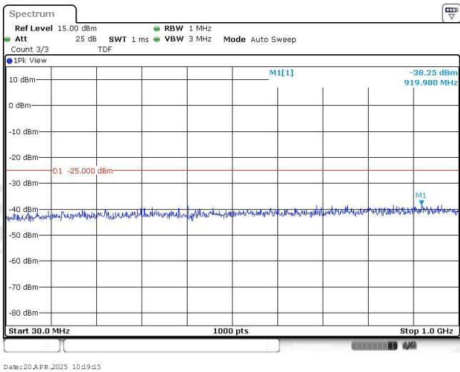
Band41-15MHz-16QAM-39725-1RB#0-Range1:30~1000MHz
