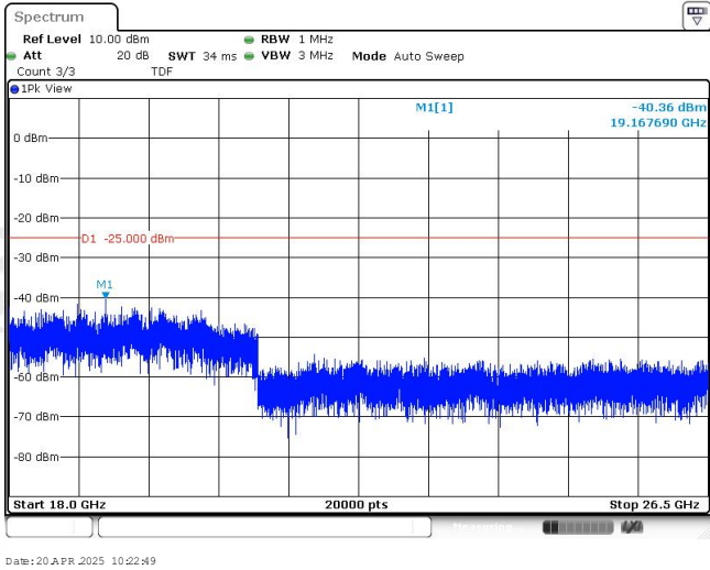
Band41-15MHz-QPSK-41515-1RB#0-Range4:18000~26500MHz
