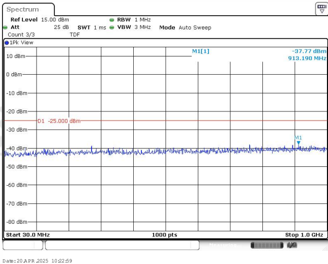
Band41-15MHz-16QAM-41515-1RB#0-Range1:30~1000MHz
