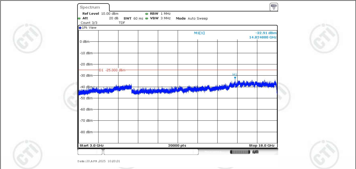
Band41-15MHz-QPSK-40620-1RB#0-Range3:3000~18000MHz
