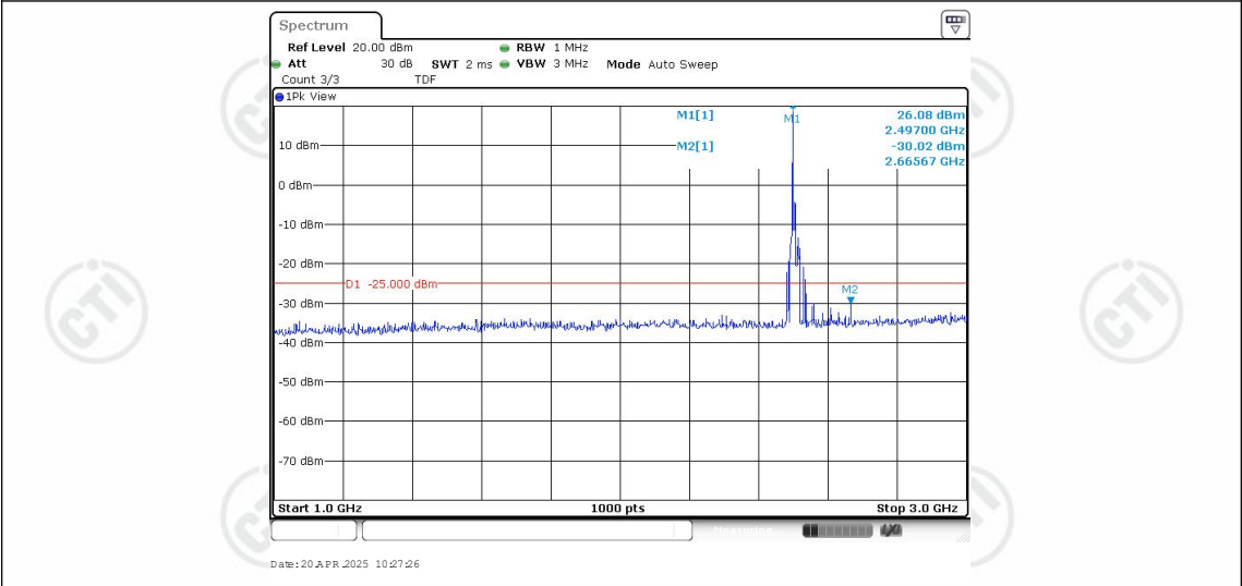
Band41-20MHz-16QAM-39750-1RB#0-Range2: 1000~3000MHz
