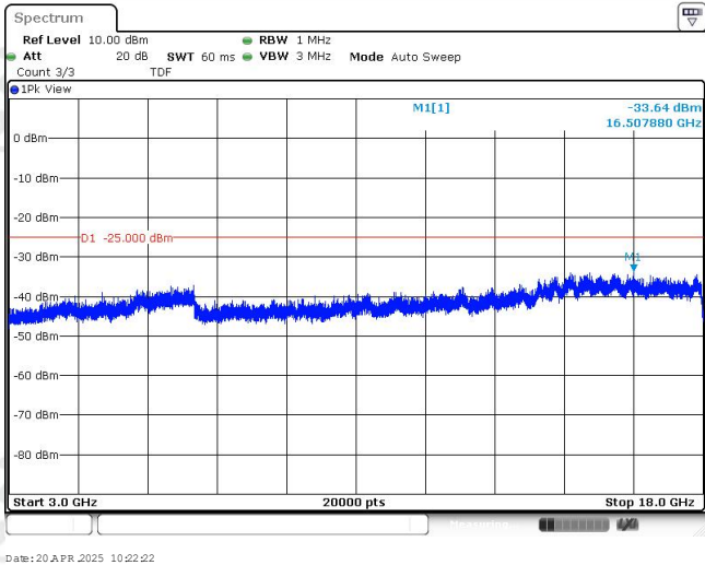
Band41-15MHz-QPSK-41515-1RB#0-Range3:3000~18000MHz
