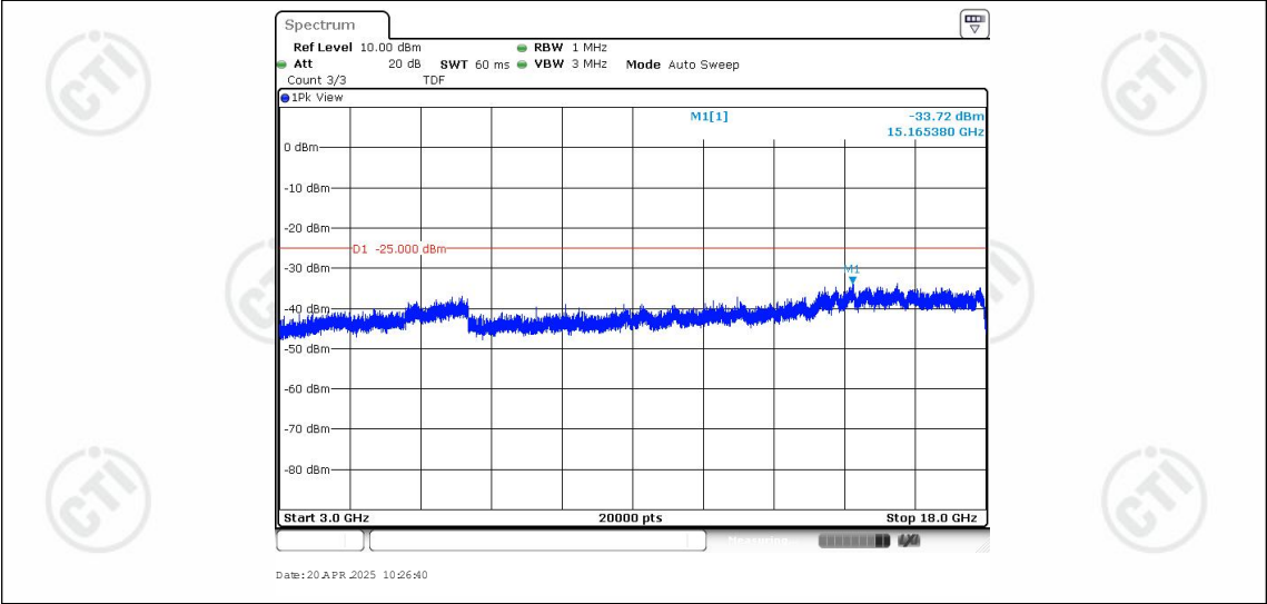
Band41-20MHz-QPSK-39750-1RB#0-Range3:3000~18000MHz
