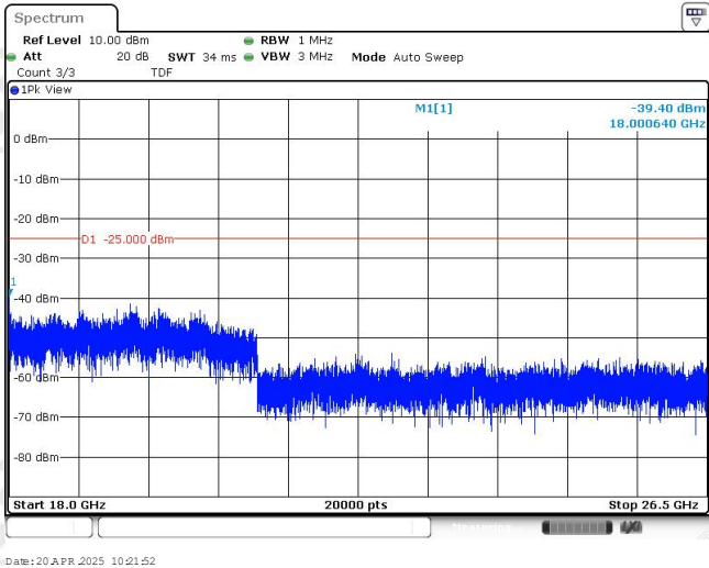
Band41-15MHz-16QAM-40620-1RB#0-Range4:18000~26500MHz
