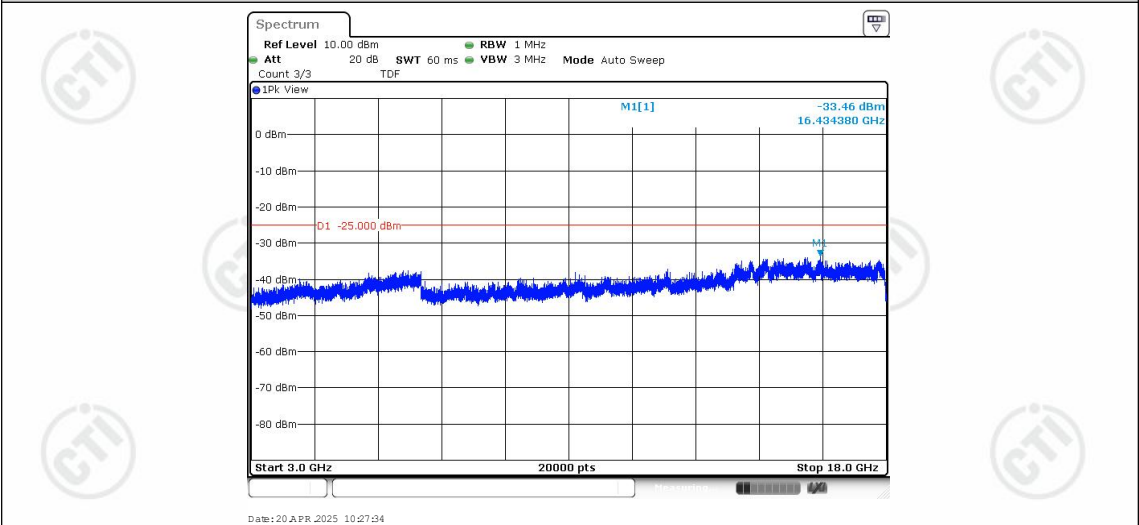
Band41-20MHz-16QAM-39750-1RB#0-Range3:3000~18000MHz
