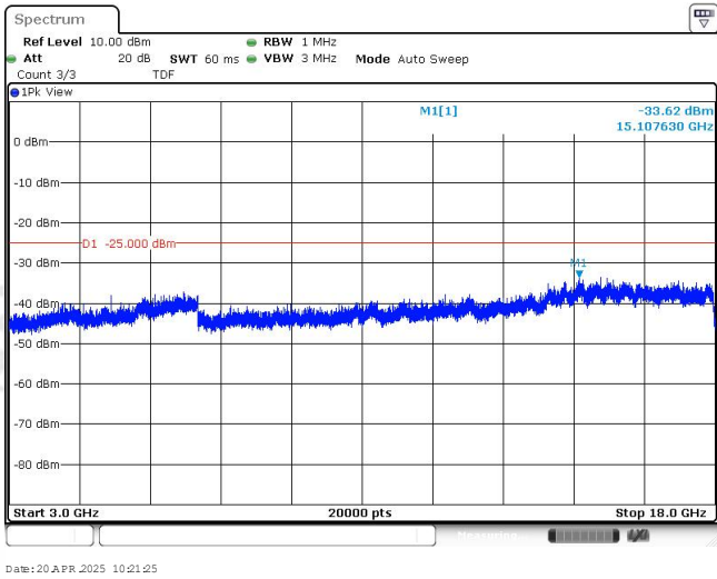
Band41-15MHz-16QAM-40620-1RB#0-Range3:3000~18000MHz
