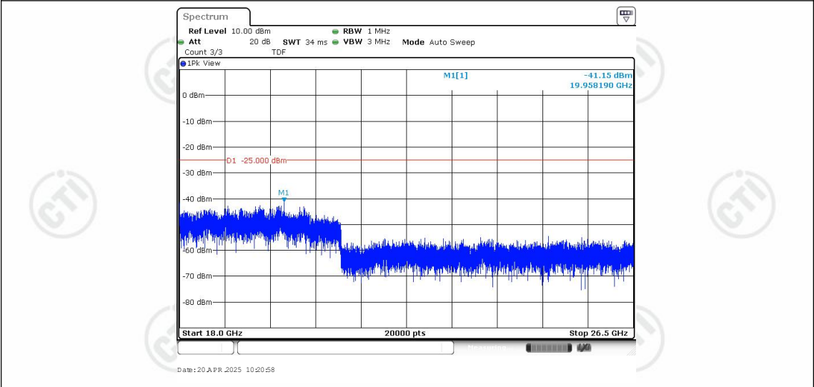
Band41-15MHz-QPSK-40620-1RB#0-Range4:18000~26500MHz
