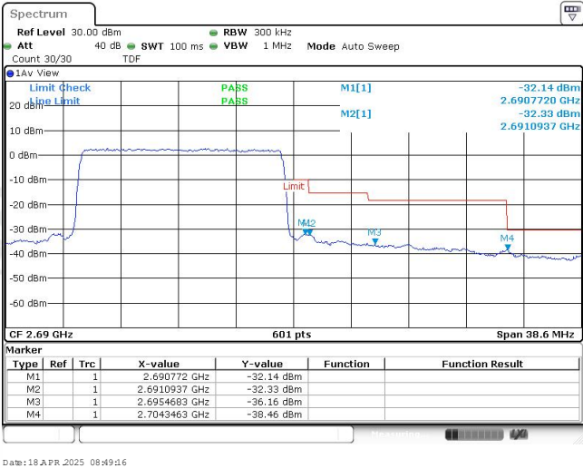
Band41-15MHz-16QAM-41515-75RB#0
