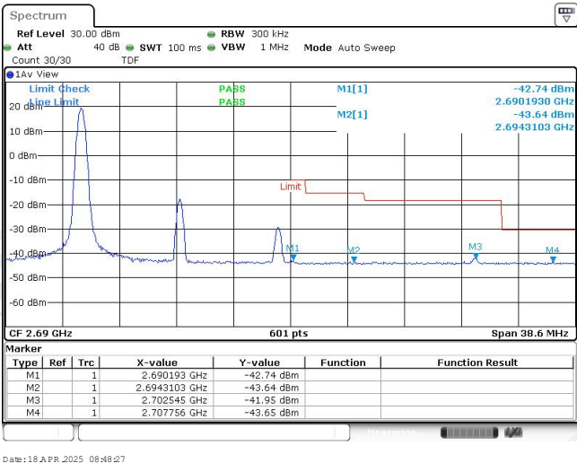
Band41-15MHz-16QAM-41515-1RB#0
