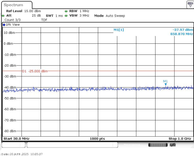
Band41-5MHz-16QAM-40620-1RB#0-Range1:30~1000MHz
