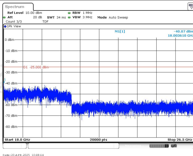
Band41-5MHz-16QAM-41565-1RB#0-Range4:18000~26500MHz
