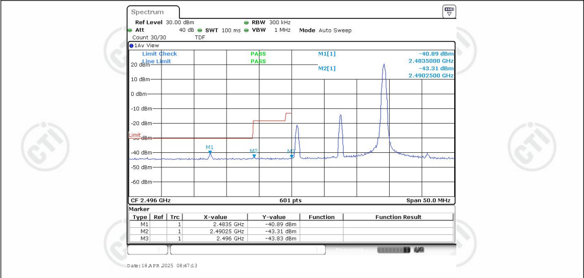
Band41-15MHz-QPSK-39725-1RB#74
