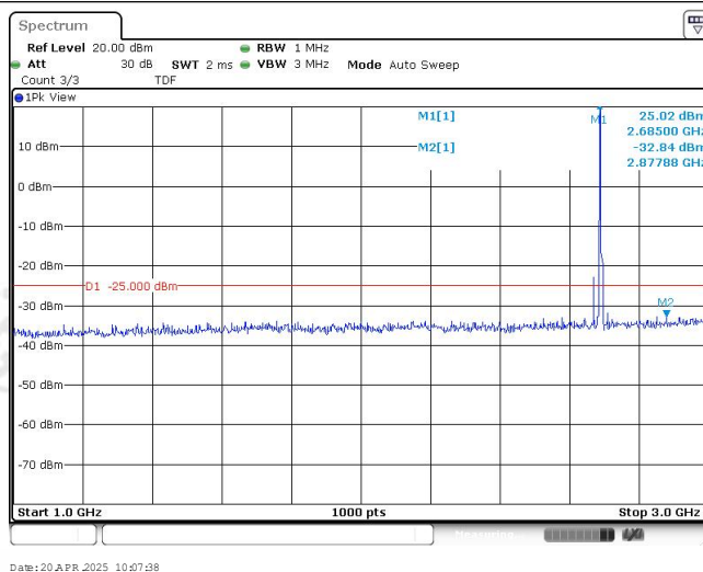
Band41-5MHz-16QAM-41565-1RB#0-Range2:1000~3000MHz
