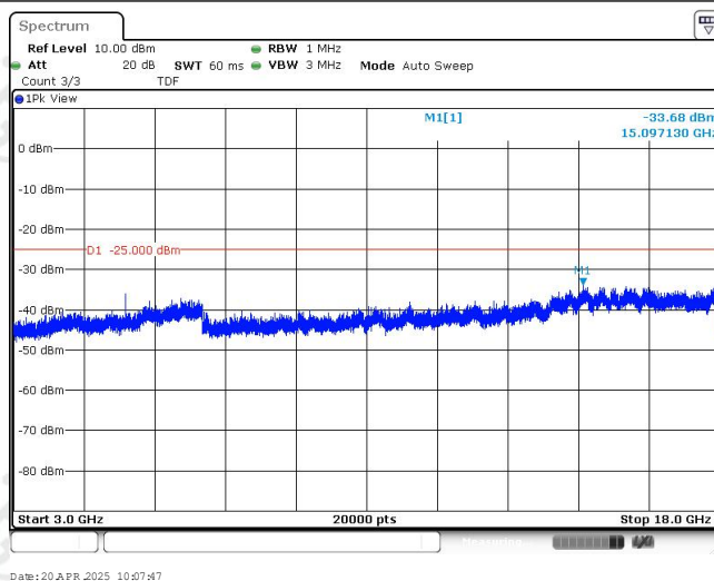
Band41-5MHz-16QAM-41565-1RB#0-Range3:3000~18000MHz
