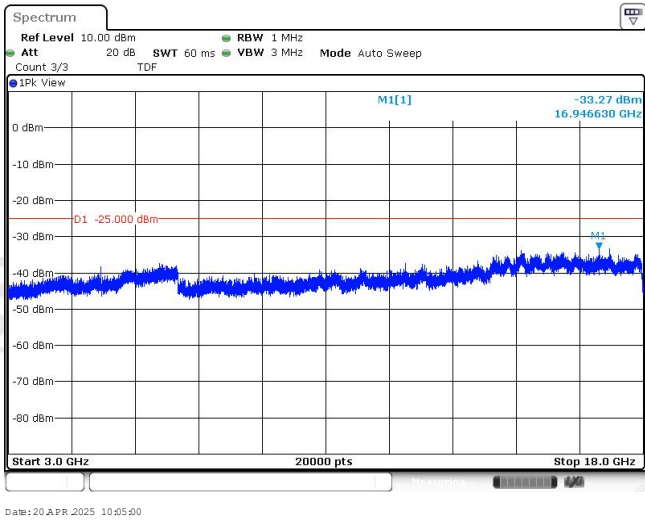
Band41-5MHz-QPSK-40620-1RB#0-Range3:3000~18000MHz
