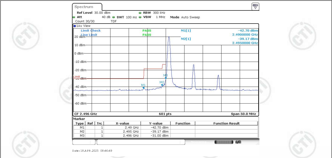
Band41-15MHz-QPSK-39725-1RB#0
