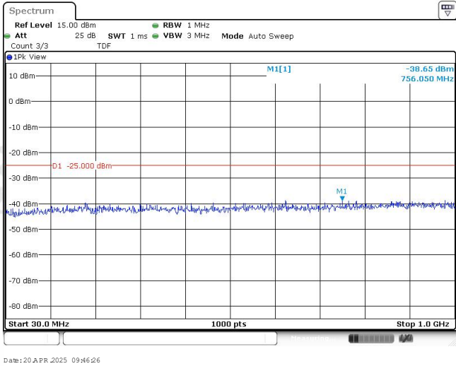
Band38-10MHz-16QAM-38000-1RB#0-Range1:30~1000MHz
