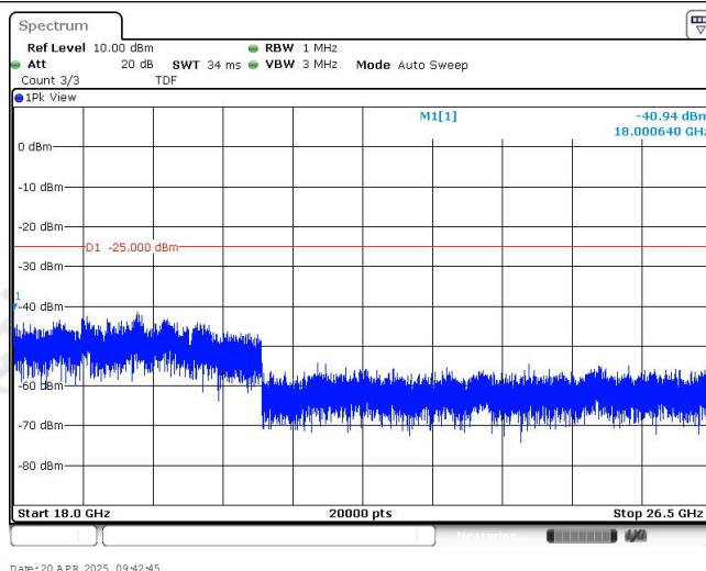
Band38-5MHz-16QAM-38225-1RB#0-Range4:18000~26500MHz
