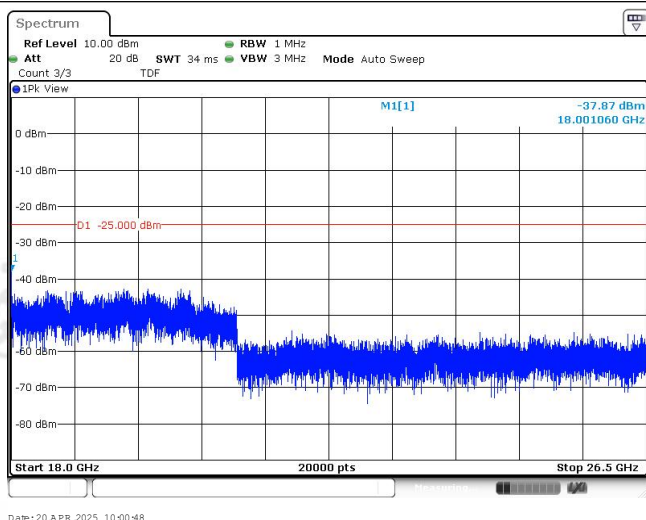
Band38-20MHz-QPSK-38150-1RB#0-Range4:18000~26500MHz
