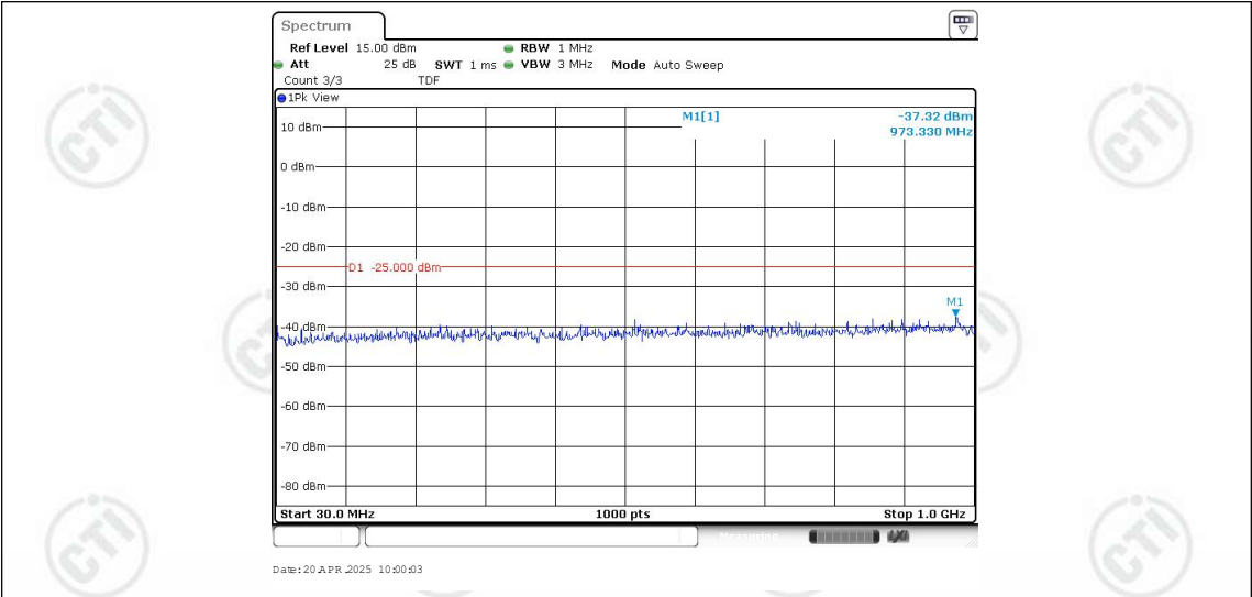
Band38-20MHz-QPSK-38150-1RB#0-Range1:30~1000MHz
