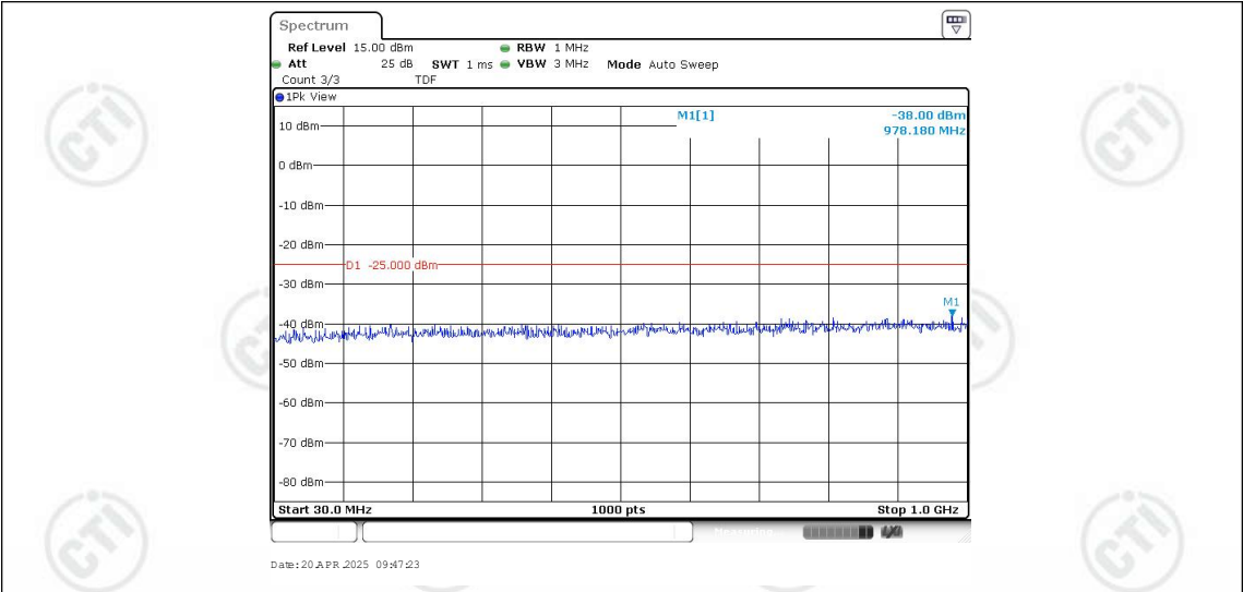
Band38-10MHz-QPSK-38200-1RB#0-Range1:30~1000MHz
