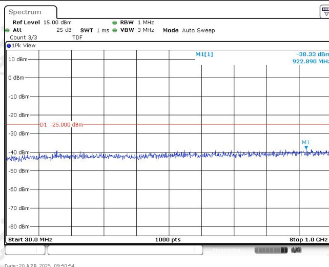
Band38-15MHz-16QAM-37825-1RB#0-Range1:30~1000MHz
