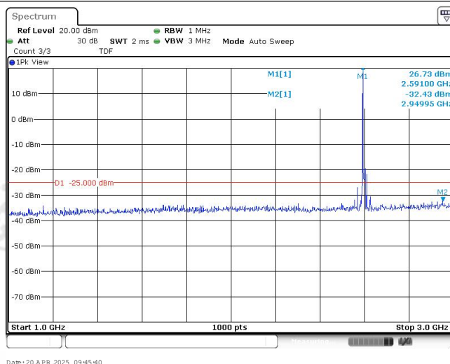
Band38-10MHz-QPSK-38000-1RB#0-Range2:1000~3000MHz
