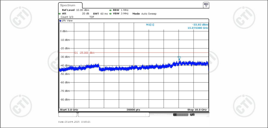
Band38-20MHz-QPSK-38150-1RB#0-Range3:3000~18000MHz
