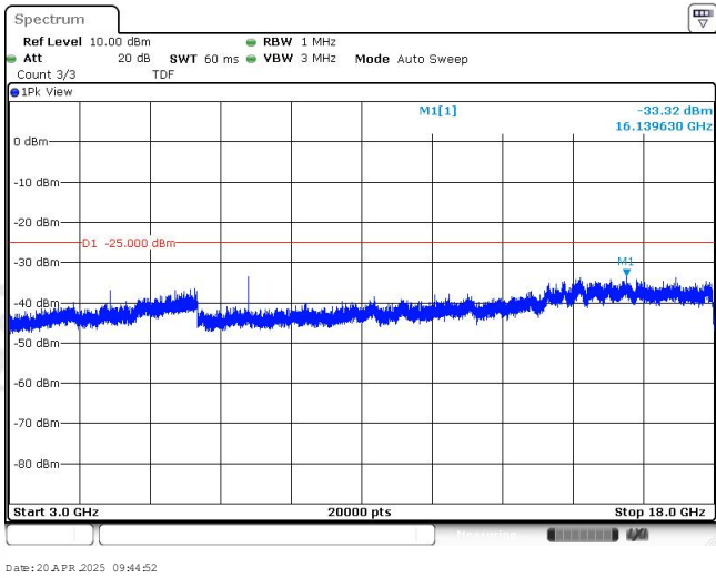
Band38-10MHz-16QAM-37800-1RB#0-Range3:3000~18000MHz
