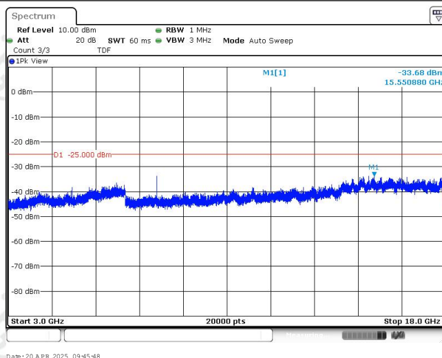
Band38-10MHz-QPSK-38000-1RB#0-Range3:3000~18000MHz
