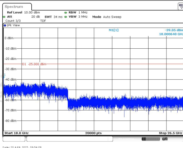
Band38-15MHz-QPSK-38175-1RB#0-Range4:18000~26500MHz
