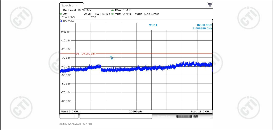
Band38-10MHz-QPSK-38200-1RB#0-Range3:3000~18000MHz
