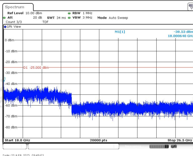
Band38-10MHz-16QAM-38200-1RB#0-Range4:18000~26500MHz
