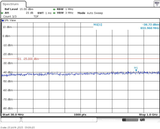
Band38-20MHz-QPSK-37850-1RB#0-Range1:30~1000MHz
