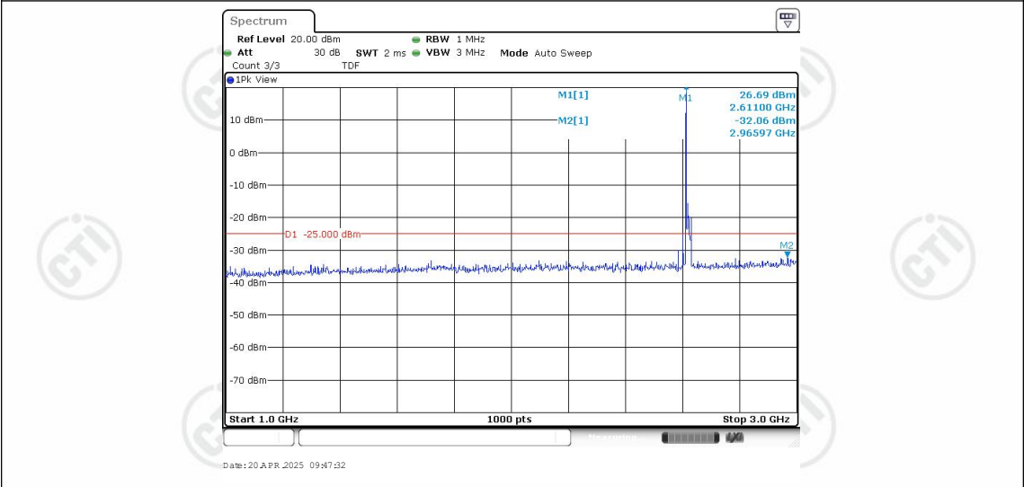
Band38-10MHz-QPSK-38200-1RB#0-Range2:1000~3000MHz
