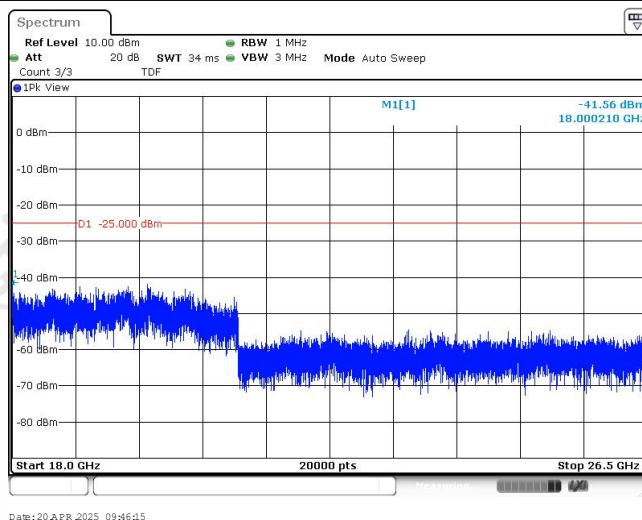
Band38-10MHz-QPSK-38000-1RB#0-Range4:18000~26500MHz
