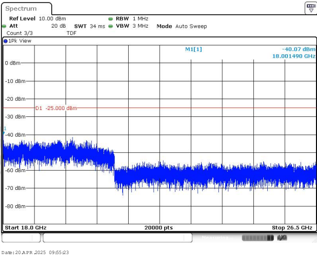
Band38-15MHz-16QAM-38175-1RB#0-Range4:18000~26500MHz
