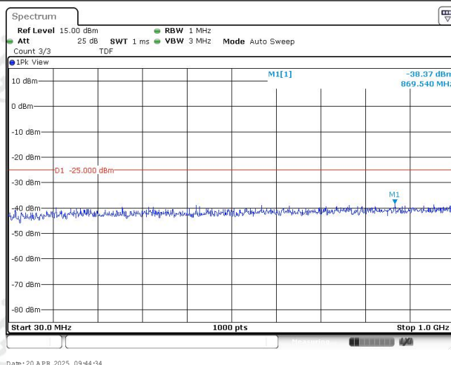
Band38-10MHz-16QAM-37800-1RB#0-Range1:30~1000MHz
