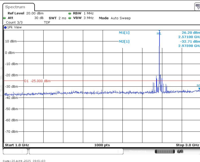
Band38-15MHz-16QAM-37825-1RB#0-Range2:1000~3000MHz
