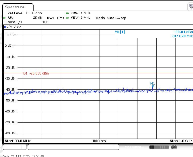
Band38-15MHz-QPSK-37825-1RB#0-Range1:30~1000MHz
