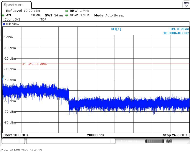
Band38-10MHz-16QAM-37800-1RB#0-Range4:18000~26500MHz
