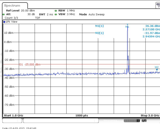
Band38-10MHz-QPSK-37800-1RB#0-Range2:1000~3000MHz
