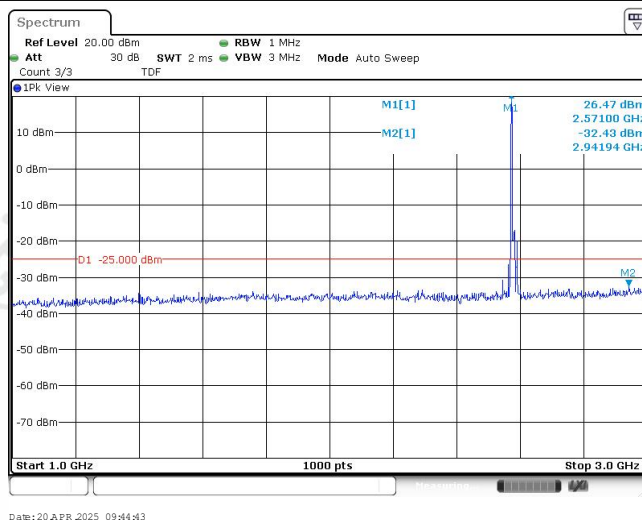
Band38-10MHz-16QAM-37800-1RB#0-Range2:1000~3000MHz
