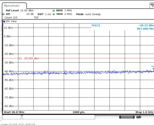
Band38-10MHz-QPSK-37800-1RB#0-Range1:30~1000MHz
