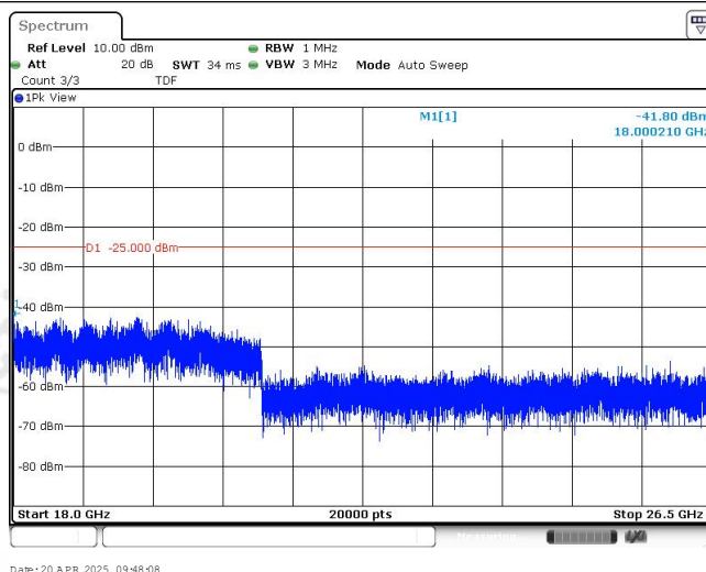
Band38-10MHz-QPSK-38200-1RB#0-Range4:18000~26500MHz
