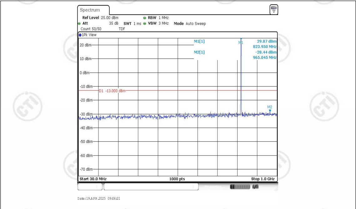
Band26-1.4MHz-QPSK-26785-1RB#0-Range1:30~1000MHz
