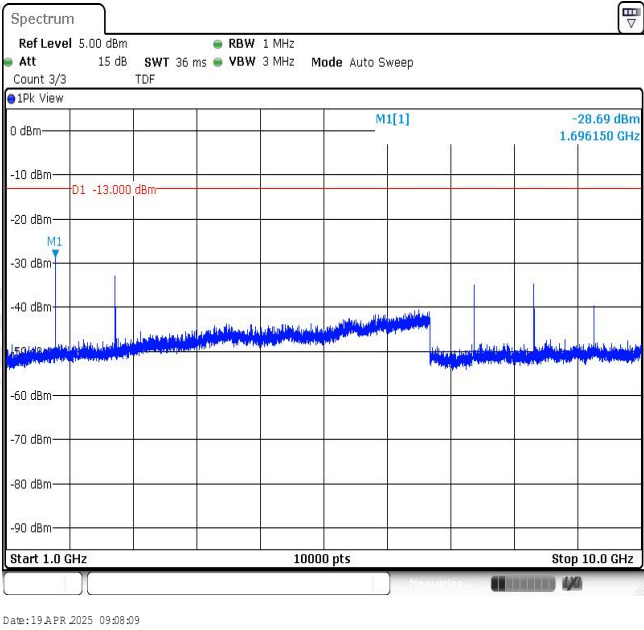
Band26-1.4MHz-16QAM-27033-1RB#0-Range2:1000~10000MHz
