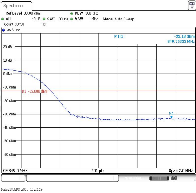
Band26-15MHz-16QAM-26965-75RB#0
