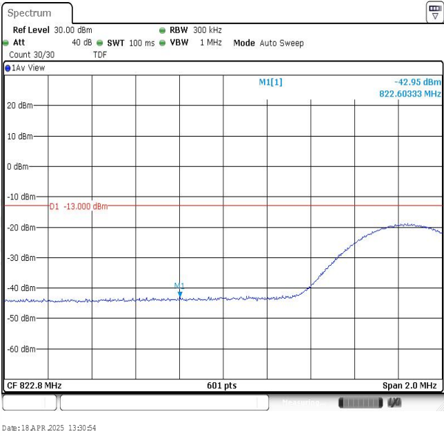
Band26-15MHz-16QAM-26853-1RB#74
