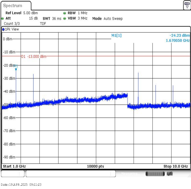
Band26-3MHz-16QAM-26909-1RB#0-Range2:1000~10000MHz
