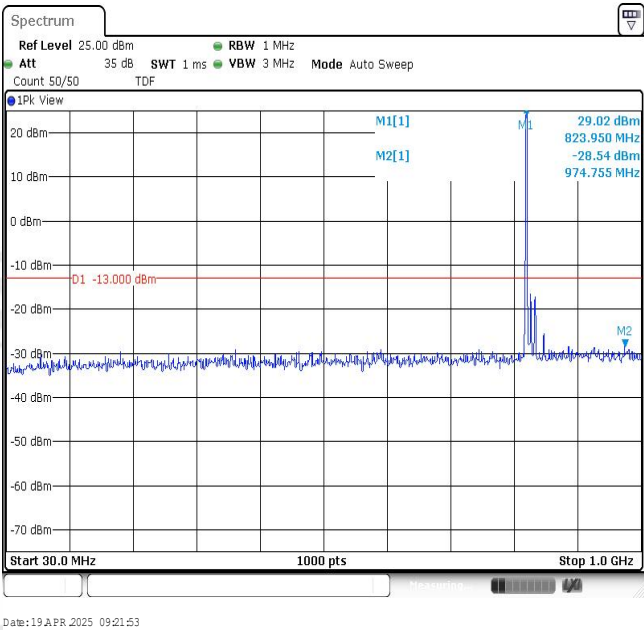
Band26-15MHz-16QAM-26853-1RB#0-Range1:30~1000MHz
