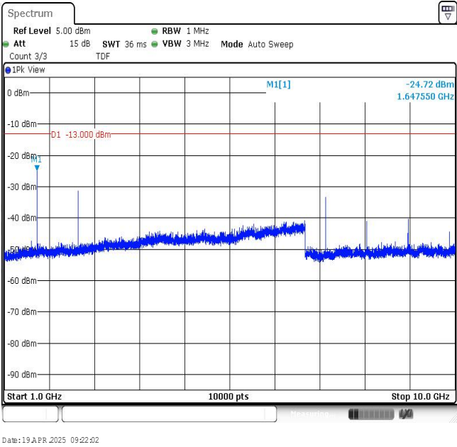
Band26-15MHz-16QAM-26853-1RB#0-Range2:1000~10000MHz
