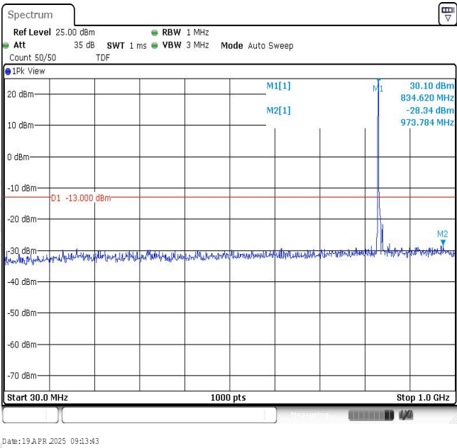
Band26-5MHz-16QAM-26909-1RB#0-Range1:30~1000MHz
