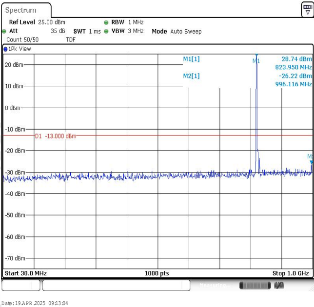
Band26-5MHz-16QAM-26803-1RB#0-Range1:30~1000MHz
