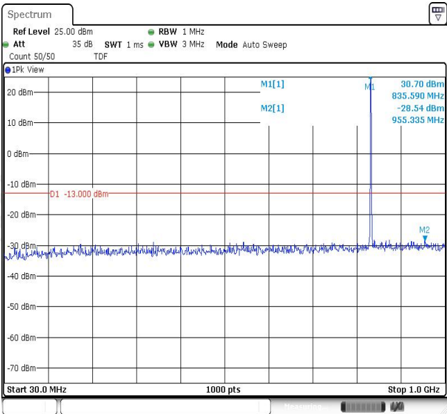
Band26-1.4MHz-QPSK-26909-1RB#0-Range1:30~1000MHz
