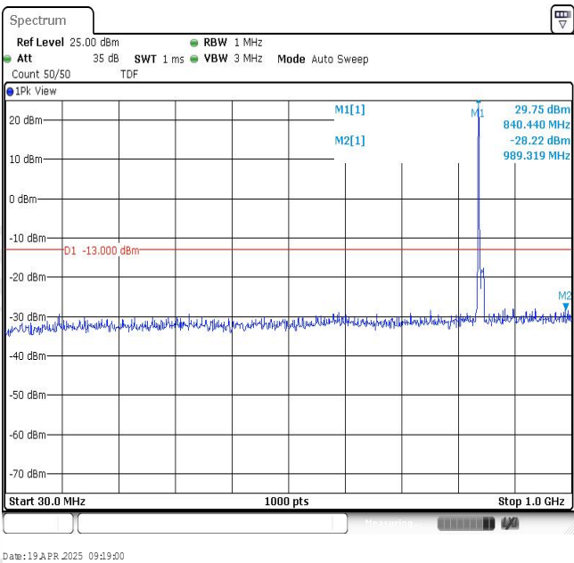
Band26-10MHz-16QAM-26990-1RB#0-Range1:30~1000MHz
