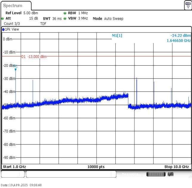
Band26-1.4MHz-16QAM-26785-1RB#0-Range2:1000~10000MHz
