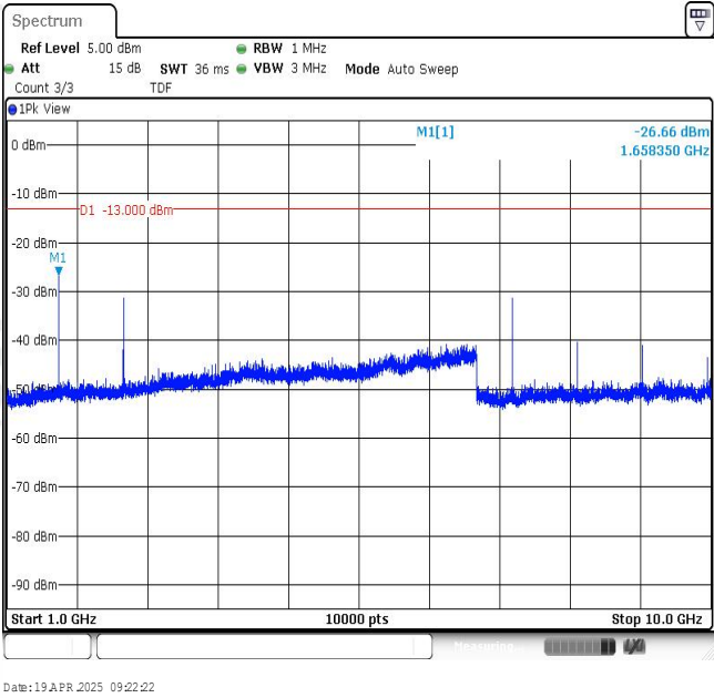
Band26-15MHz-QPSK-26909-1RB#0-Range2:1000~10000MHz
