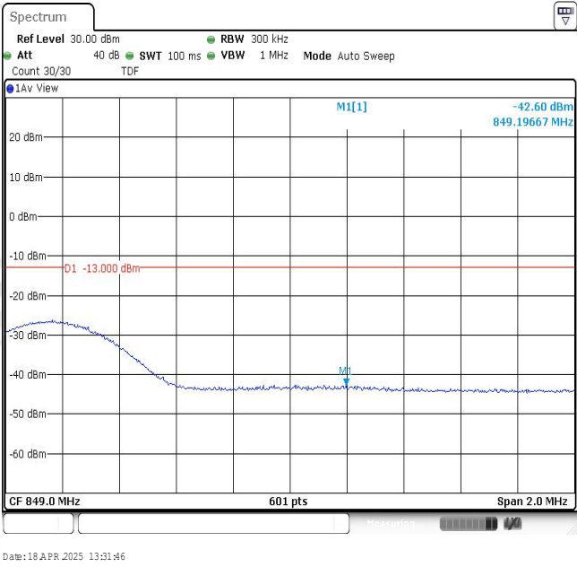
Band26-15MHz-16QAM-26965-1RB#0
