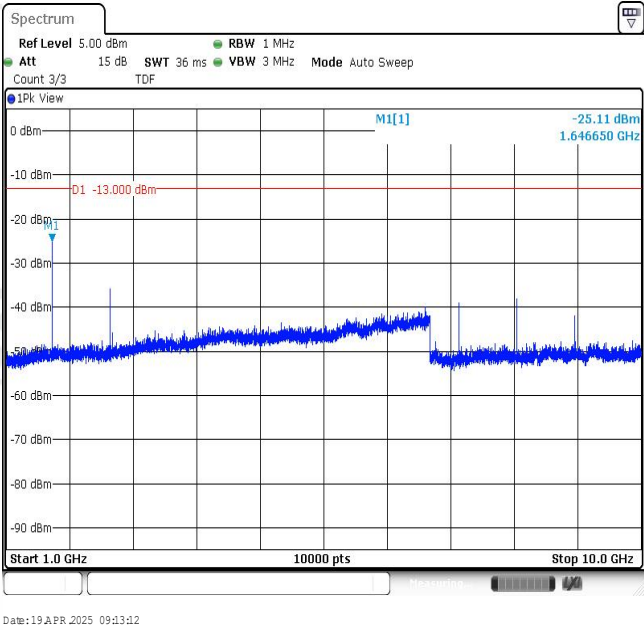
Band26-5MHz-16QAM-26803-1RB#0-Range2:1000~10000MHz
