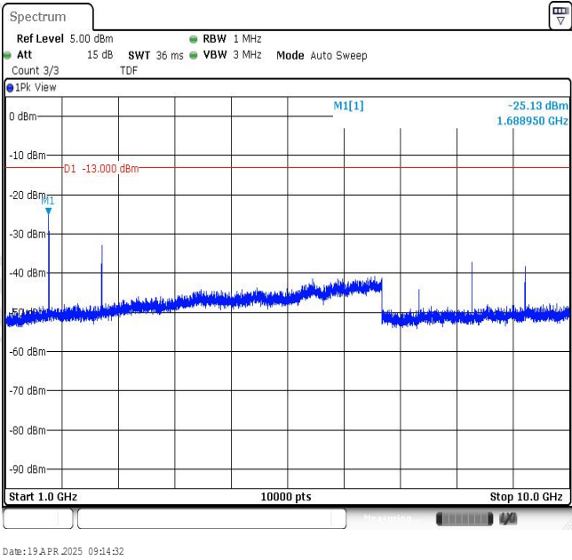
Band26-5MHz-16QAM-27015-1RB#0-Range2:1000~10000MHz
