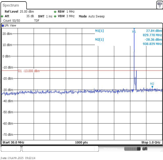
Band26-15MHz-QPSK-26909-1RB#0-Range1:30~1000MHz
