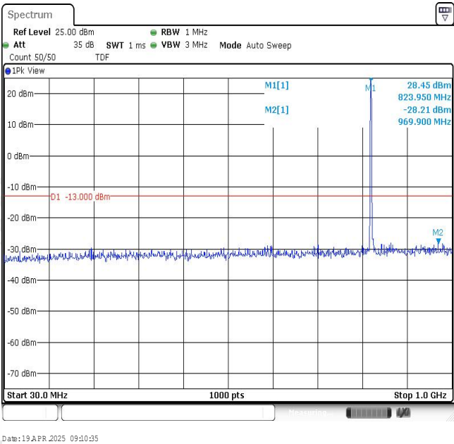
Band26-3MHz-16QAM-26793-1RB#0-Range1:30~1000MHz
