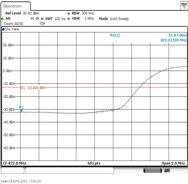
Band26-15MHz-16QAM-26853-75RB#0
