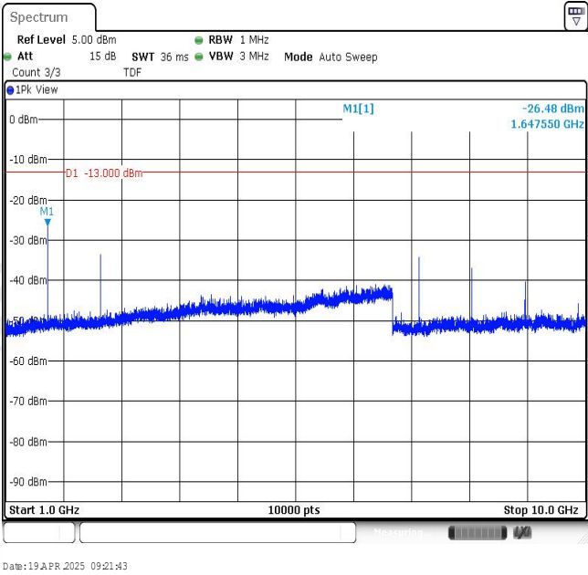
Band26-15MHz-QPSK-26853-1RB#0-Range2:1000~10000MHz
