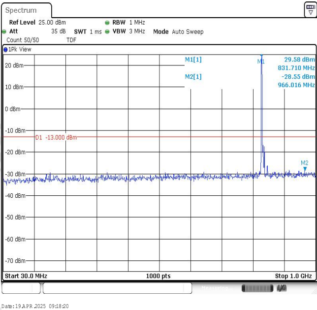
Band26-10MHz-16QAM-26909-1RB#0-Range1:30~1000MHz
