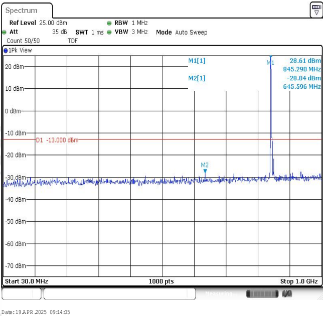
Band26-5MHz-QPSK-27015-1RB#0-Range1:30~1000MHz
