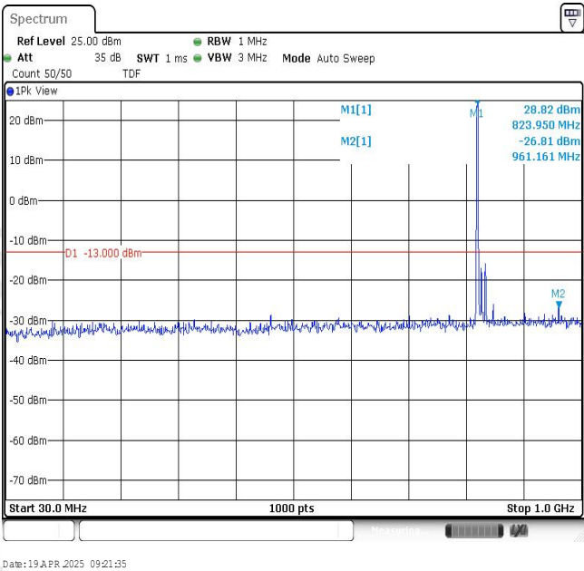
Band26-15MHz-QPSK-26853-1RB#0-Range1:30~1000MHz
