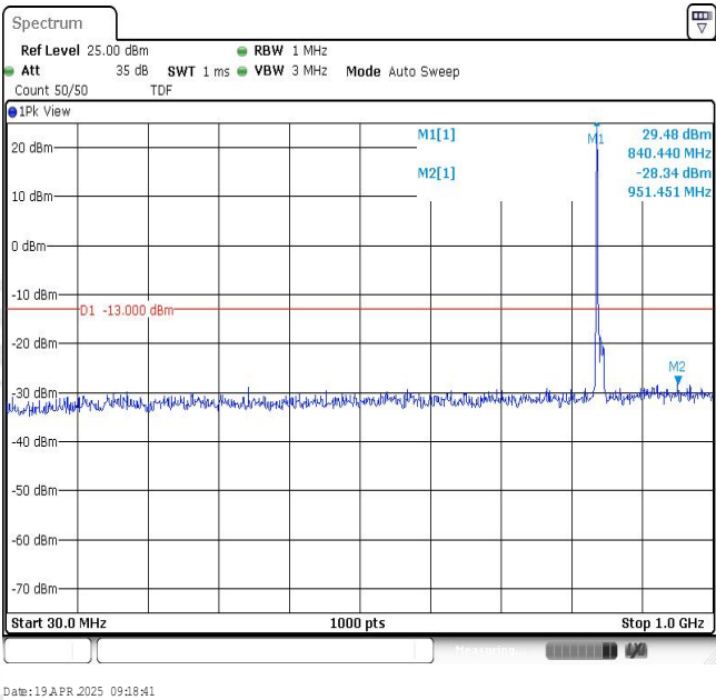
Band26-10MHz-QPSK-26990-1RB#0-Range1:30~1000MHz
