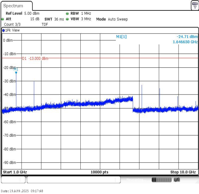
Band26-10MHz-16QAM-26828-1RB#0-Range2:1000~10000MHz
