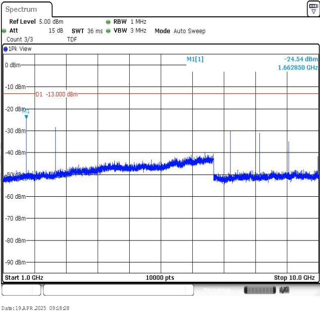
Band26-10MHz-16QAM-26909-1RB#0-Range2:1000~10000MHz
