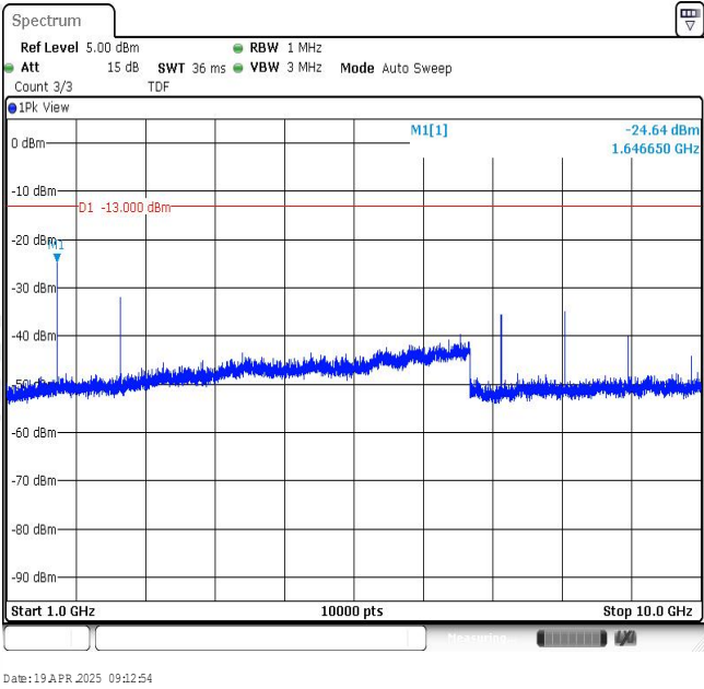
Band26-5MHz-QPSK-26803-1RB#0-Range2:1000~10000MHz
