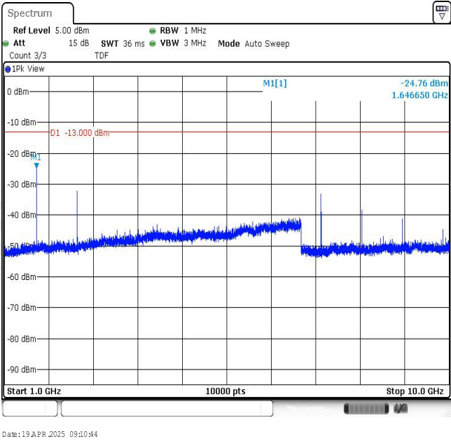
Band26-3MHz-16QAM-26793-1RB#0-Range2:1000~10000MHz
