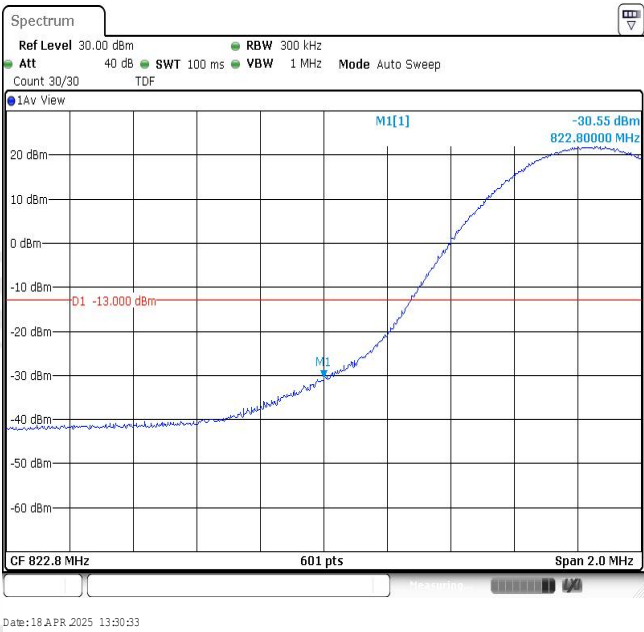
Band26-15MHz-16QAM-26853-1RB#0
