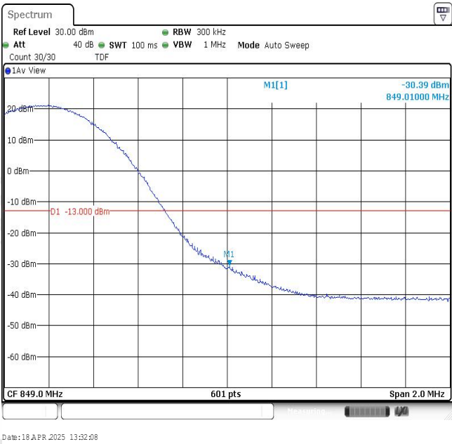
Band26-15MHz-16QAM-26965-1RB#74
