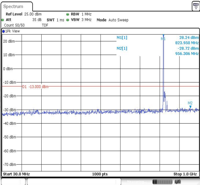
Band26-10MHz-QPSK-26828-1RB#0-Range1:30~1000MHz
