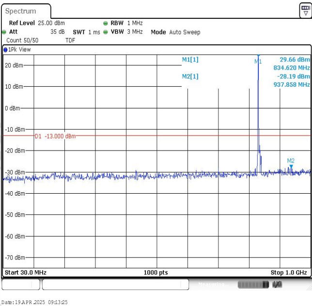
Band26-5MHz-QPSK-26909-1RB#0-Range1:30~1000MHz
