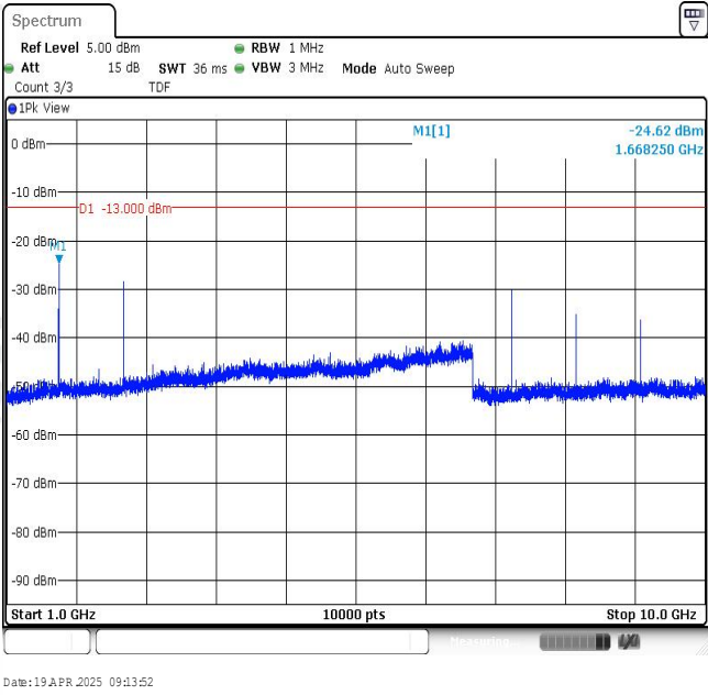
Band26-5MHz-16QAM-26909-1RB#0-Range2:1000~10000MHz
