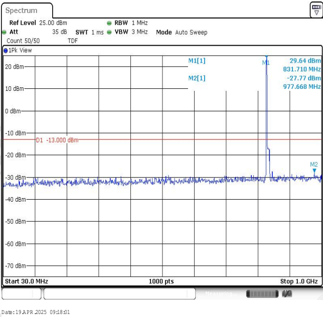
Band26-10MHz-QPSK-26909-1RB#0-Range1:30~1000MHz
