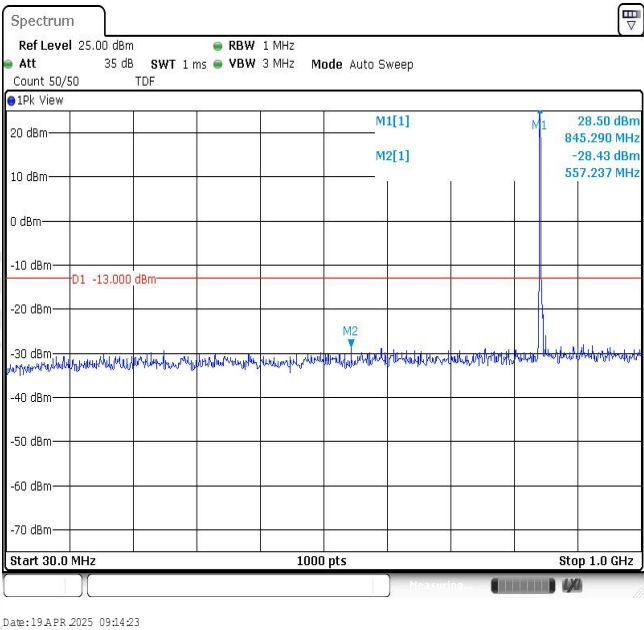
Band26-5MHz-16QAM-27015-1RB#0-Range1:30~1000MHz
