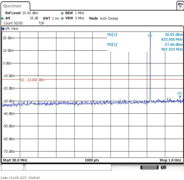
Band26-1.4MHz-16QAM-26785-1RB#0-Range1:30~1000MHz
