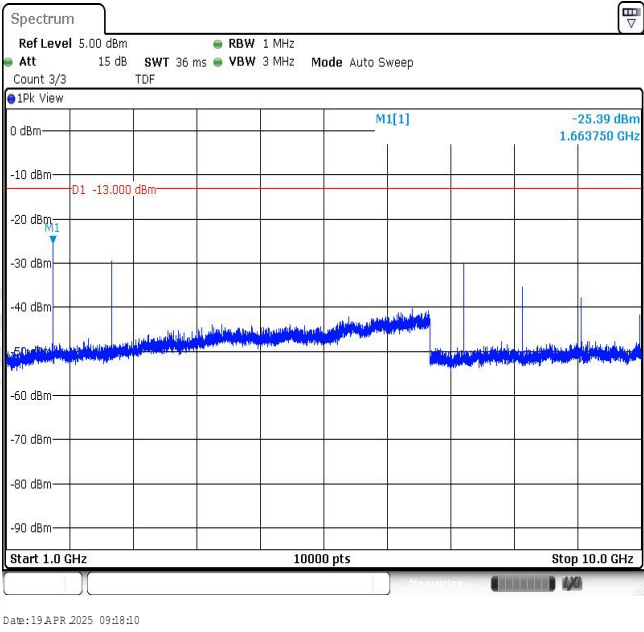
Band26-10MHz-QPSK-26909-1RB#0-Range2:1000~10000MHz
