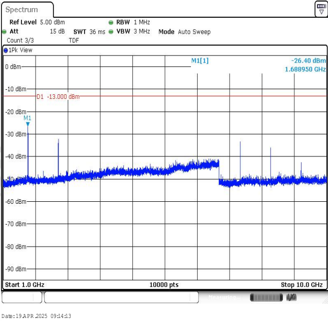
Band26-5MHz-QPSK-27015-1RB#0-Range2:1000~10000MHz
