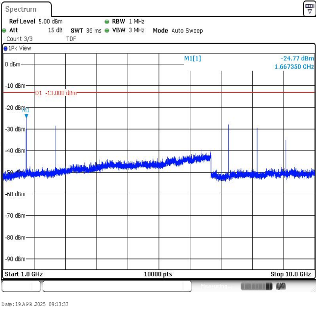
Band26-5MHz-QPSK-26909-1RB#0-Range2:1000~10000MHz
