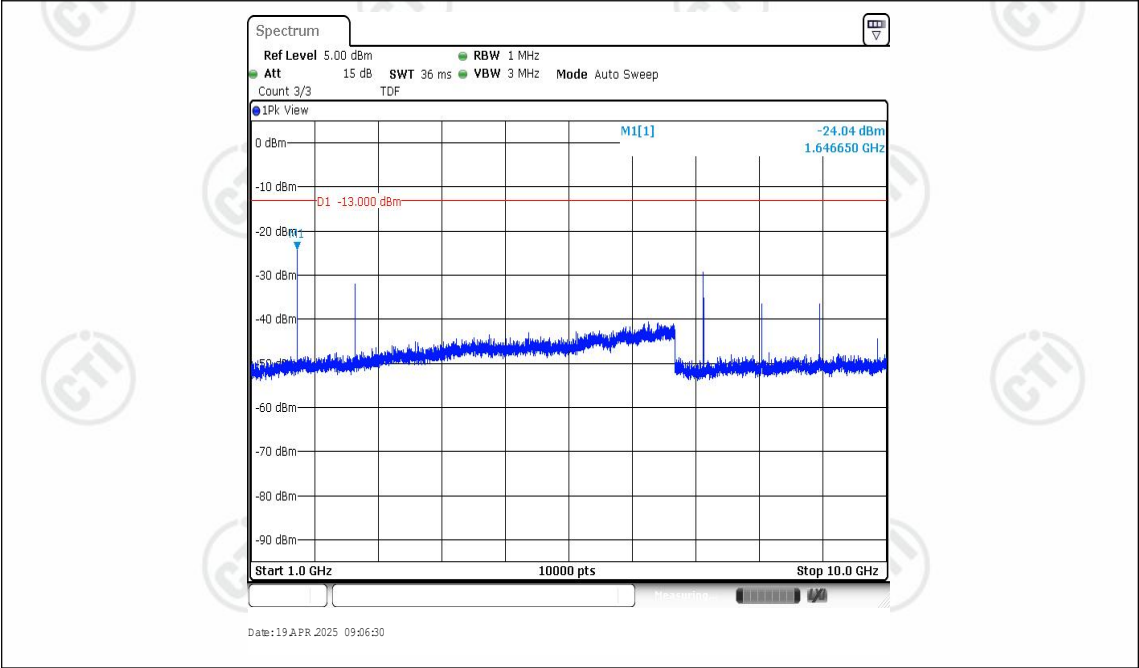
Band26-1.4MHz-QPSK-26785-1RB#0-Range2:1000~10000MHz
