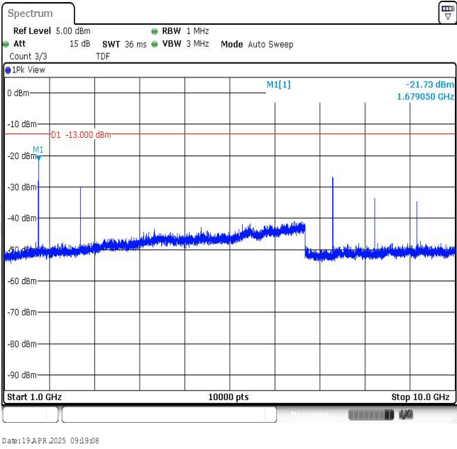
Band26-10MHz-16QAM-26990-1RB#0-Range2:1000~10000MHz
