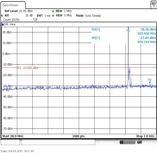
Band26-10MHz-16QAM-26828-1RB#0-Range1:30~1000MHz
