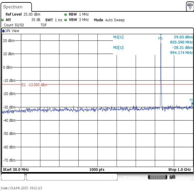
Band26-3MHz-16QAM-26909-1RB#0-Range1:30~1000MHz
