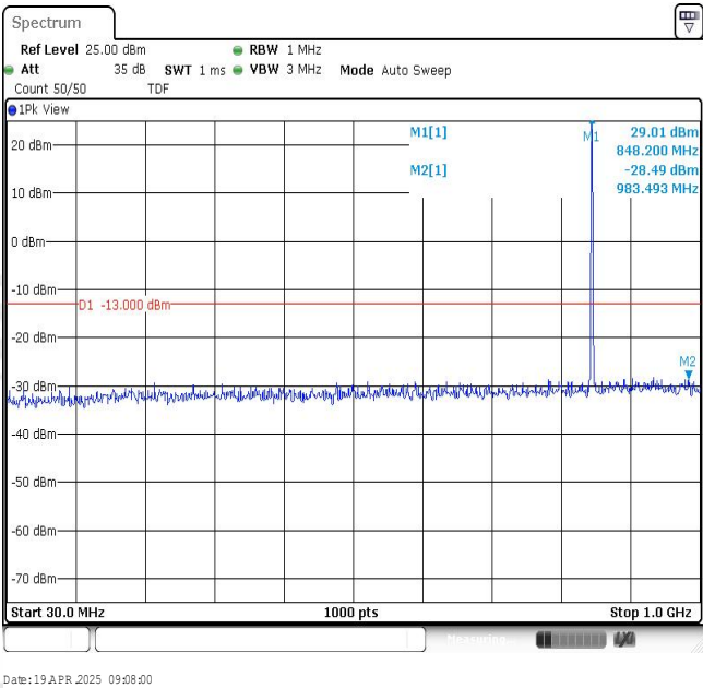
Band26-1.4MHz-16QAM-27033-1RB#0-Range1:30~1000MHz
