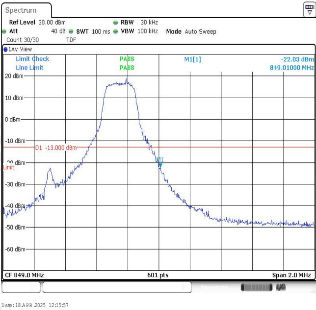
Band26-1.4MHz-QPSK-27033-1RB#5
