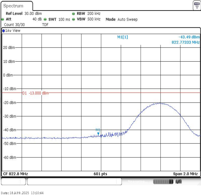
Band26-10MHz-16QAM-26828-1RB#49
