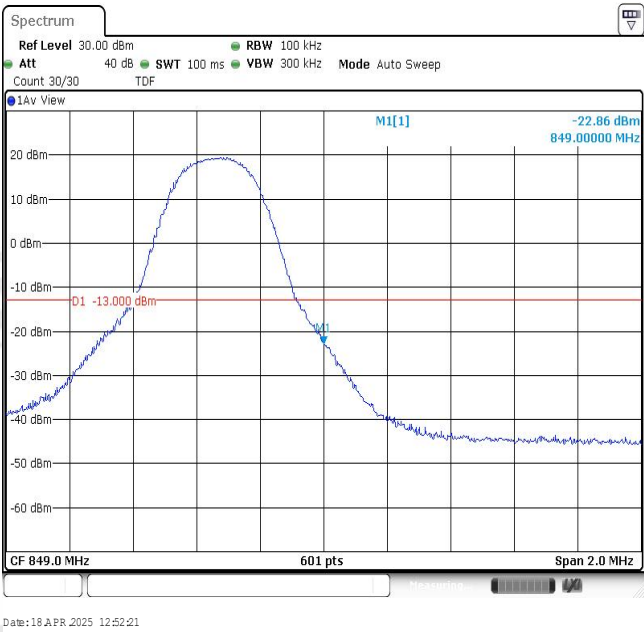
Band26-5MHz-16QAM-27015-1RB#24
