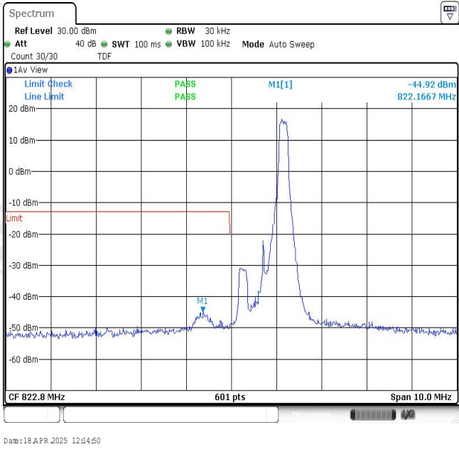
Band26-1.4MHz-16QAM-26785-1RB#5
