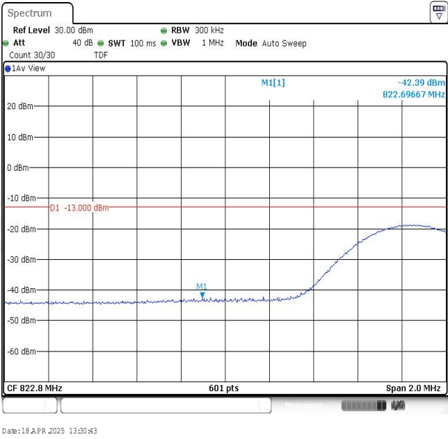
Band26-15MHz-QPSK-26853-1RB#74
