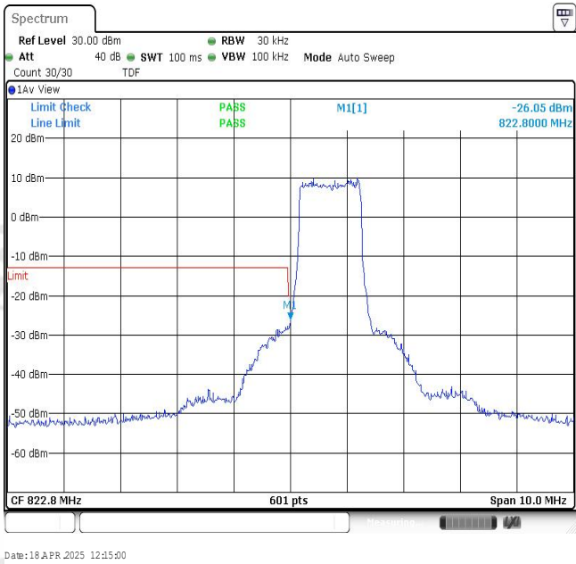
Band26-1.4MHz-QPSK-26785-6RB#0
