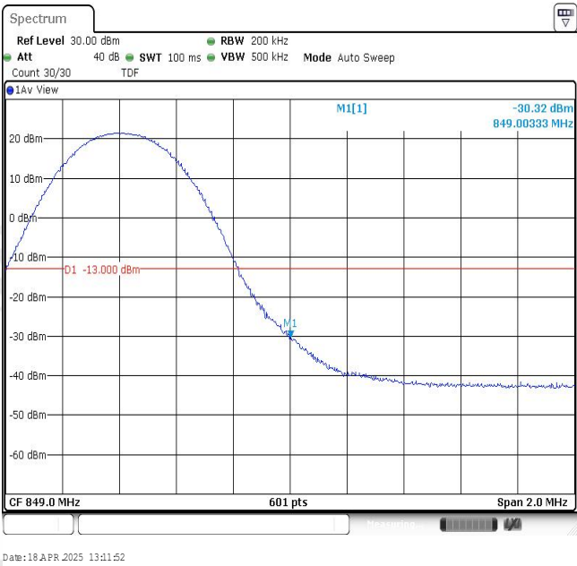
Band26-10MHz-QPSK-26990-1RB#49
