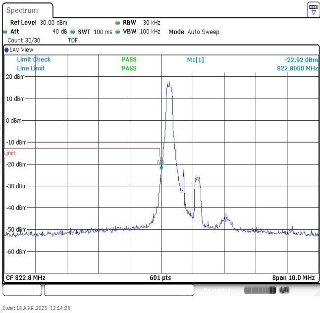
Band26-1.4MHz-16QAM-26785-1RB#0
