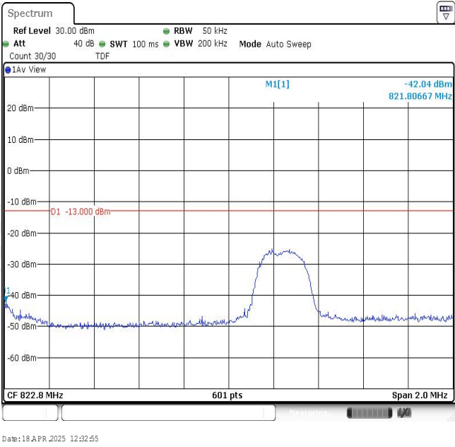
Band26-3MHz-16QAM-26793-1RB#14
