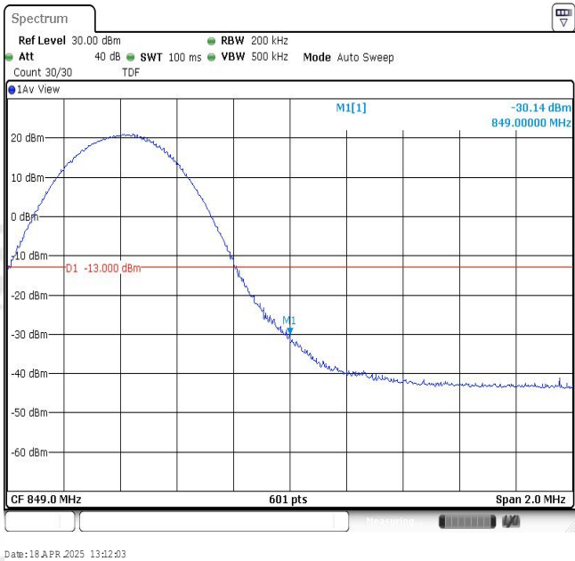
Band26-10MHz-16QAM-26990-1RB#49
