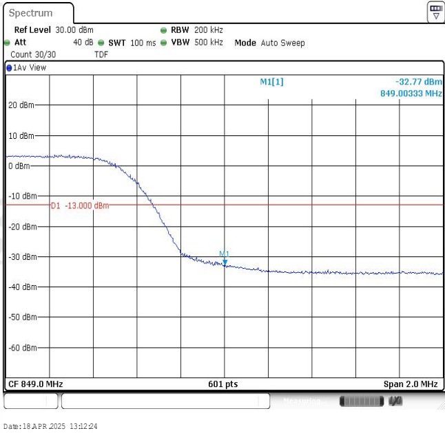
Band26-10MHz-16QAM-26990-50RB#0
