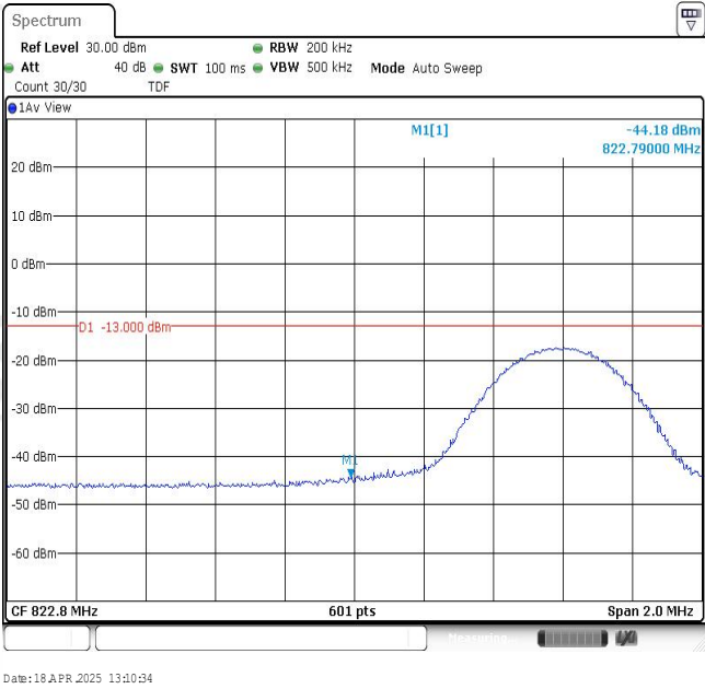
Band26-10MHz-QPSK-26828-1RB#49
