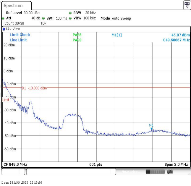
Band26-1.4MHz-QPSK-27033-1RB#0
