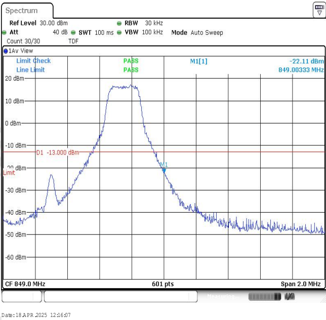
Band26-1.4MHz-16QAM-27033-1RB#5
