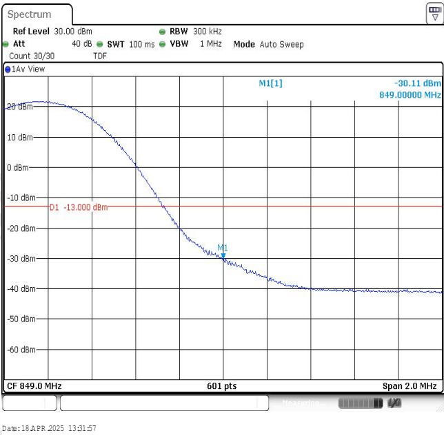
Band26-15MHz-QPSK-26965-1RB#74
