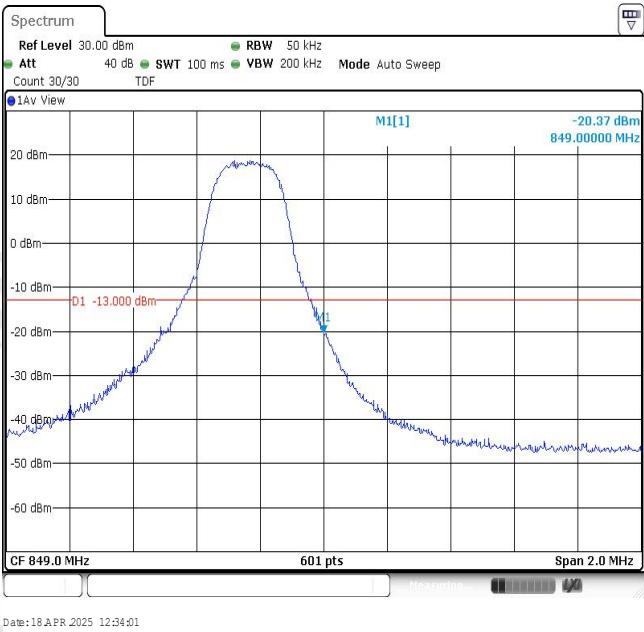
Band26-3MHz-QPSK-27025-1RB#14
