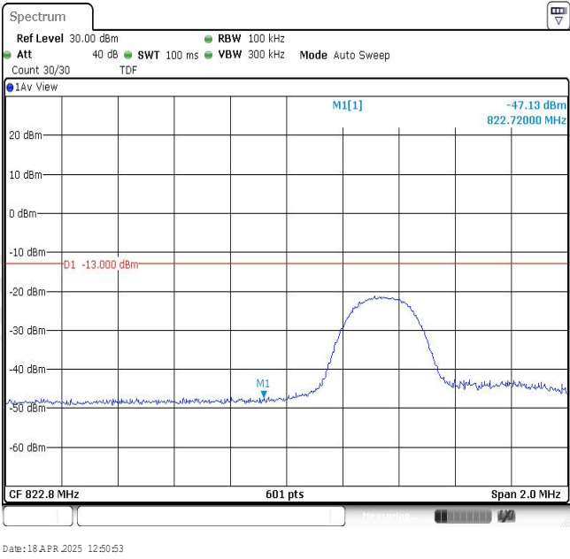
Band26-5MHz-QPSK-26803-1RB#24
