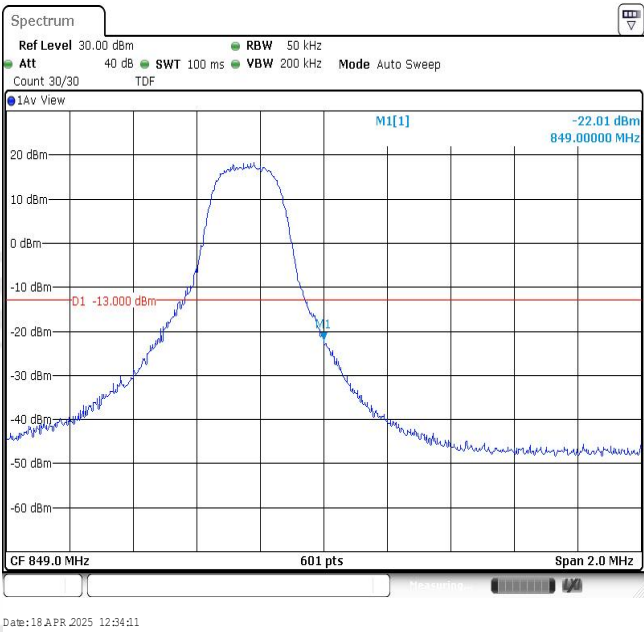
Band26-3MHz-16QAM-27025-1RB#14
