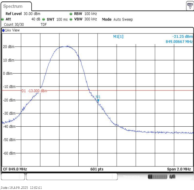
Band26-5MHz-QPSK-27015-1RB#24
