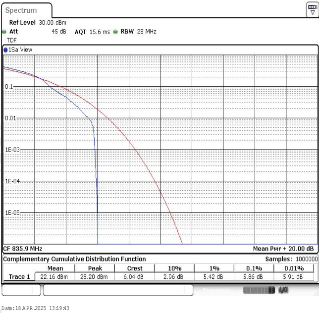
Band26-10MHz-16QAM-26909-1RB#0
