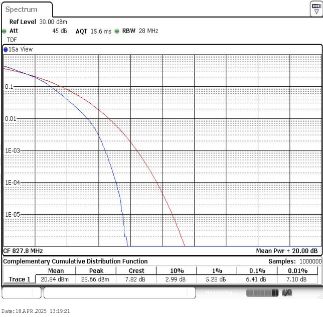
Band26-10MHz-16QAM-26828-50RB#0
