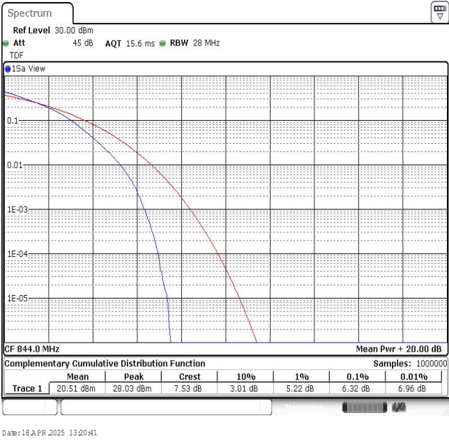
Band26-10MHz-16QAM-26990-50RB#0
