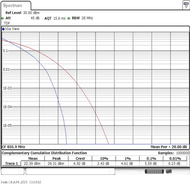
Band26-10MHz-QPSK-26909-50RB#0
