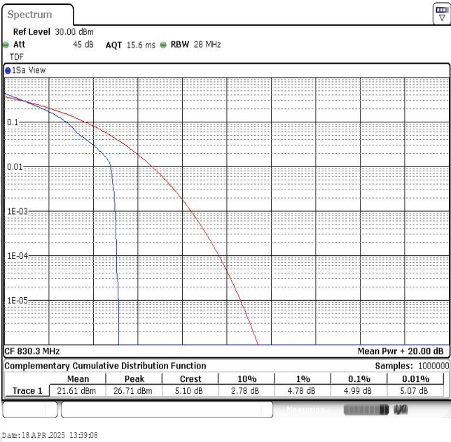
Band26-15MHz-QPSK-26853-1RB#0
