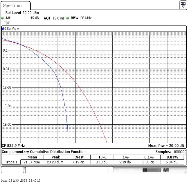
Band26-15MHz-16QAM-26909-75RB#0
