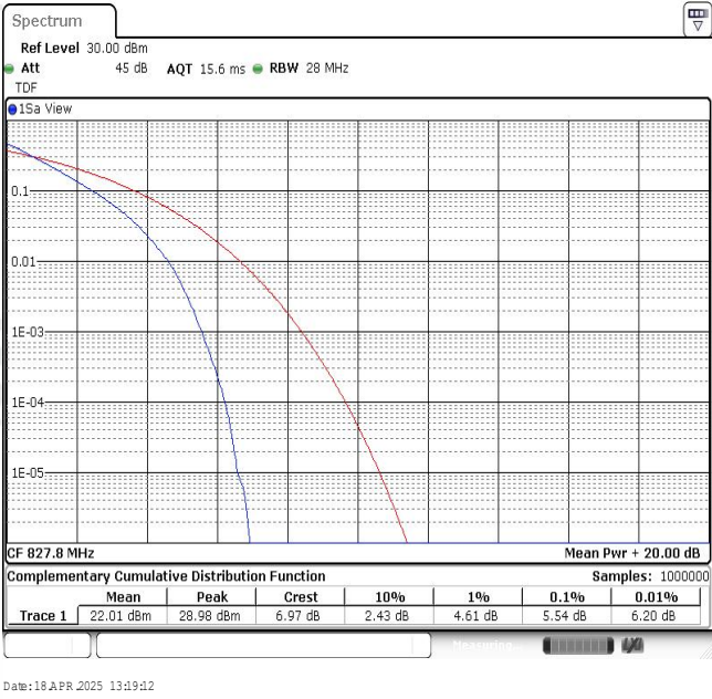
Band26-10MHz-QPSK-26828-50RB#0
