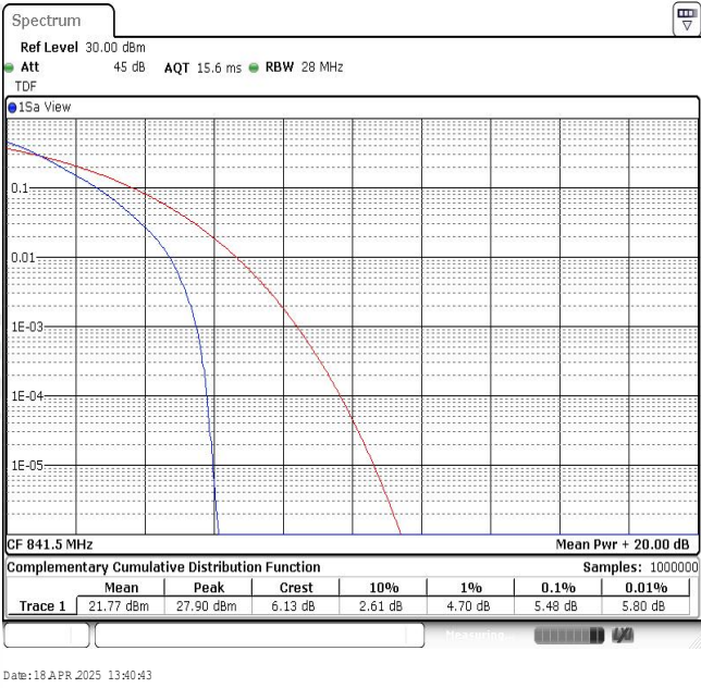
Band26-15MHz-QPSK-26965-75RB#0
