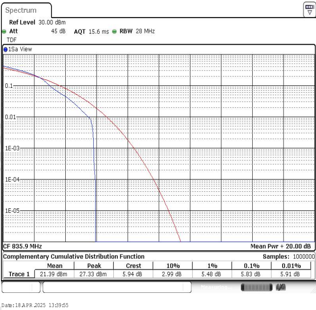
Band26-15MHz-16QAM-26909-1RB#0
