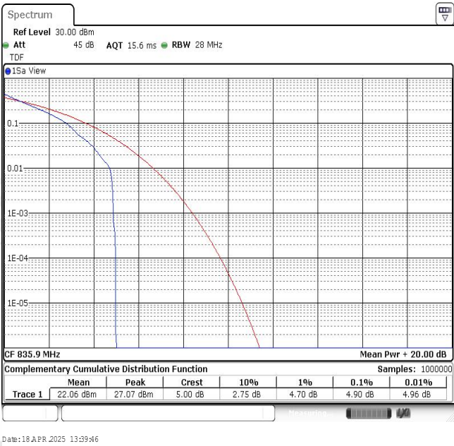
Band26-15MHz-QPSK-26909-1RB#0
