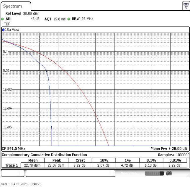
Band26-15MHz-QPSK-26965-1RB#0
