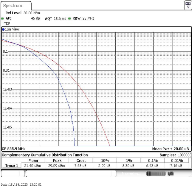
Band26-10MHz-16QAM-26909-50RB#0
