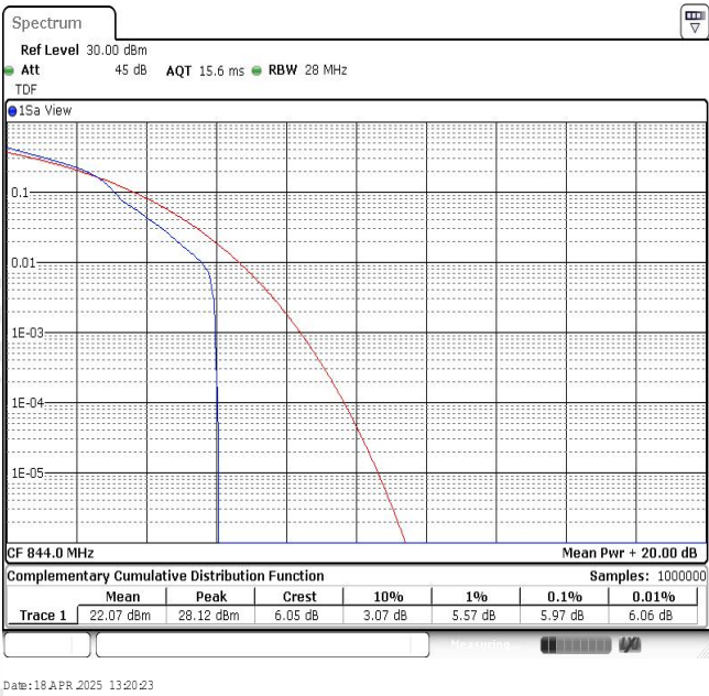
Band26-10MHz-16QAM-26990-1RB#0
