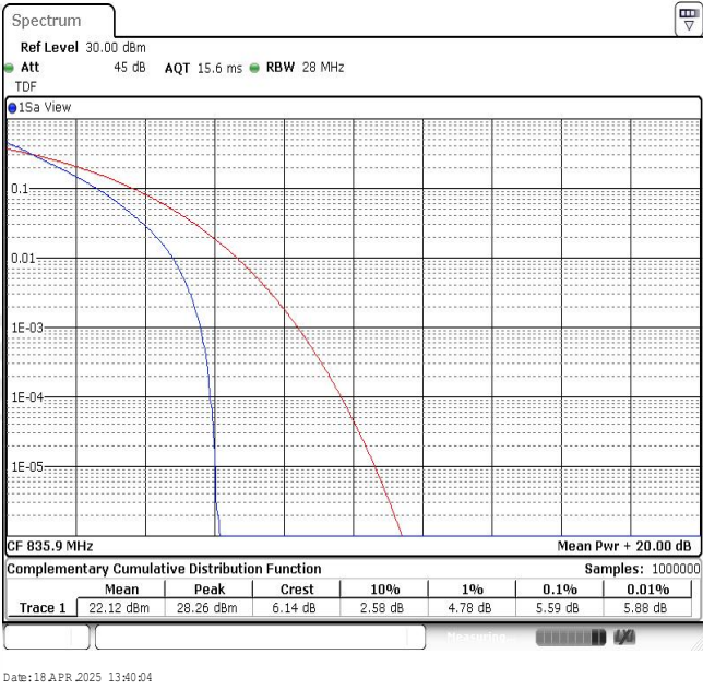
Band26-15MHz-QPSK-26909-75RB#0
