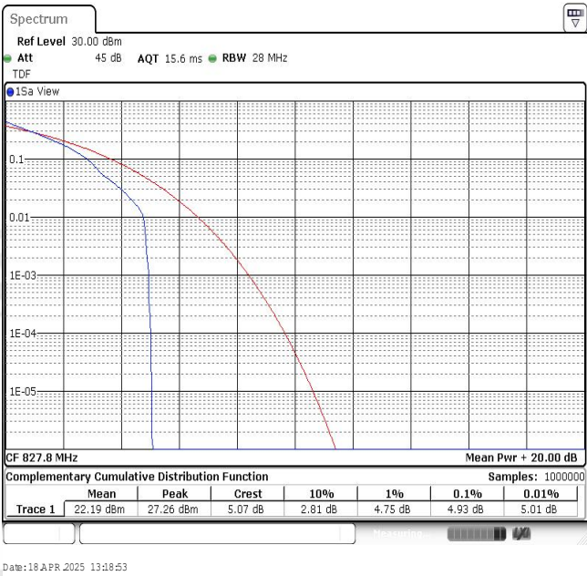
Band26-10MHz-QPSK-26828-1RB#0
