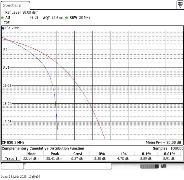
Band26-15MHz-QPSK-26853-75RB#0
