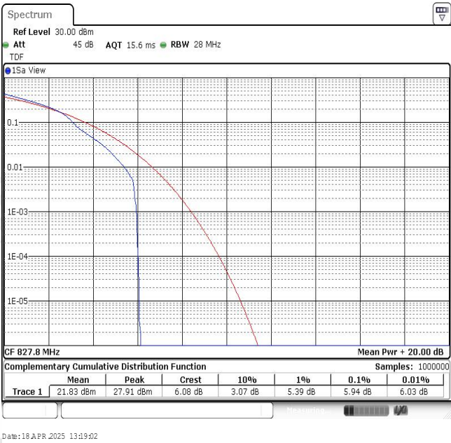
Band26-10MHz-16QAM-26828-1RB#0
