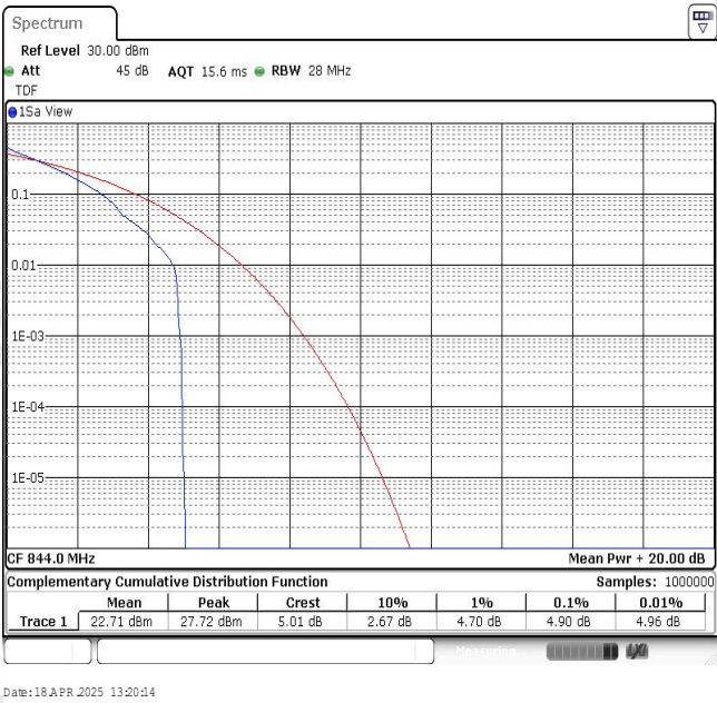
Band26-10MHz-QPSK-26990-1RB#0
