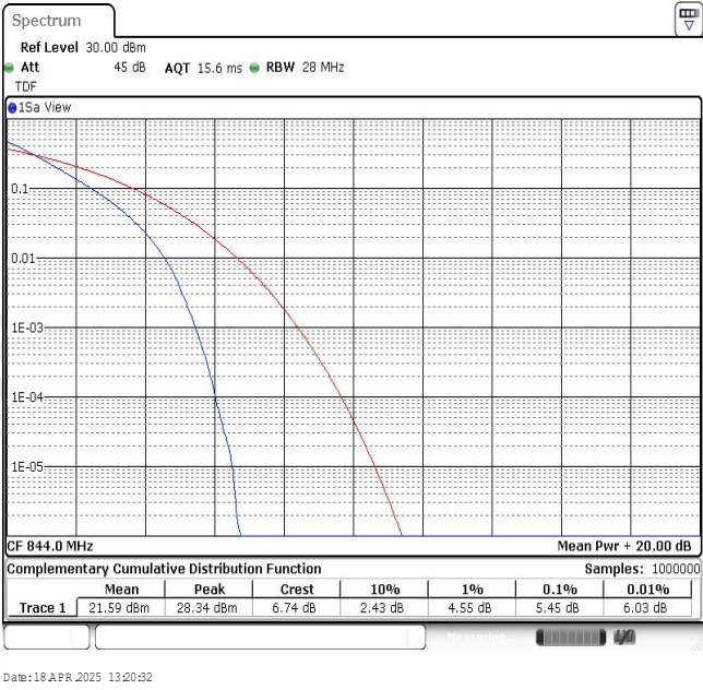
Band26-10MHz-QPSK-26990-50RB#0
