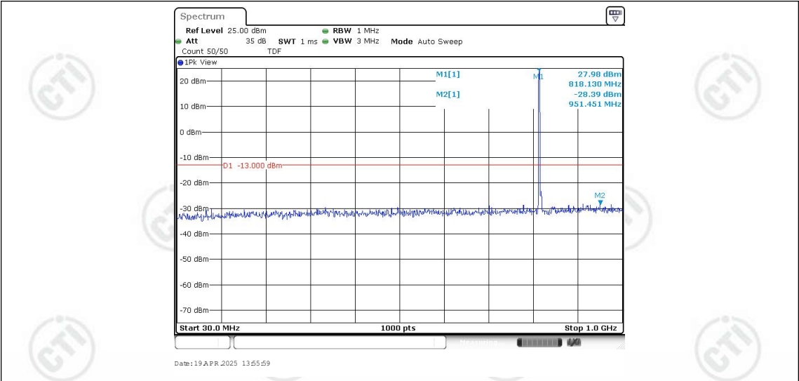
Band26-3MHz-16QAM-26740-1RB#0-Range1:30~1000MHz
