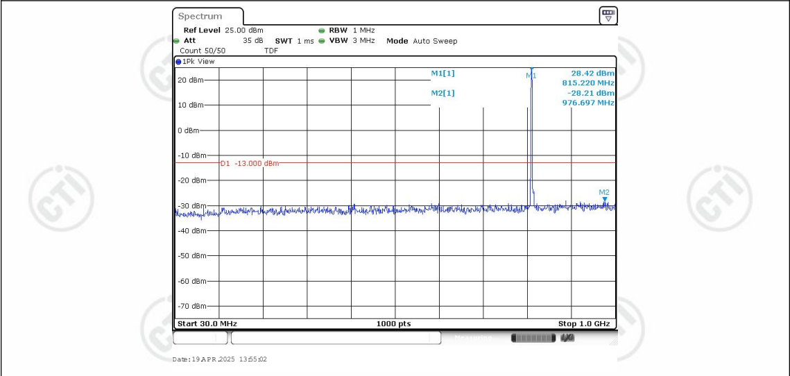
Band26-3MHz-QPSK-26705-1RB#0-Range1:30~1000MHz
