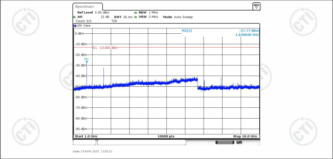
Band26-3MHz-QPSK-26705-1RB#0-Range2:1000~10000MHz
