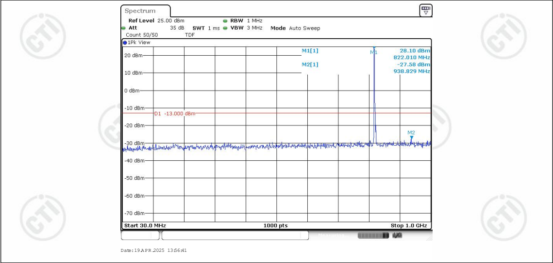
Band26-3MHz-16QAM-26775-1RB#0-Range1:30~1000MHz
