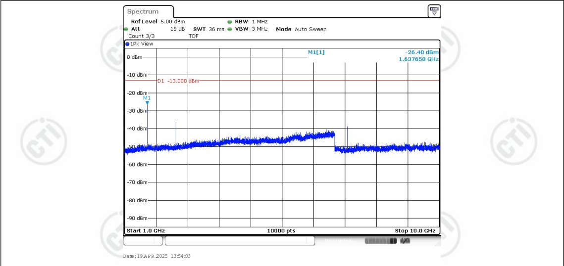
Band26-1.4MHz-16QAM-26740-1RB#0-Range2:1000~10000MHz
