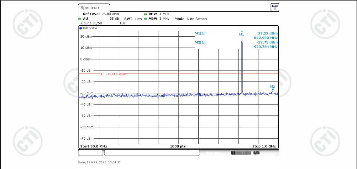
Band26-1.4MHz-16QAM-26783-1RB#0-Range1:30~1000MHz
