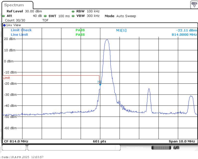
Band26-5MHz-16QAM-26715-1RB#0
