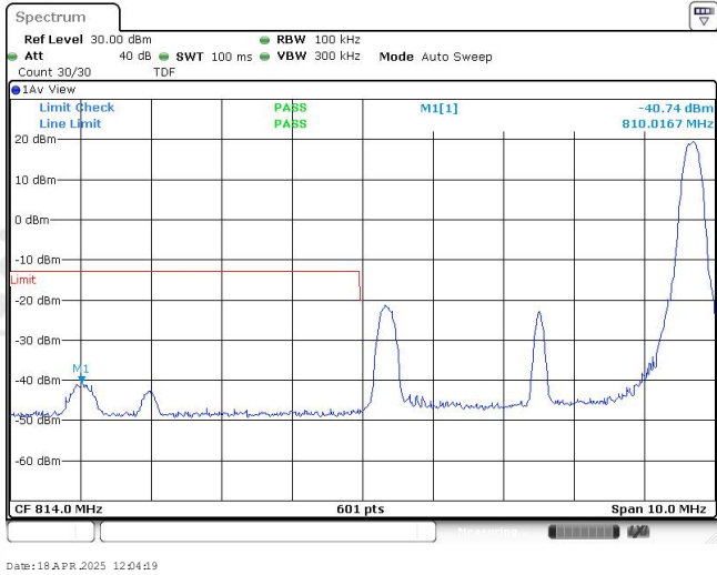
Band26-5MHz-16QAM-26715-1RB#24
