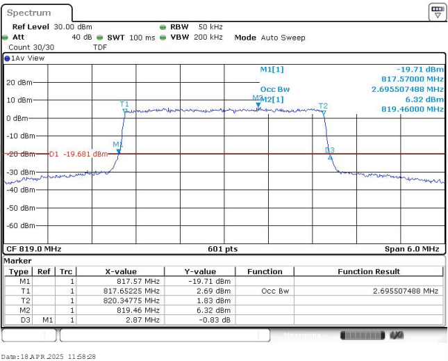
Band26-3MHz-QPSK-26740-15RB#0-2.696
