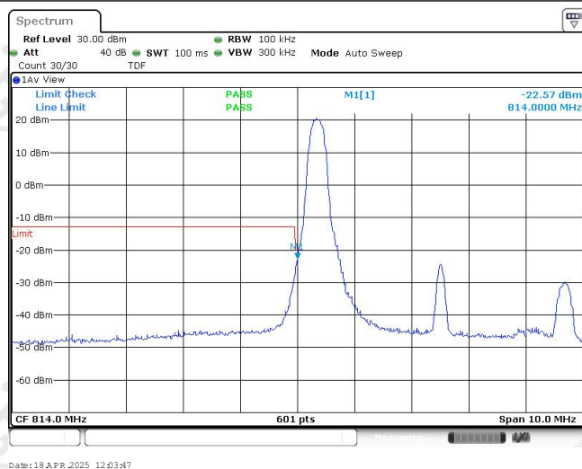
Band26-5MHz-QPSK-26715-1RB#0
