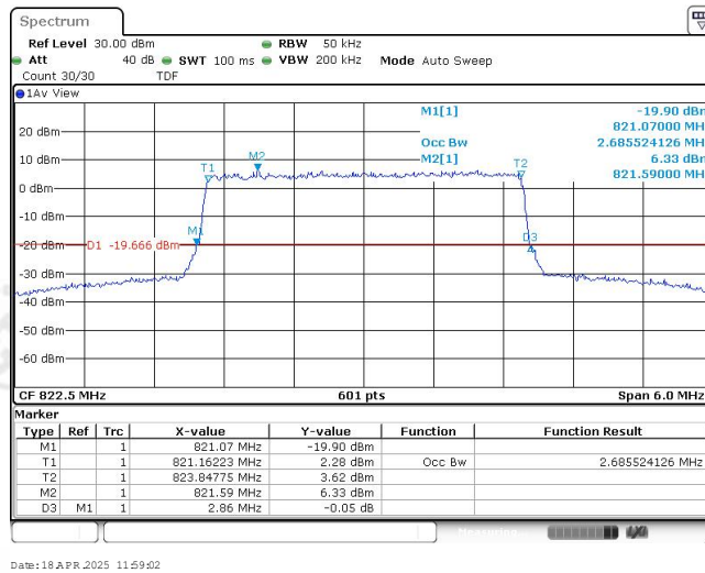
Band26-3MHz-16QAM-26775-15RB#0-2.686
