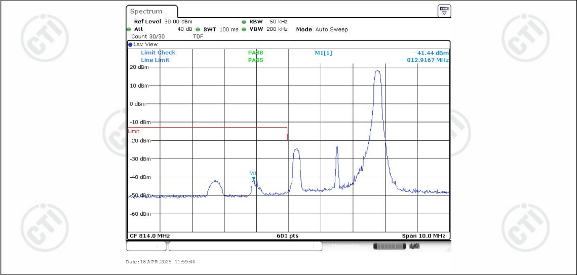
Band26-3MHz-QPSK-26705-1RB#14
