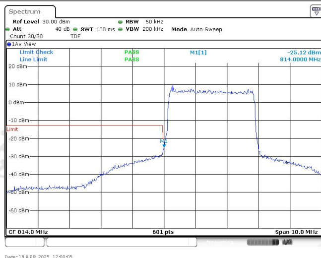
Band26-3MHz-QPSK-26705-15RB#0
