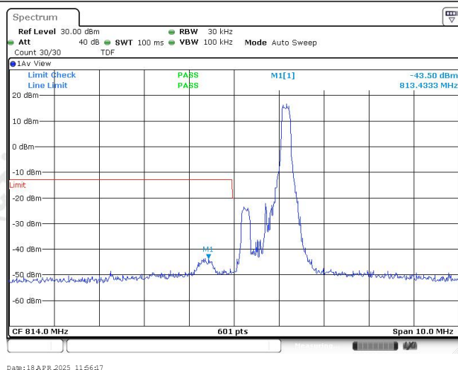
Band26-1.4MHz-16QAM-26697-1RB#5
