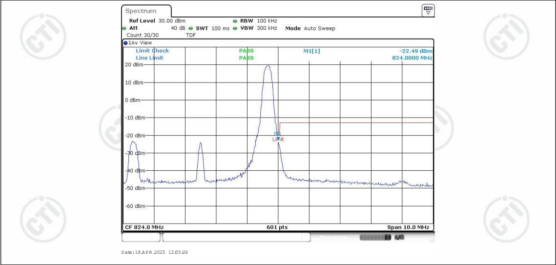
Band26-5MHz-16QAM-26765-1RB#24
