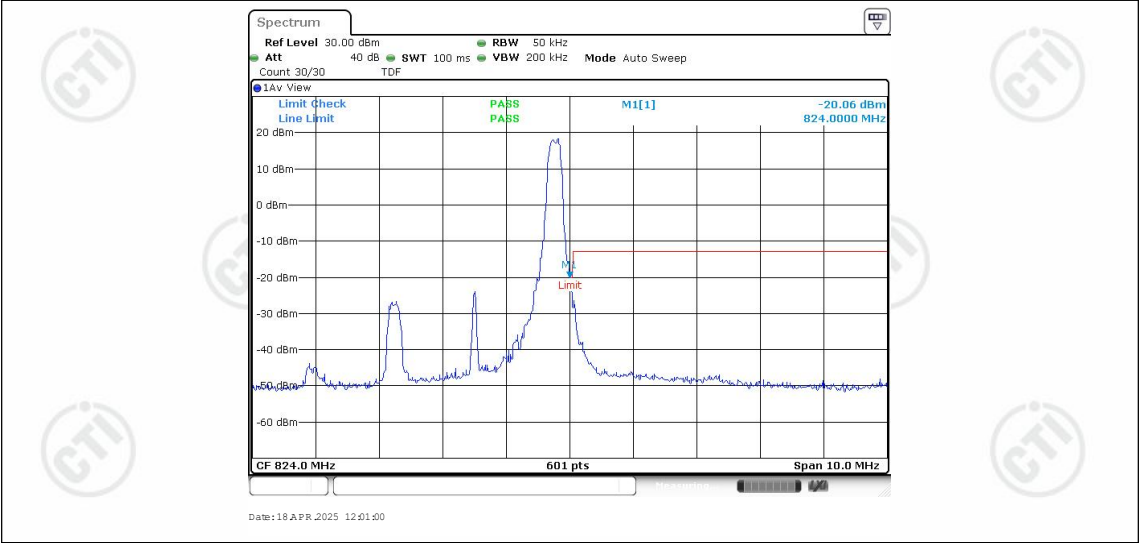
Band26-3MHz-16QAM-26775-1RB#14
