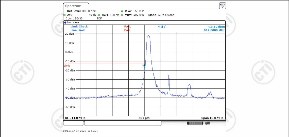
Band26-3MHz-QPSK-26705-1RB#0
