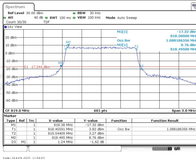
Band26-1.4MHz-16QAM-26740-6RB#0-1.088
