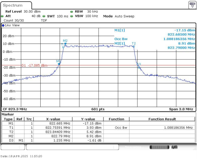
Band26-1.4MHz-16QAM-26783-6RB#0-1.088
