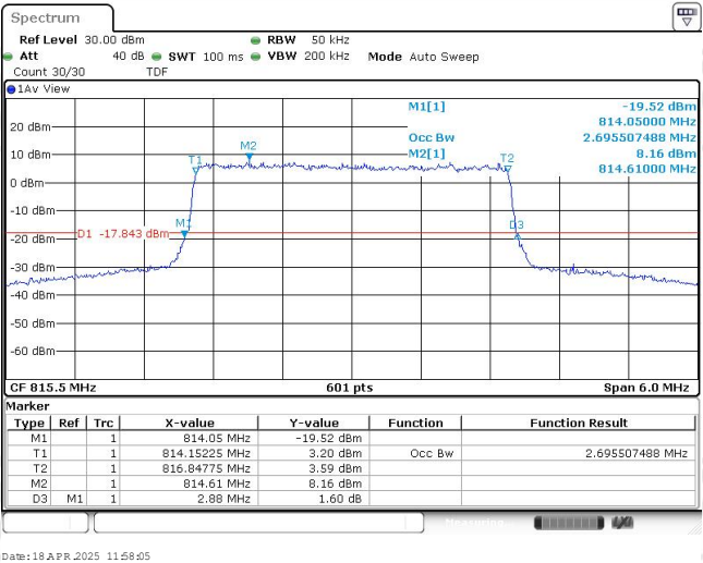
Band26-3MHz-QPSK-26705-15RB#0-2.696
