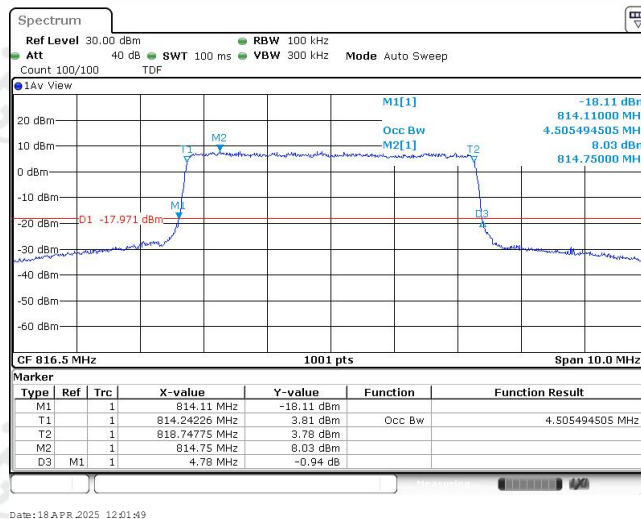
Band26-5MHz-QPSK-26715-25RB#0-4.505
