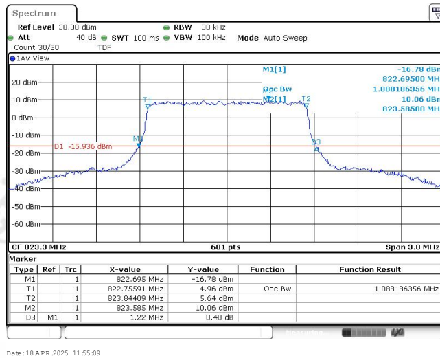
Band26-1.4MHz-QPSK-26783-6RB#0-1.088
