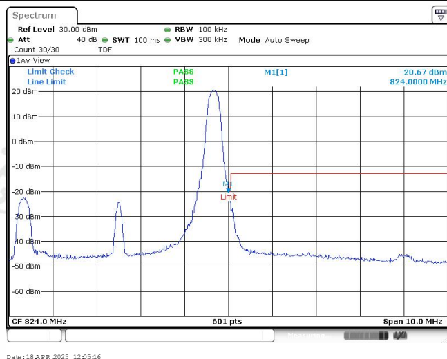
Band26-5MHz-QPSK-26765-1RB#24
