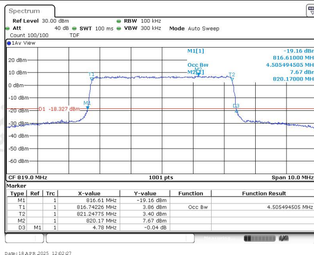
Band26-5MHz-QPSK-26740-25RB#0-4.505
