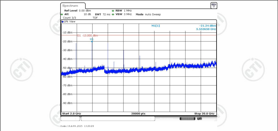
Band25-20MHz-QPSK-26140-1RB#0-Range3:2000~20000MHz
