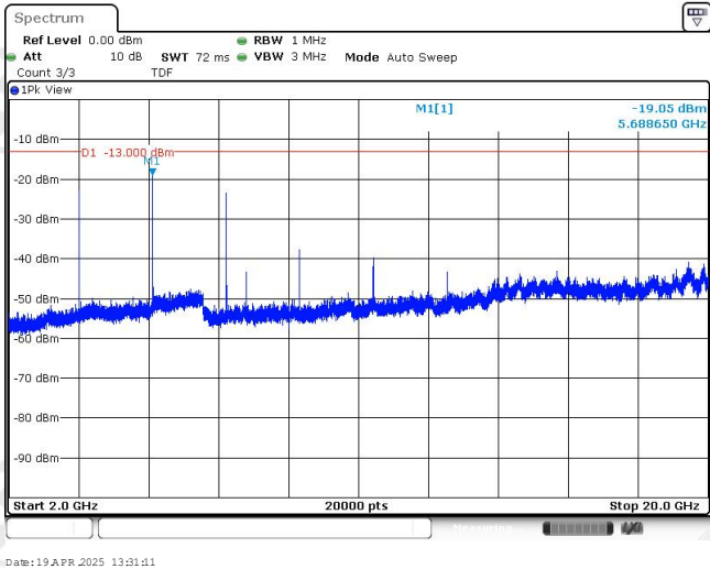
Band25-20MHz-QPSK-26590-1RB#0-Range3:2000~20000MHz
