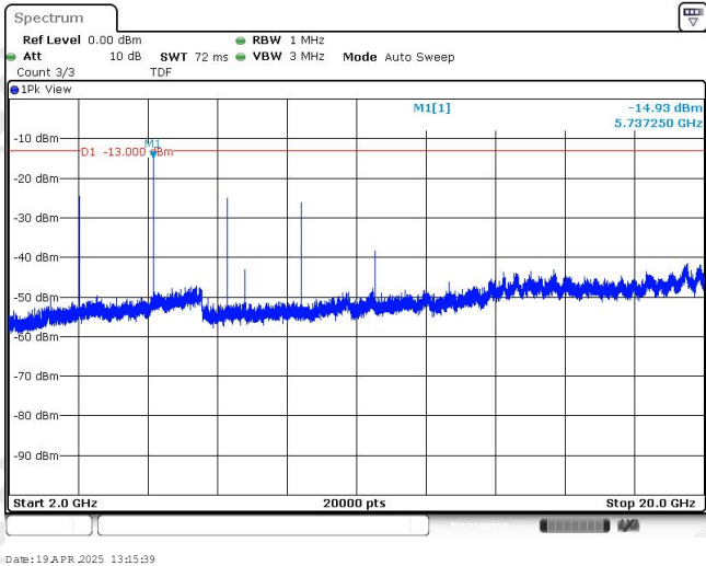
Band25-3MHz-QPSK-26675-1RB#0-Range3:2000~20000MHz
