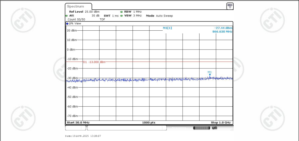
Band25-5MHz-16QAM-26365-1RB#0-Range1:30~1000MHz
