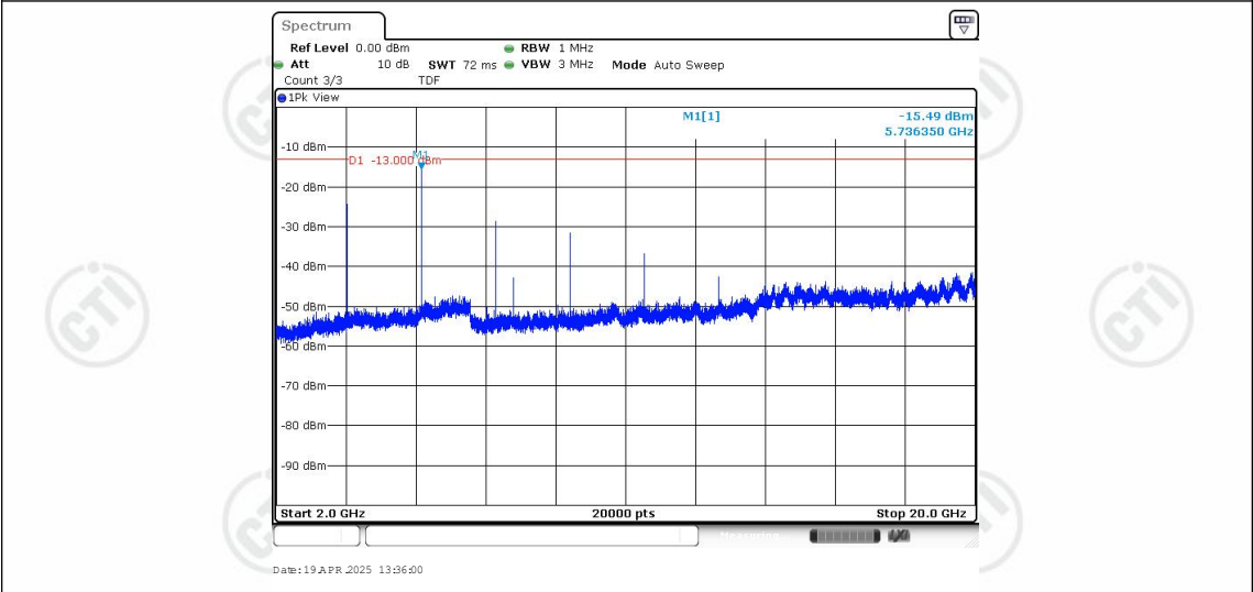
Band25-3MHz-16QAM-26675-1RB#0-Range3:2000~20000MHz
