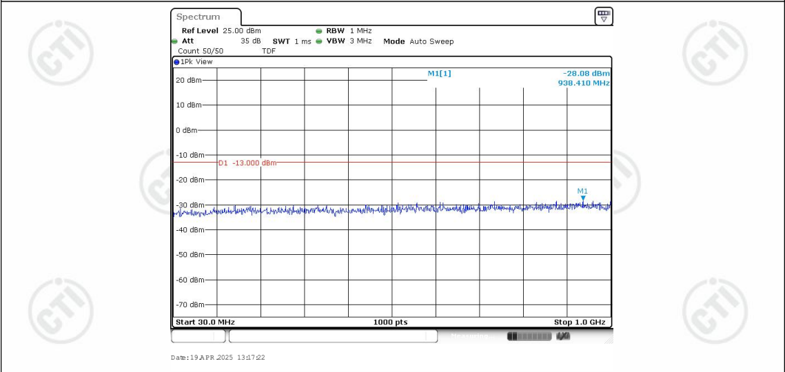
Band25-5MHz-QPSK-26065-1RB#0-Range1:30~1000MHz
