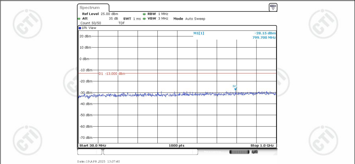
Band25-5MHz-16QAM-26065-1RB#0-Range1:30~1000MHz
