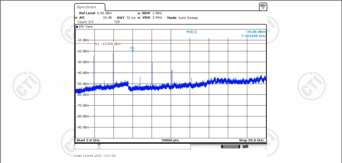
Band25-5MHz-QPSK-26065-1RB#0-Range3:2000~20000MHz
