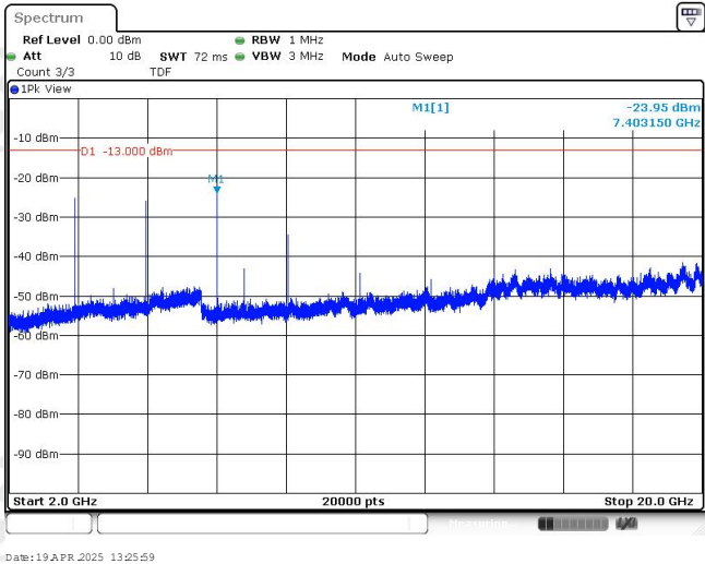
Band25-15MHz-QPSK-26115-1RB#0-Range3:2000~20000MHz
