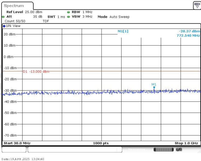
Band25-3MHz-16QAM-26055-1RB#0-Range1:30~1000MHz
