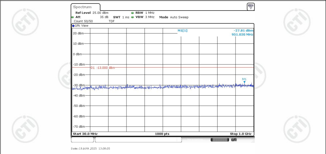
Band25-5MHz-16QAM-26665-1RB#0-Range1:30~1000MHz
