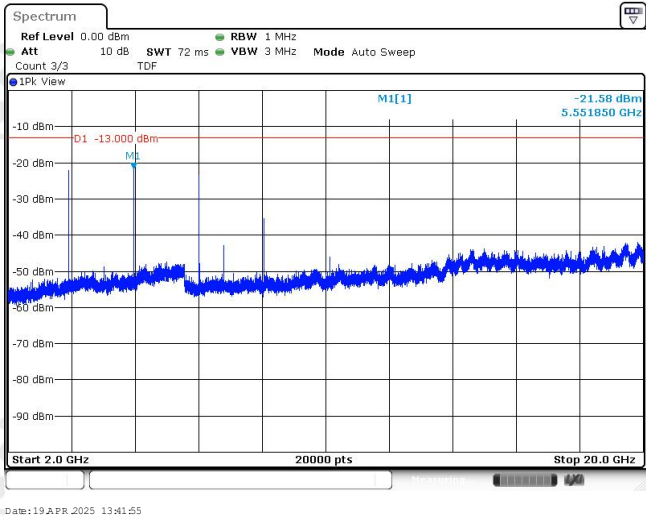
Band25-10MHz-16QAM-26090-1RB#0-Range3:2000~20000MHz
