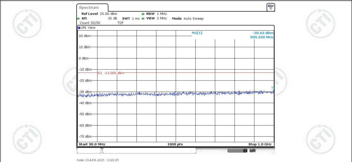
Band25-10MHz-QPSK-26640-1RB#0-Range1:30~1000MHz
