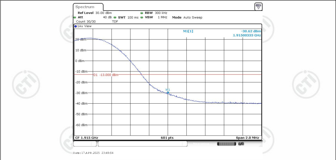
Band25-15MHz-16QAM-26615-1RB#74
