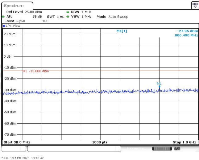
Band25-1.4MHz-QPSK-26365-1RB#0-Range1:30~1000MHz
