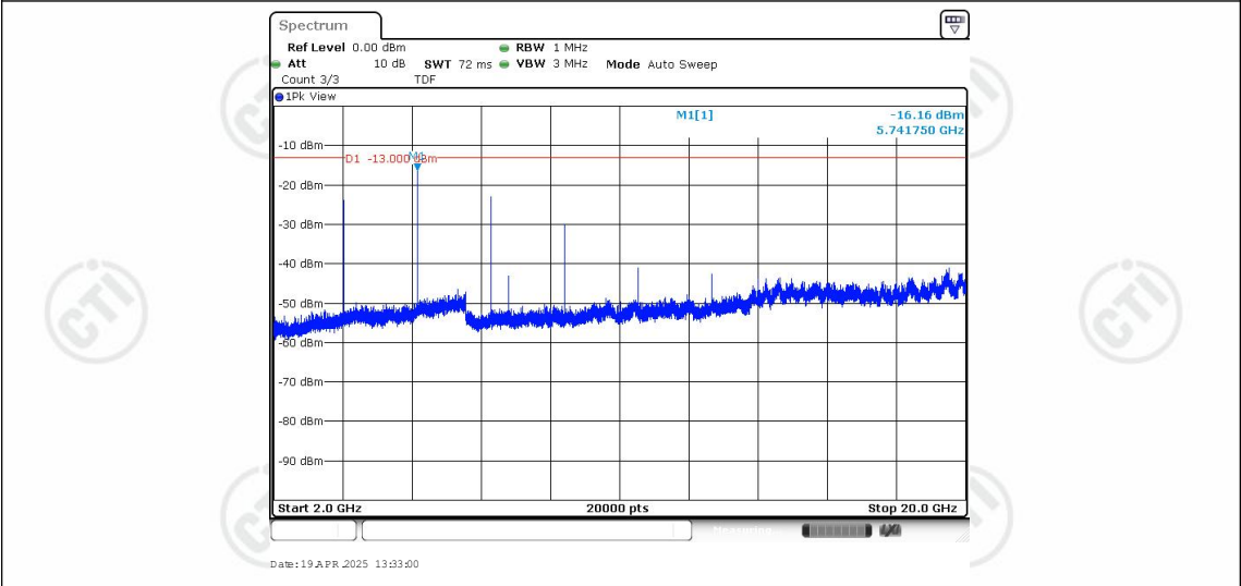
Band25-1.4MHz-16QAM-26683-1RB#0-Range3:2000~20000MHz
