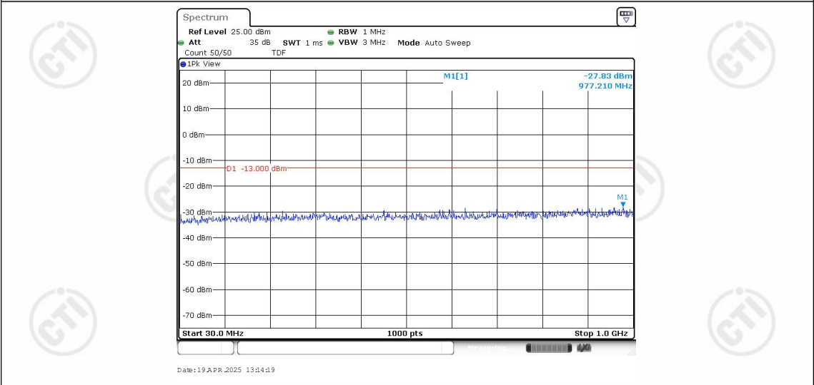
Band25-3MHz-QPSK-26055-1RB#0-Range1:30~1000MHz
