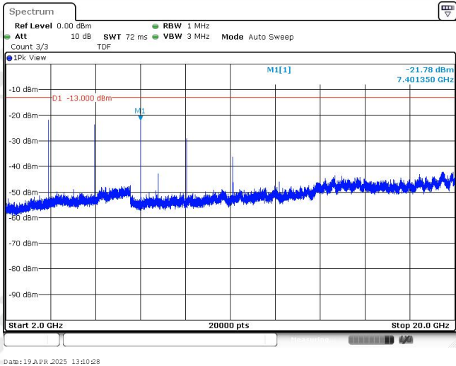
Band25-1.4MHz-QPSK-26047-1RB#0-Range3:2000~20000MHz
