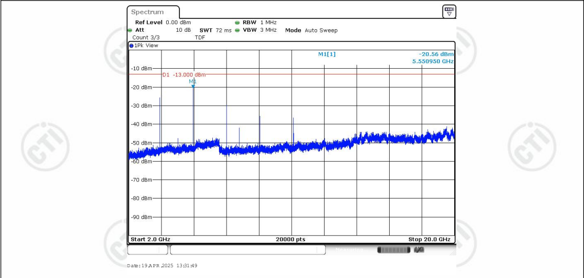
Band25-1.4MHz-16QAM-26047-1RB#0-Range3:2000~20000MHz
