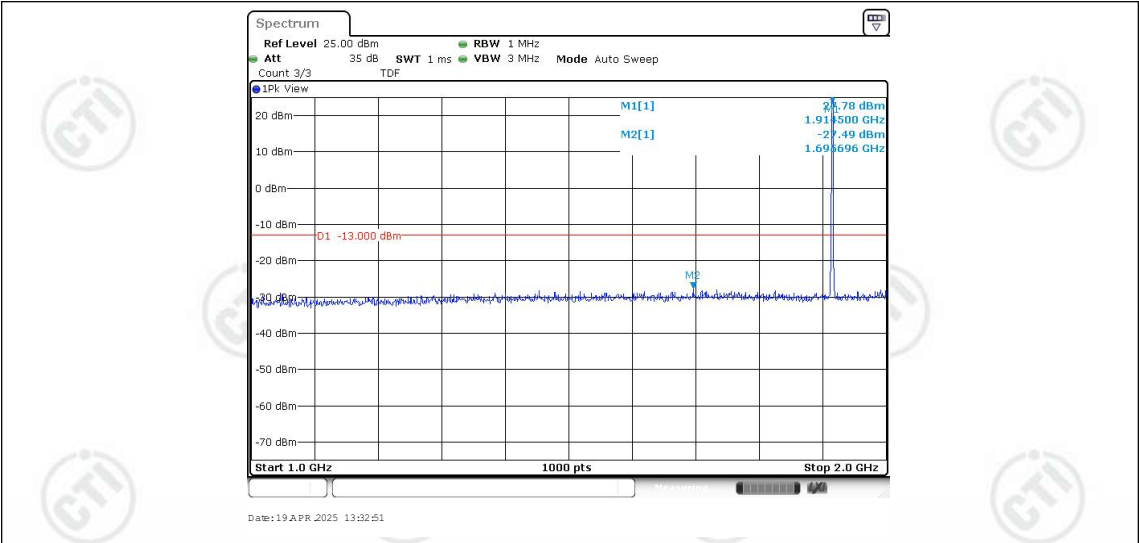
Band25-1.4MHz-16QAM-26683-1RB#0-Range2:1000~2000MHz
