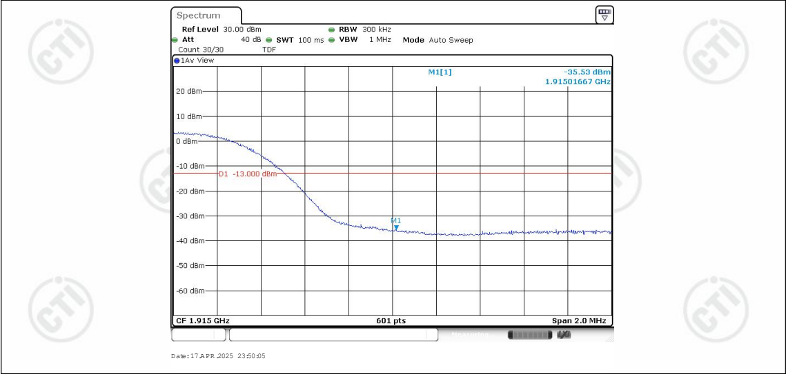
Band25-15MHz-16QAM-26615-75RB#0
