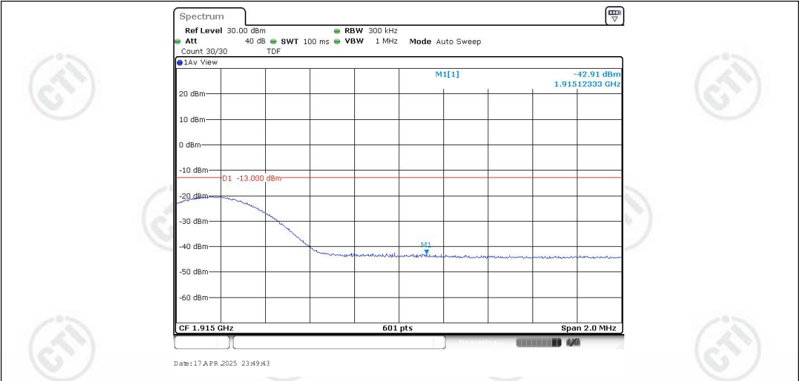
Band25-15MHz-16QAM-26615-1RB#0
