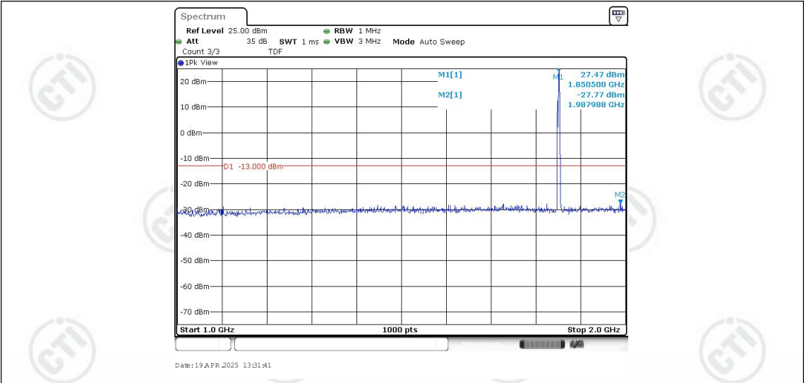
Band25-1.4MHz-16QAM-26047-1RB#0-Range2:1000~2000MHz
