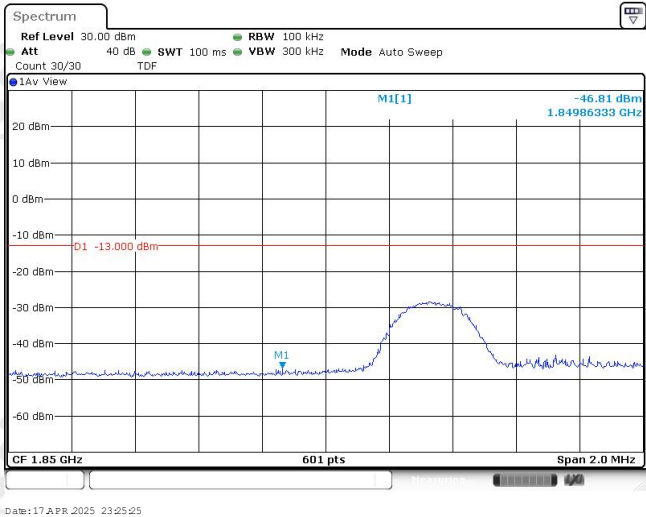
Band25-5MHz-16QAM-26065-1RB#24
