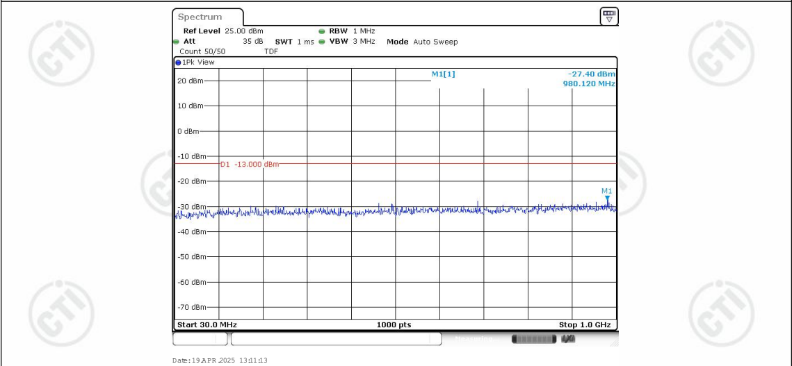
Band25-1.4MHz-QPSK-26683-1RB#0-Range1:30~1000MHz
