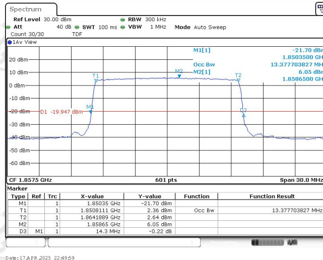
Band25-15MHz-QPSK-26115-75RB#0-13.378
