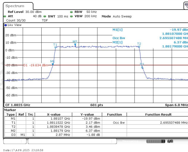
Band25-3MHz-16QAM-26365-15RB#0-2.696
