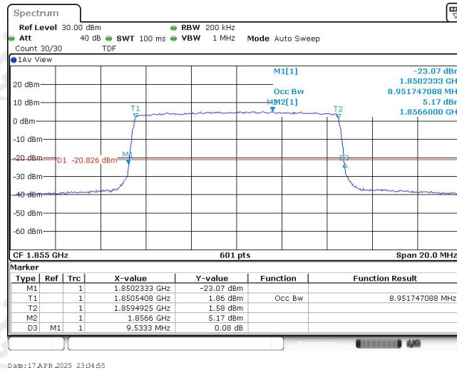
Band25-10MHz-16QAM-26090-50RB#0-8.952
