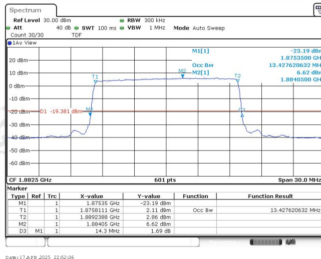
Band25-15MHz-QPSK-26365-75RB#0-13.428
