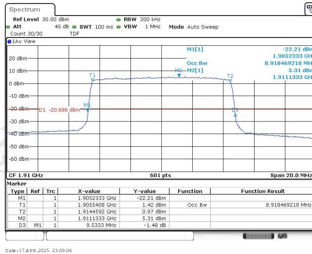
Band25-10MHz-16QAM-26640-50RB#0-8.918
