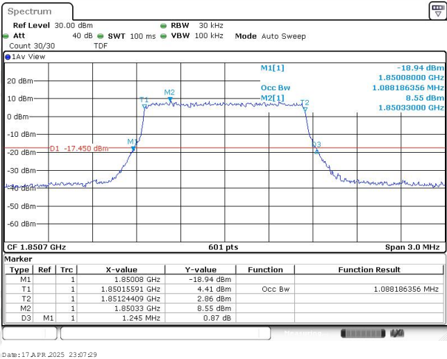
Band25-1.4MHz-16QAM-26047-6RB#0-1.088
