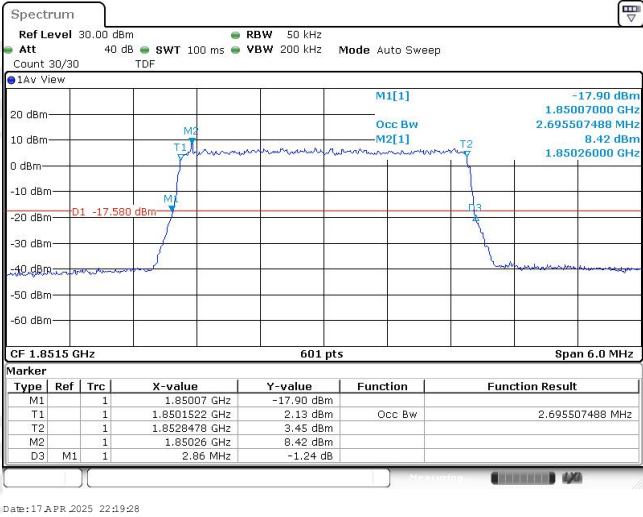
Band25-3MHz-QPSK-26055-15RB#0-2.696
