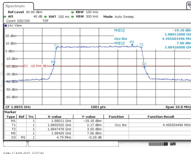
Band25-5MHz-16QAM-26365-25RB#0-4.496
