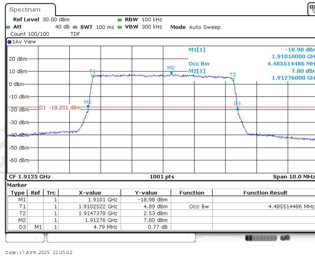
Band25-5MHz-QPSK-26665-25RB#0-4.486
