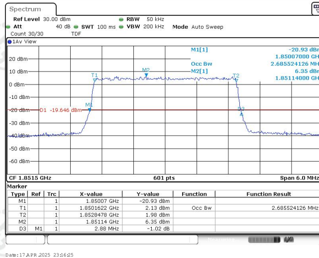
Band25-3MHz-16QAM-26055-15RB#0-2.686
