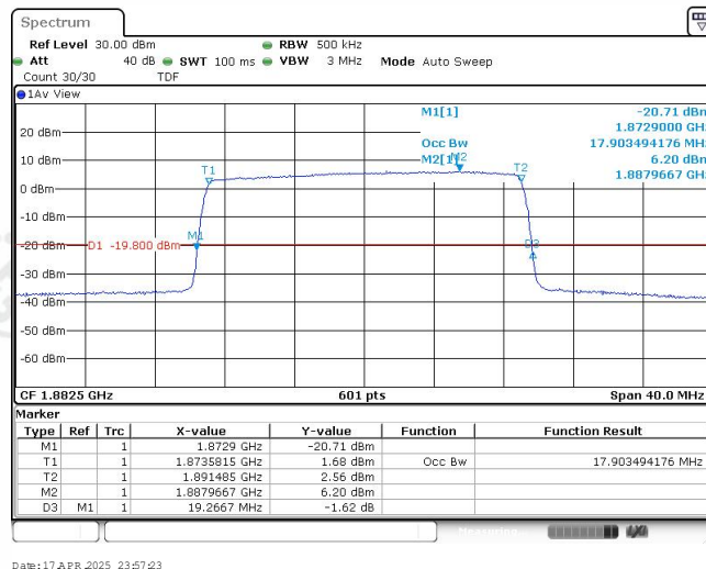
Band25-20MHz-16QAM-26365-100RB#0-17.903
