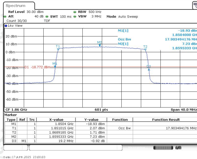
Band25-20MHz-QPSK-26140-100RB#0-17.903
