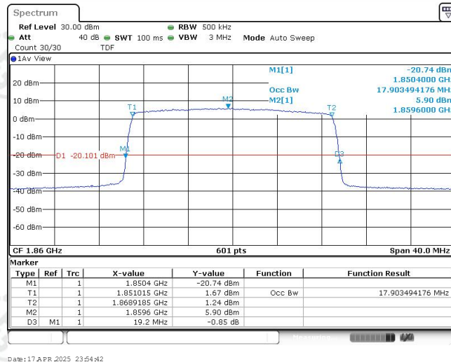
Band25-20MHz-16QAM-26140-100RB#0-17.903
