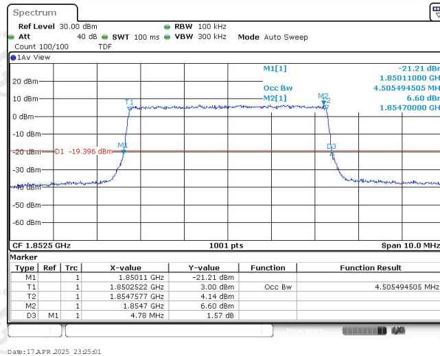
Band25-5MHz-16QAM-26065-25RB#0-4.505
