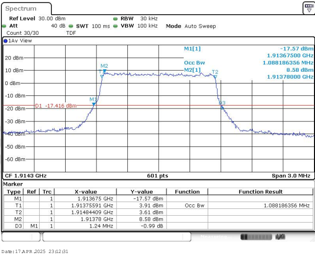
Band25-1.4MHz-16QAM-26683-6RB#0-1.088
