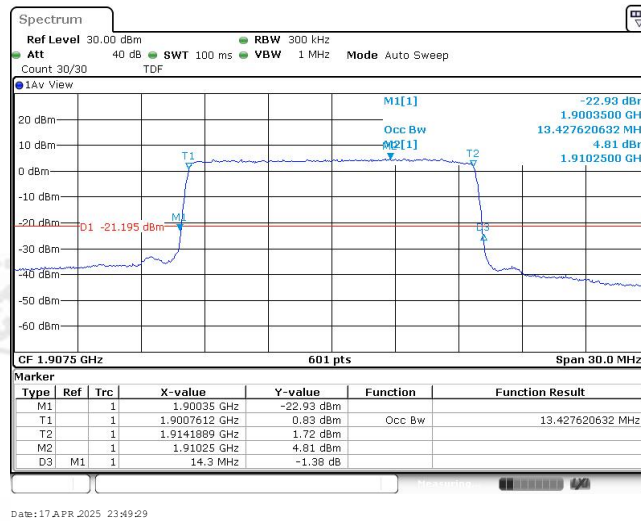
Band25-15MHz-16QAM-26615-75RB#0-13.428
