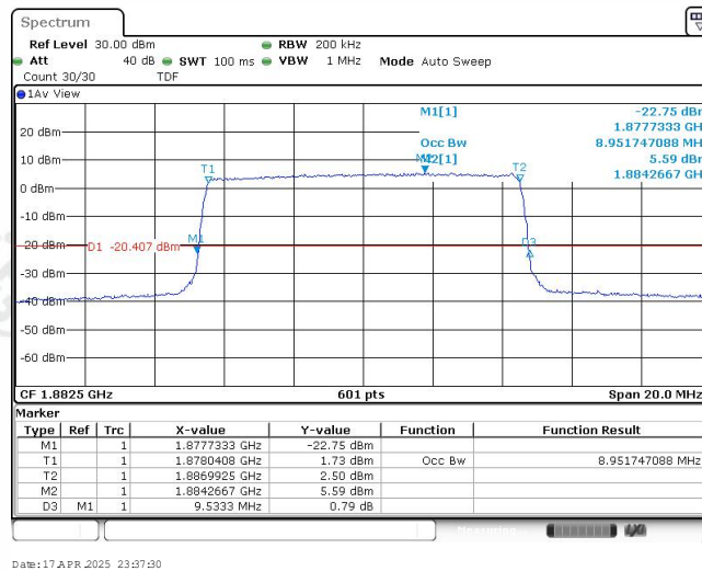
Band25-10MHz-16QAM-26365-50RB#0-8.952
